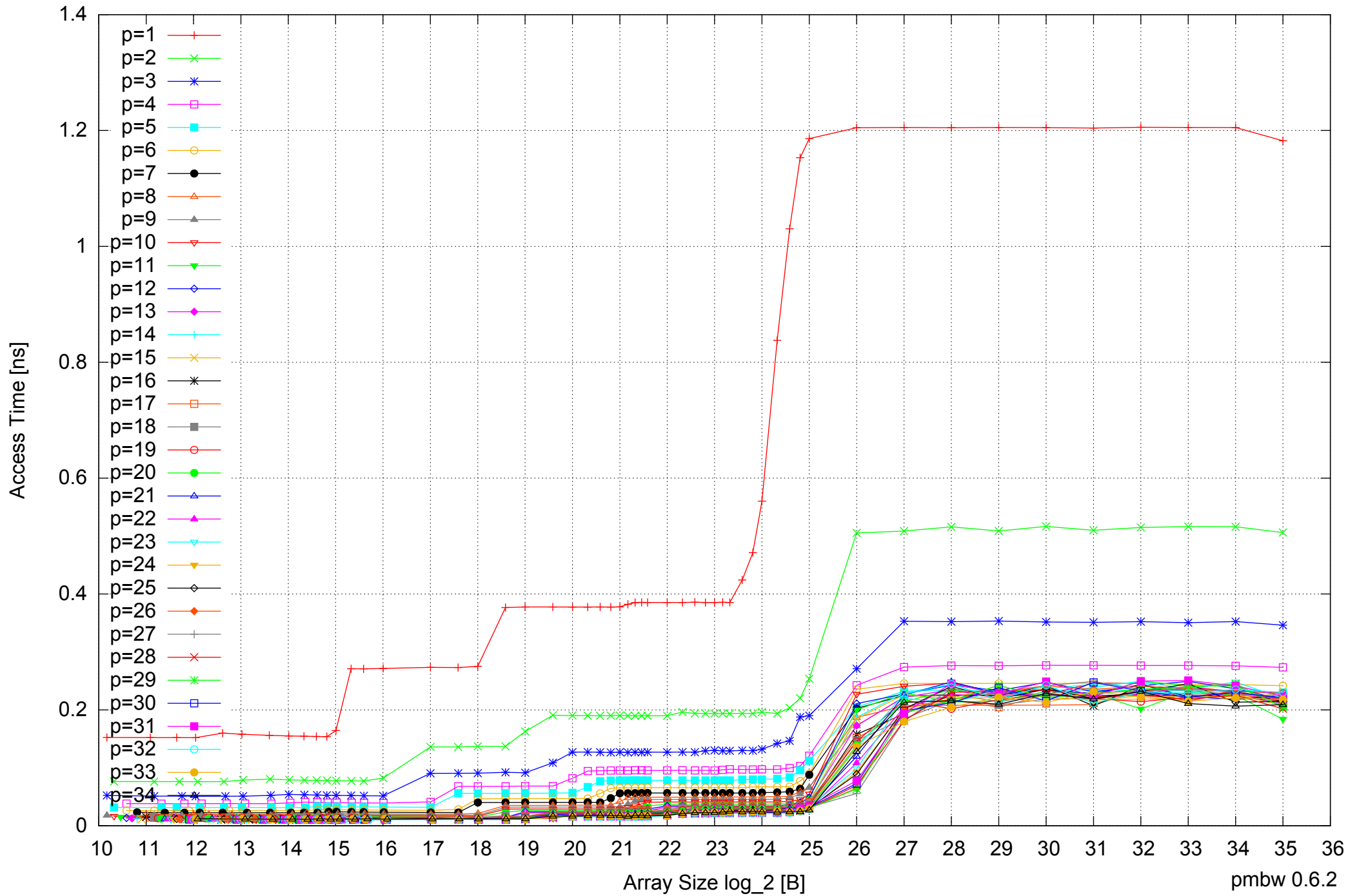
Intel Xeon E5-2670 64GB - Parallel Memory Access Time - ScanRead64PtrUnrollLoop
