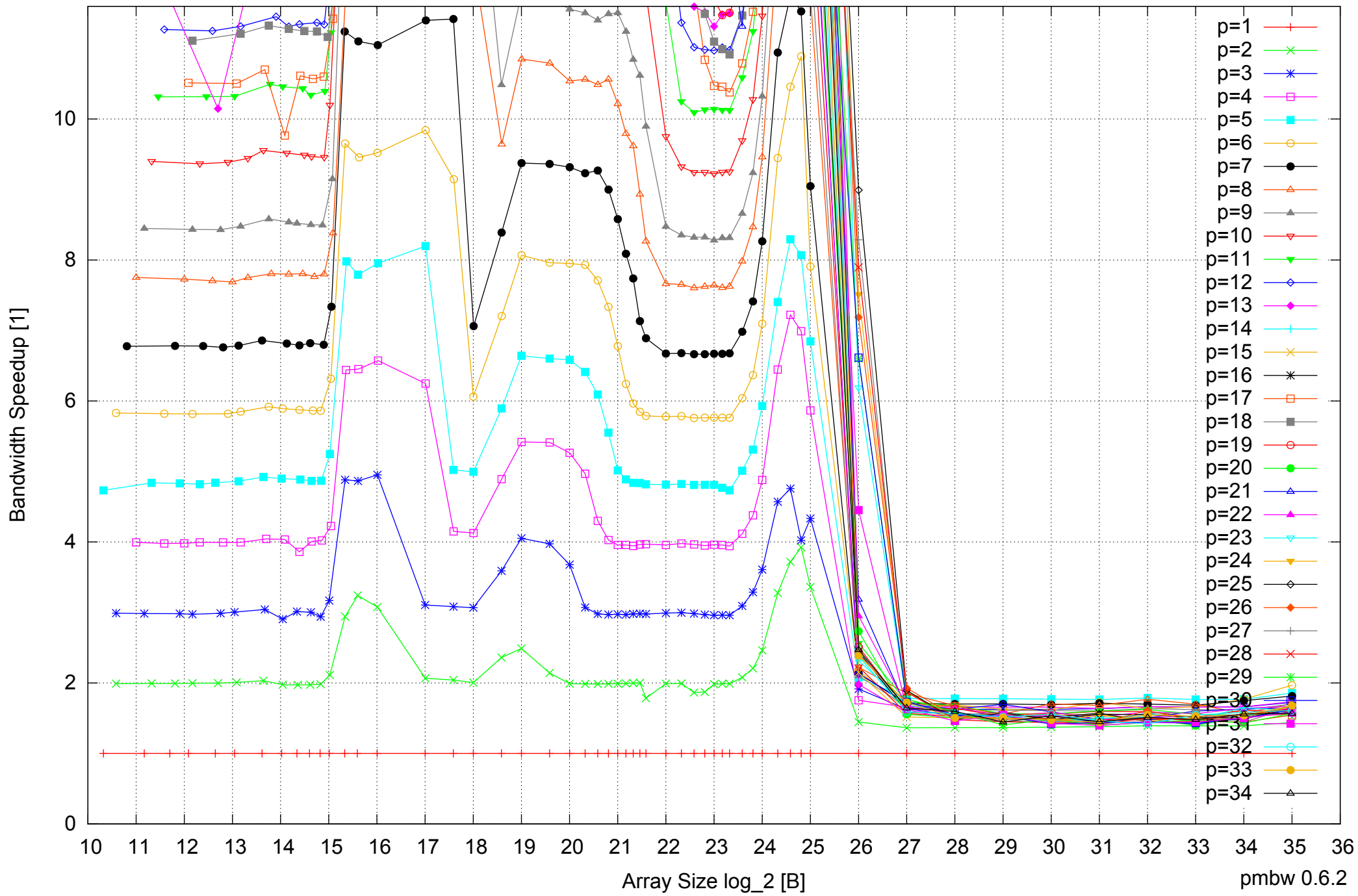
Intel Xeon E5-2670 64GB - Speedup of Parallel Memory Bandwidth (enlarged) - ScanWrite128PtrUnrollLoop
