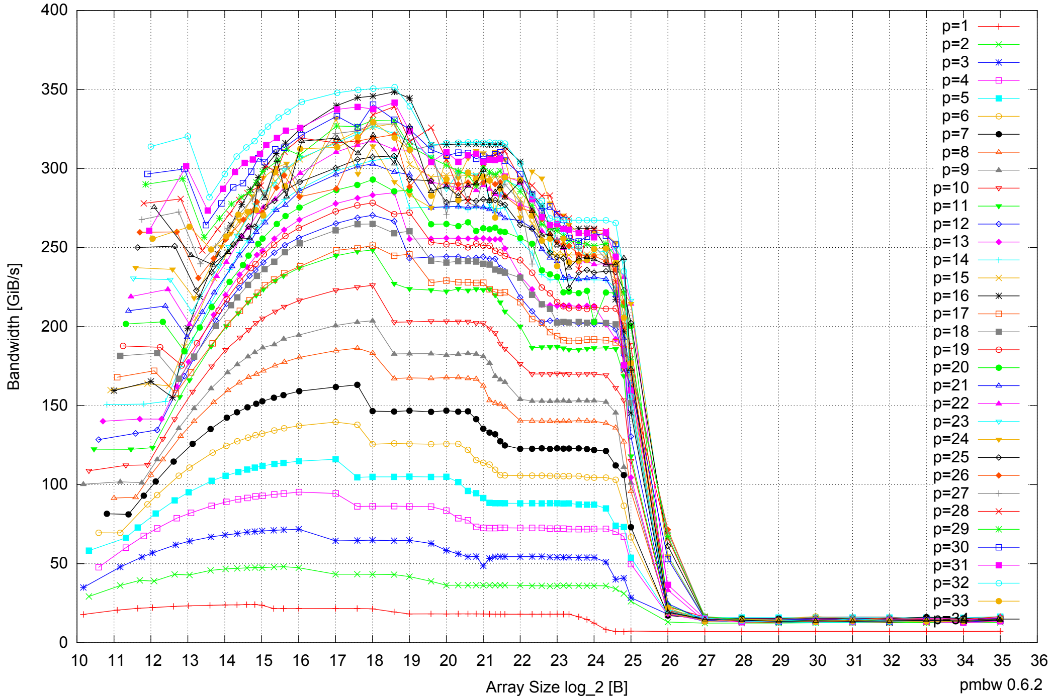
Intel Xeon E5-2670 64GB - Parallel Memory Bandwidth - ScanWrite64PtrSimpleLoop
