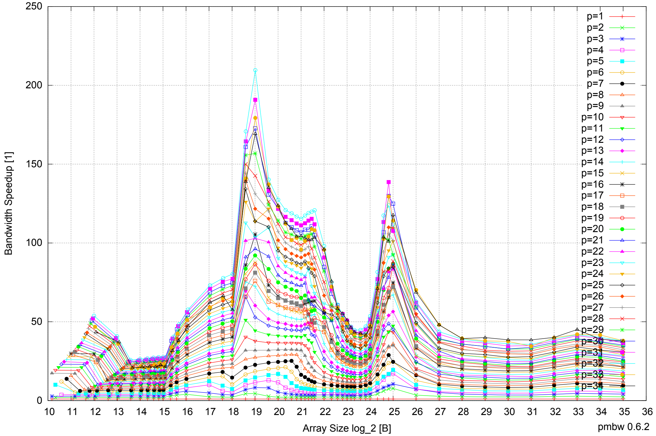
Intel Xeon E5-2670 64GB - Speedup of Parallel Memory Bandwidth - PermRead64SimpleLoop
