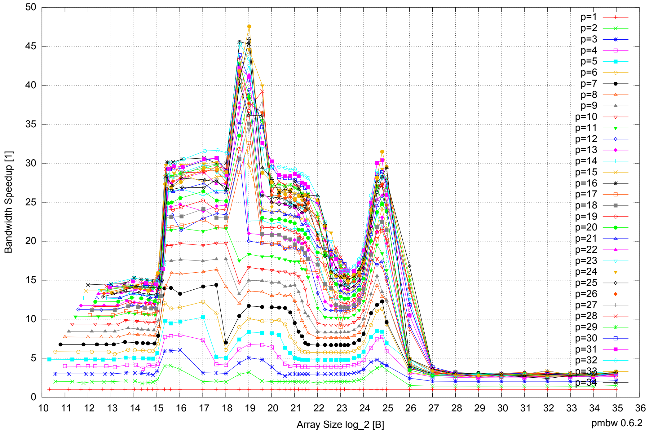
Intel Xeon E5-2670 64GB - Speedup of Parallel Memory Bandwidth - ScanRead128PtrUnrollLoop
