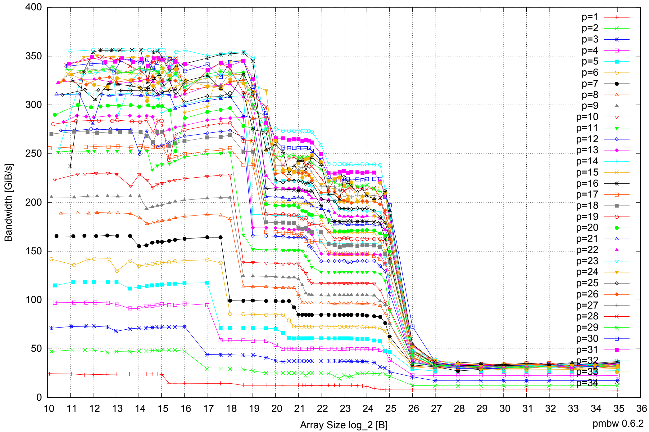
Intel Xeon E5-2670 64GB - Parallel Memory Bandwidth - ScanRead32PtrUnrollLoop
