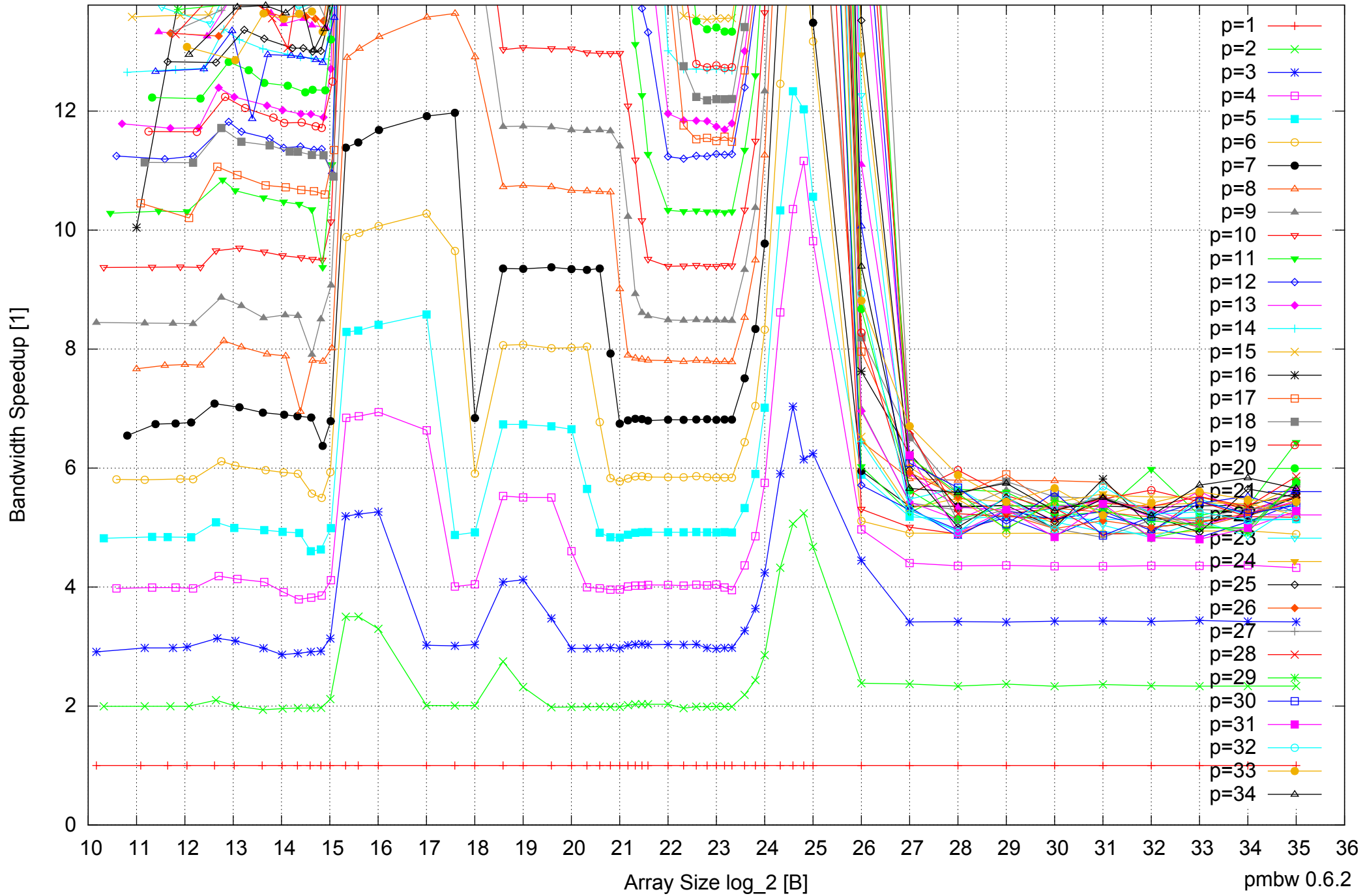
Intel Xeon E5-2670 64GB - Speedup of Parallel Memory Bandwidth (enlarged) - ScanRead64PtrUnrollLoop
