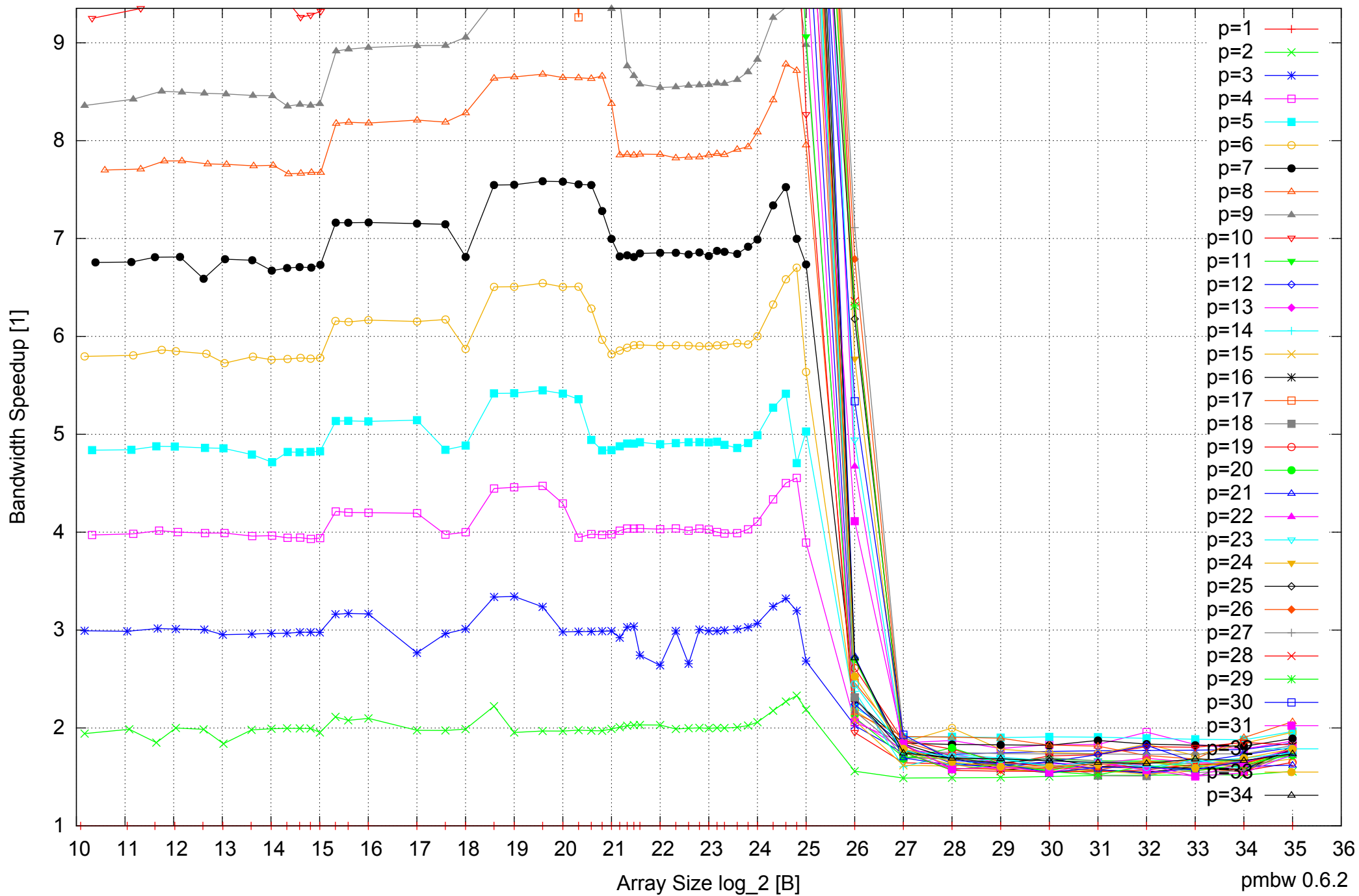
Intel Xeon E5-2670 64GB - Speedup of Parallel Memory Bandwidth (enlarged) - ScanWrite32PtrUnrollLoop
