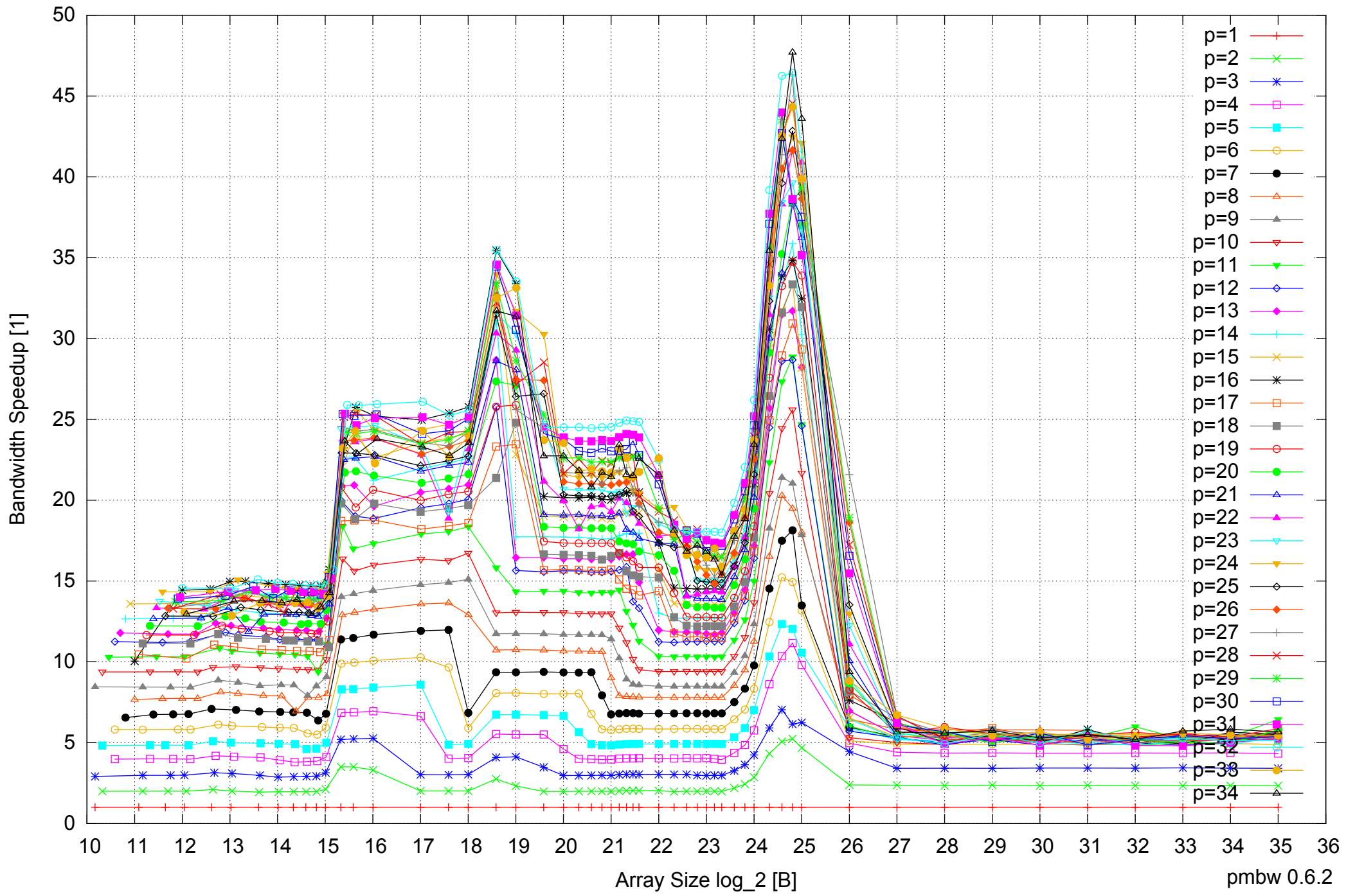
Intel Xeon E5-2670 64GB - Speedup of Parallel Memory Bandwidth - ScanRead64PtrUnrollLoop
