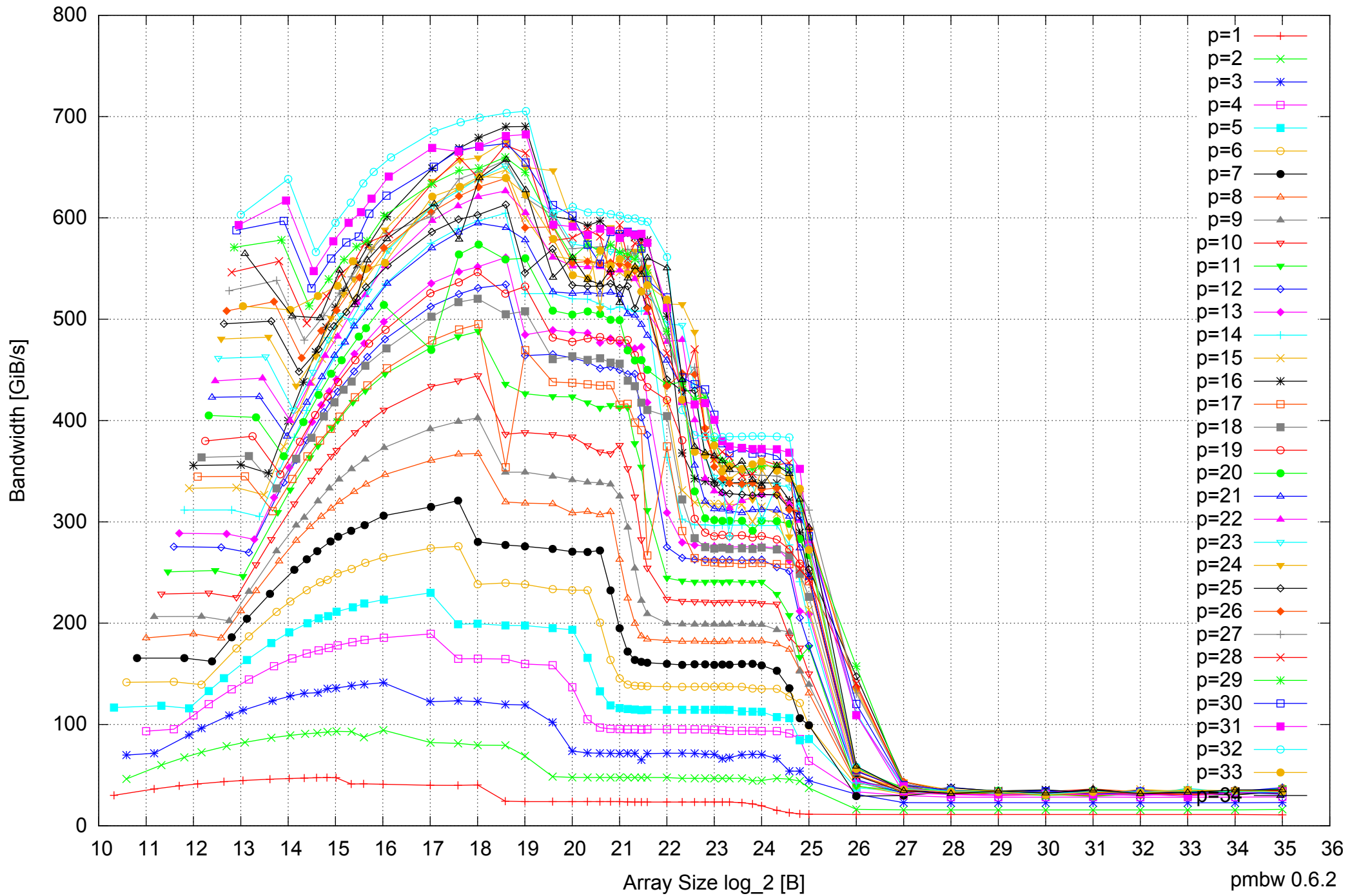
Intel Xeon E5-2670 64GB - Parallel Memory Bandwidth - ScanRead128PtrSimpleLoop
