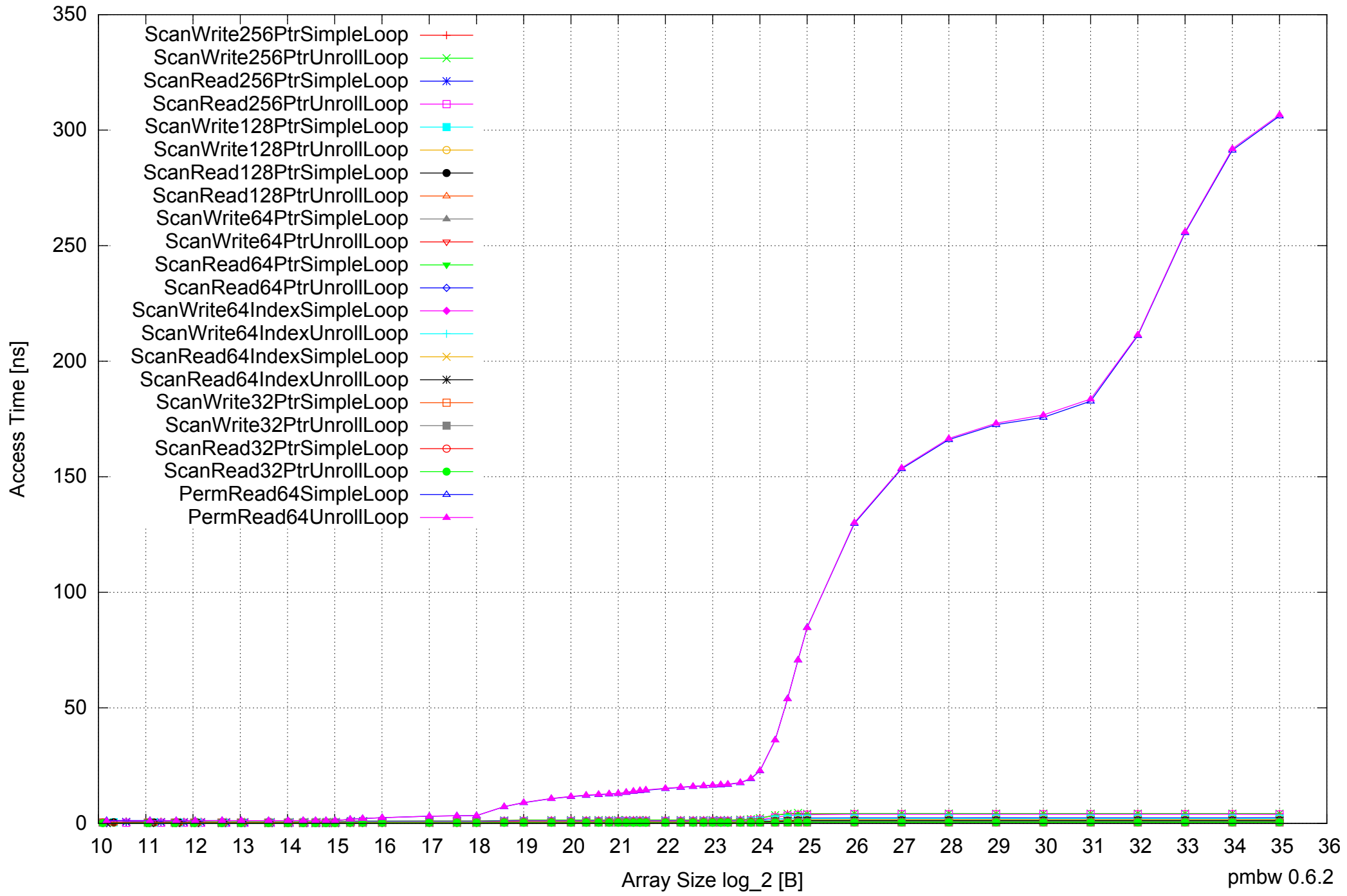
Intel Xeon E5-2670 64GB - One Thread Memory Latency (Access Time)
