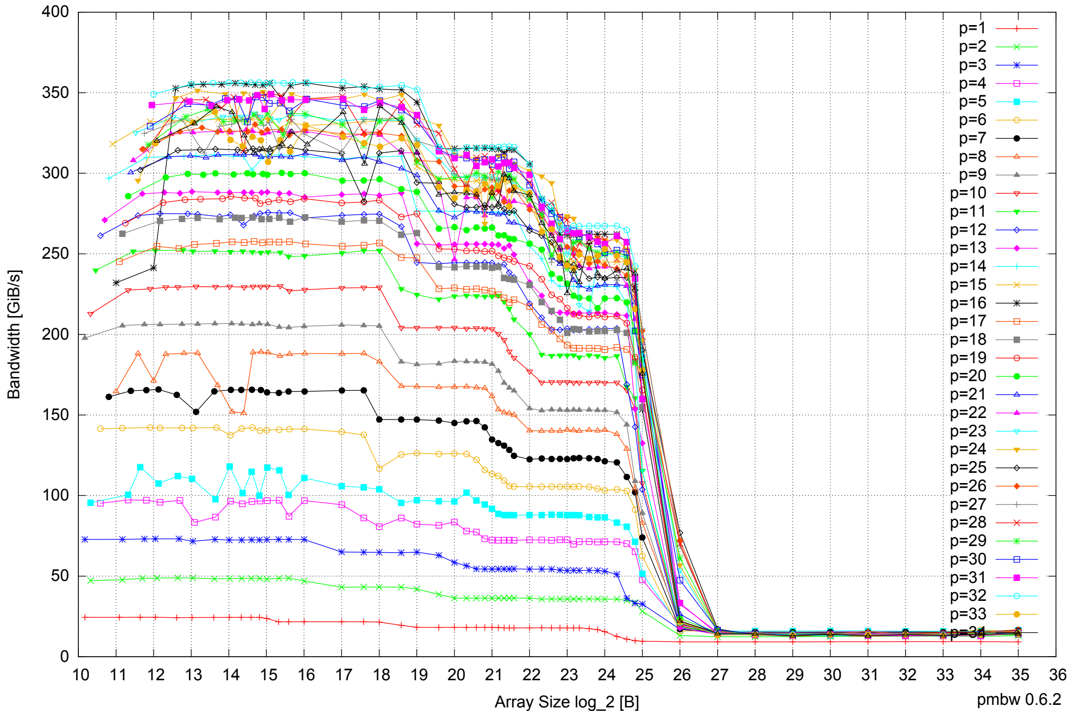
Intel Xeon E5-2670 64GB - Parallel Memory Bandwidth - ScanWrite64PtrUnrollLoop
