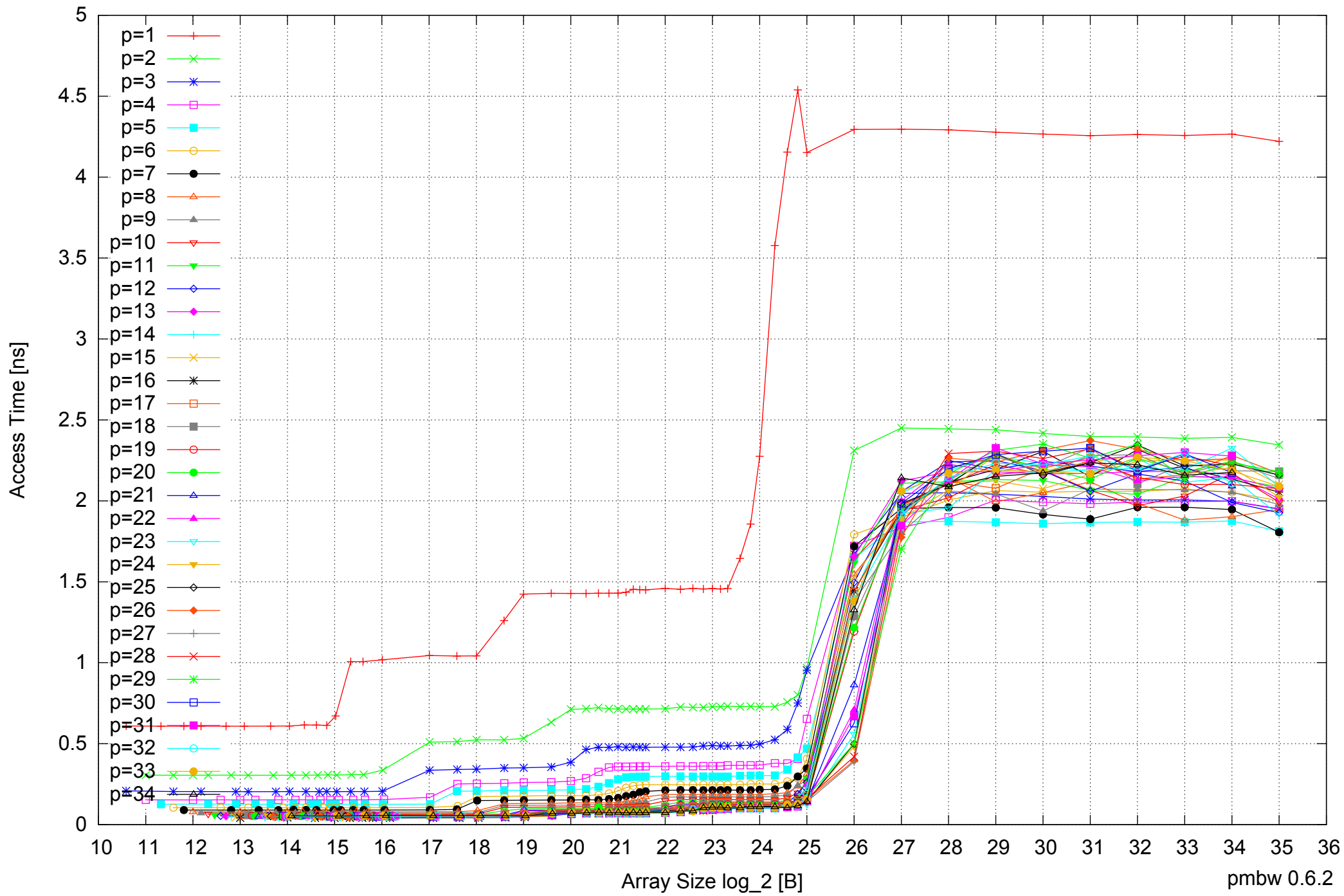
Intel Xeon E5-2670 64GB - Parallel Memory Access Time - ScanWrite256PtrUnrollLoop
