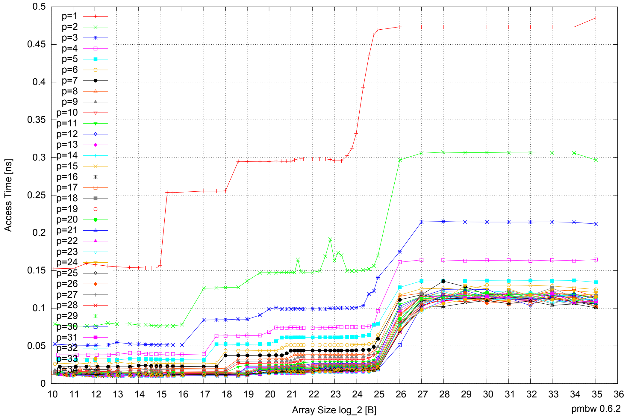
Intel Xeon E5-2670 64GB - Parallel Memory Access Time - ScanRead32PtrUnrollLoop
