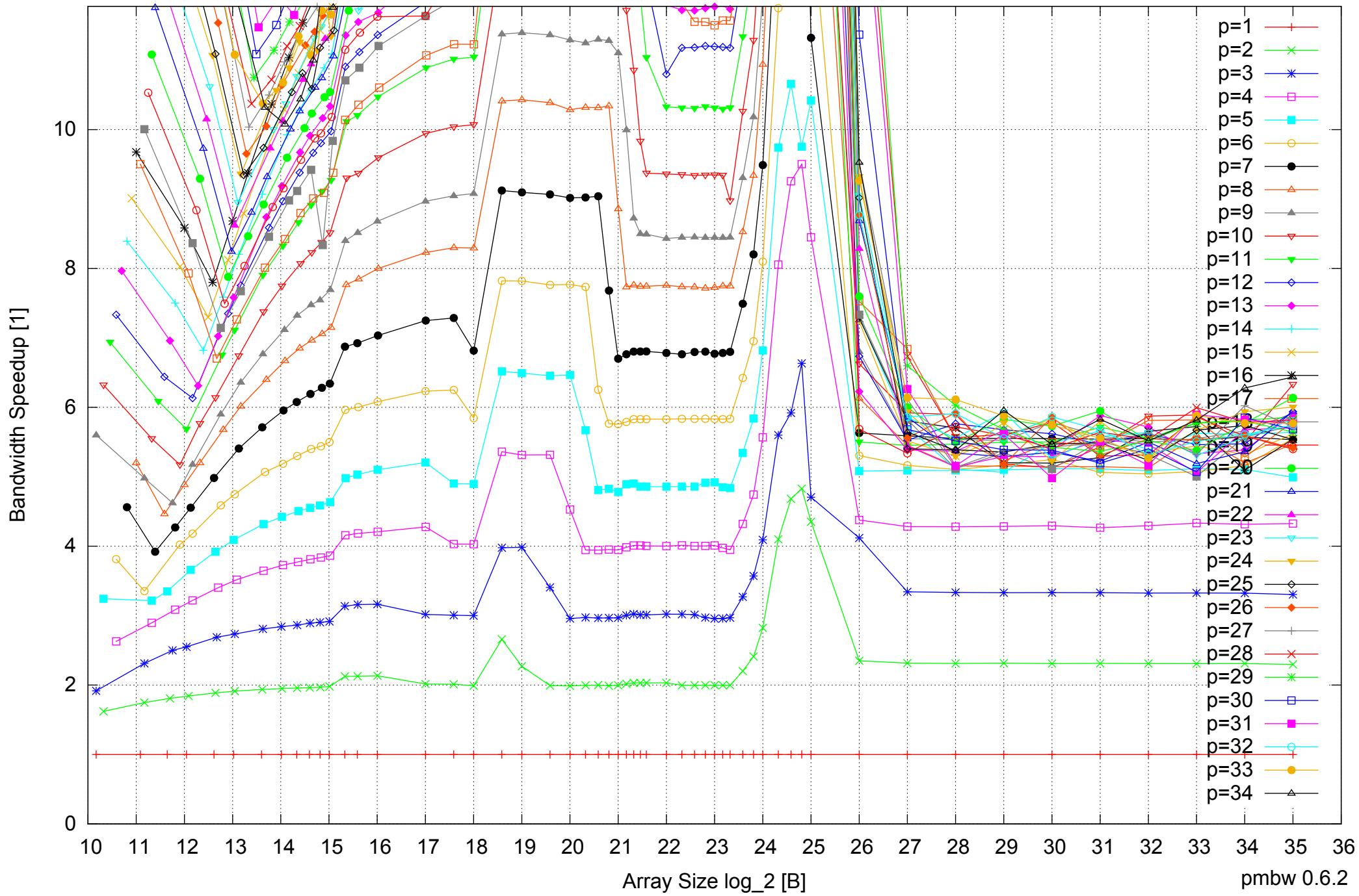
Intel Xeon E5-2670 64GB - Speedup of Parallel Memory Bandwidth (enlarged) - ScanRead64IndexSimpleLoop
