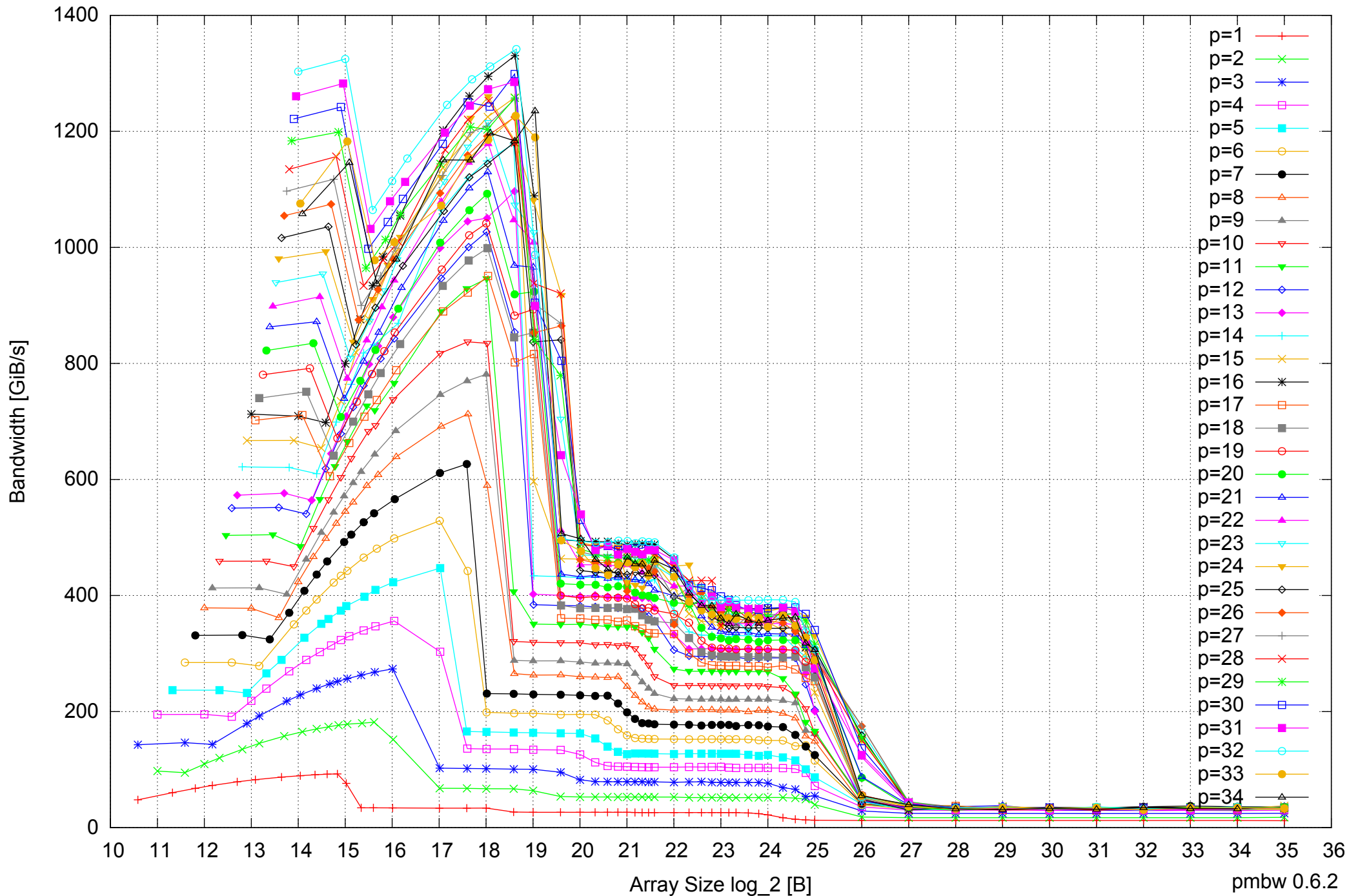
Intel Xeon E5-2670 64GB - Parallel Memory Bandwidth - ScanRead256PtrSimpleLoop
