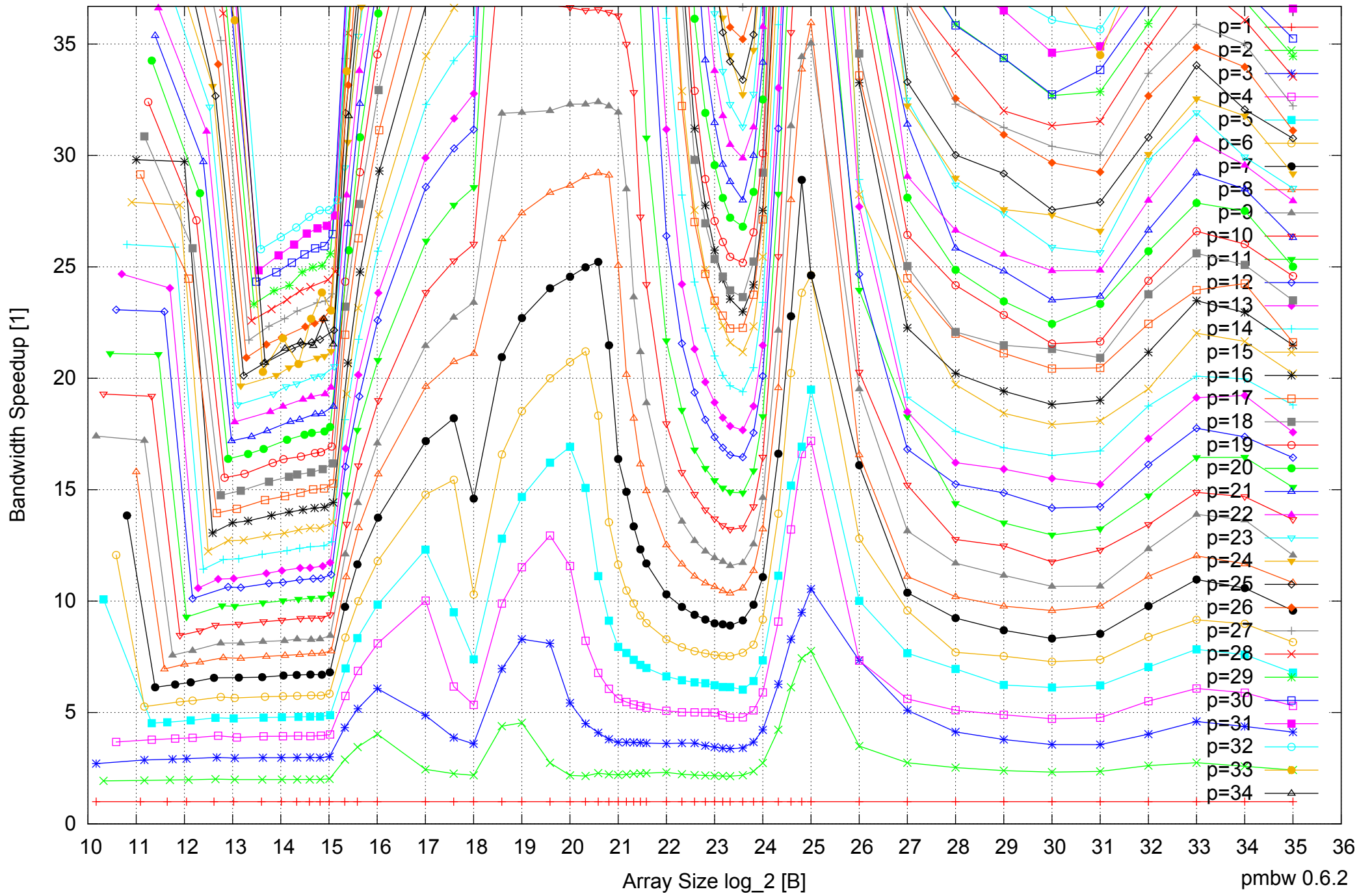
Intel Xeon E5-2670 64GB - Speedup of Parallel Memory Bandwidth (enlarged) - PermRead64SimpleLoop
