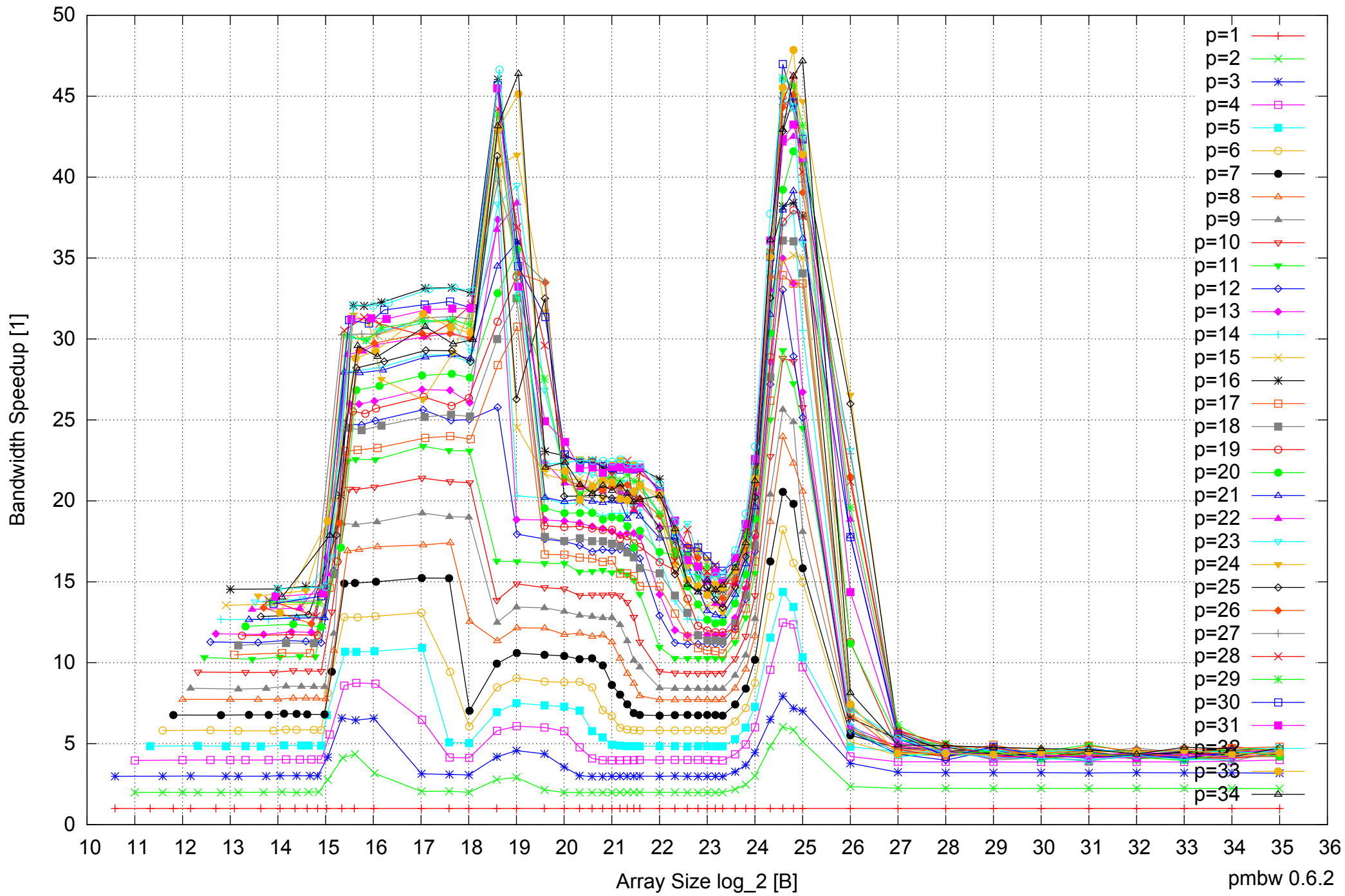
Intel Xeon E5-2670 64GB - Speedup of Parallel Memory Bandwidth - ScanRead256PtrUnrollLoop
