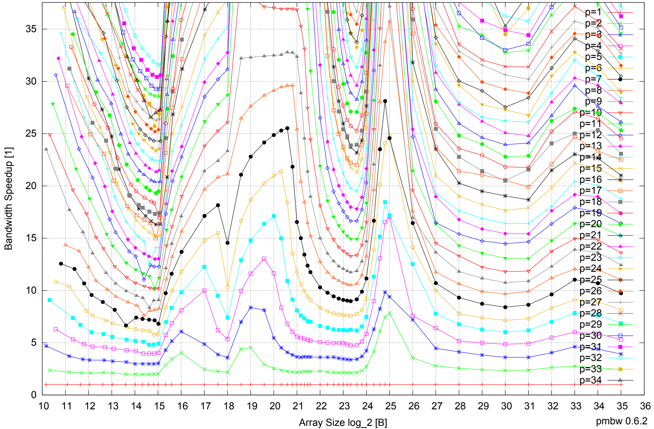
Intel Xeon E5-2670 64GB - Speedup of Parallel Memory Bandwidth (enlarged) - PermRead64UnrollLoop
