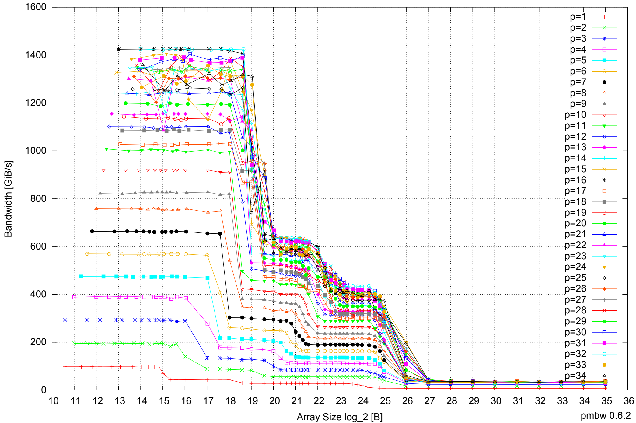
Intel Xeon E5-2670 64GB - Parallel Memory Bandwidth - ScanRead256PtrUnrollLoop
