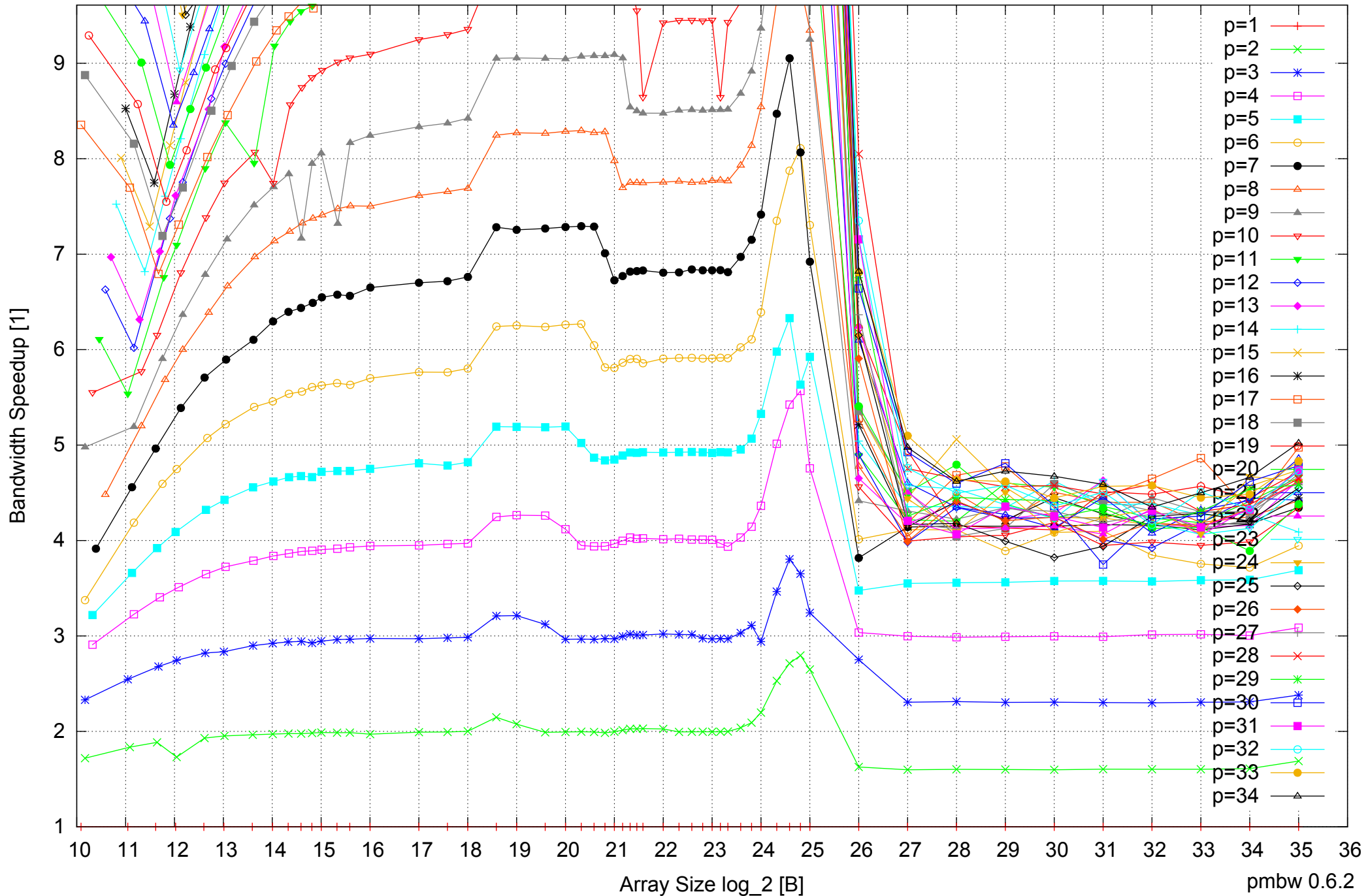
Intel Xeon E5-2670 64GB - Speedup of Parallel Memory Bandwidth (enlarged) - ScanRead32PtrSimpleLoop
