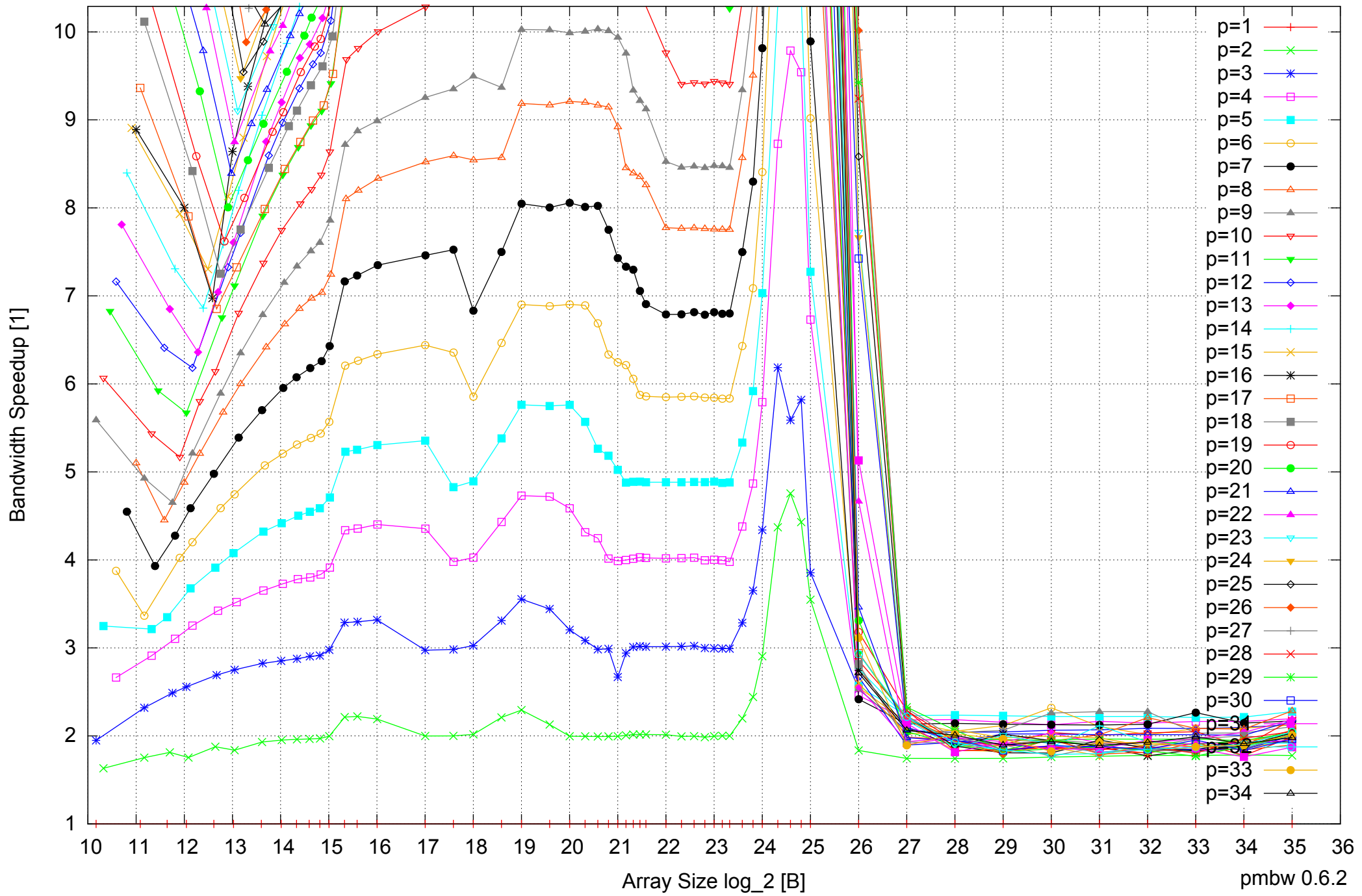
Intel Xeon E5-2670 64GB - Speedup of Parallel Memory Bandwidth (enlarged) - ScanWrite64PtrSimpleLoop
