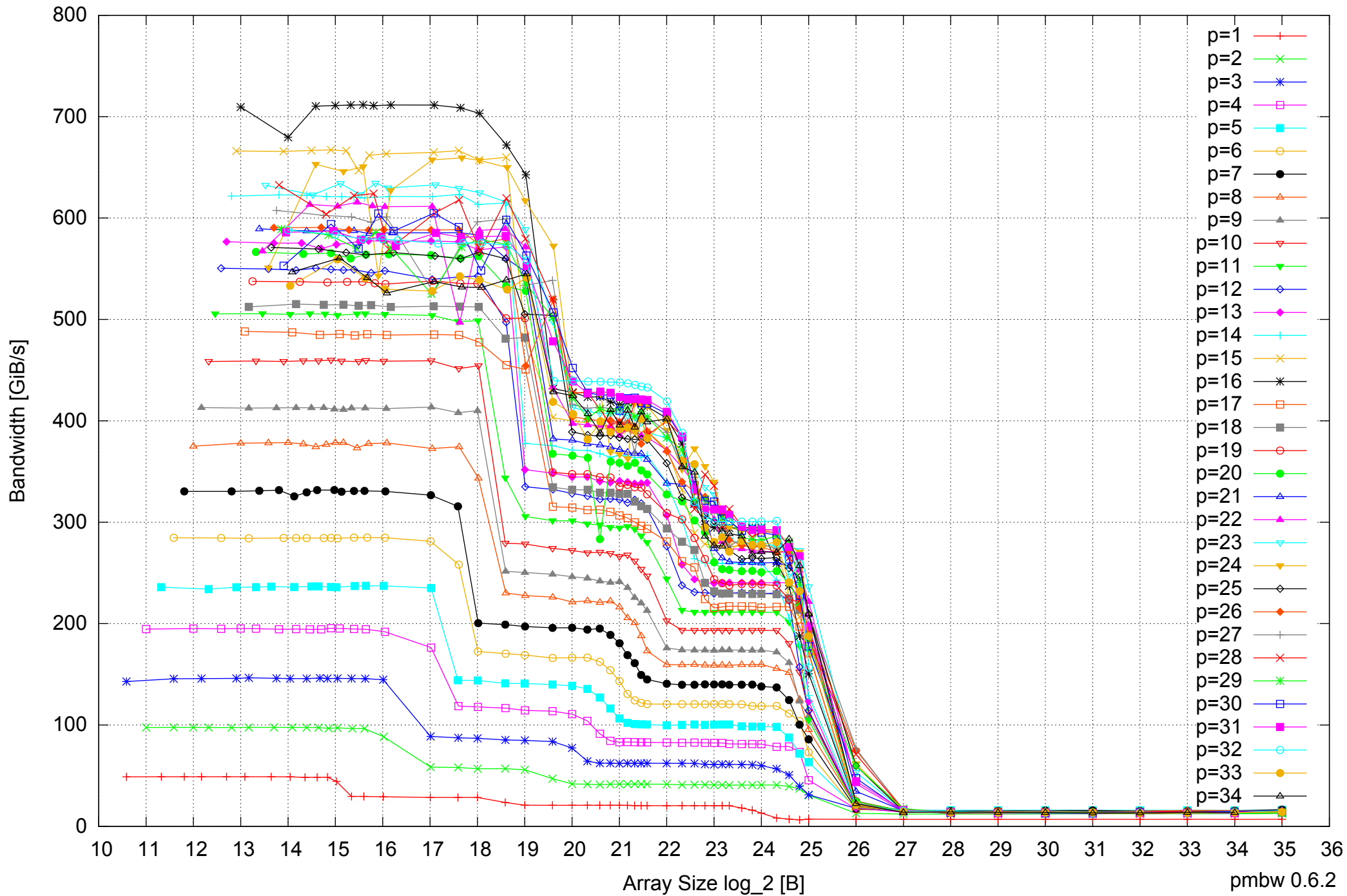
Intel Xeon E5-2670 64GB - Parallel Memory Bandwidth - ScanWrite256PtrUnrollLoop
