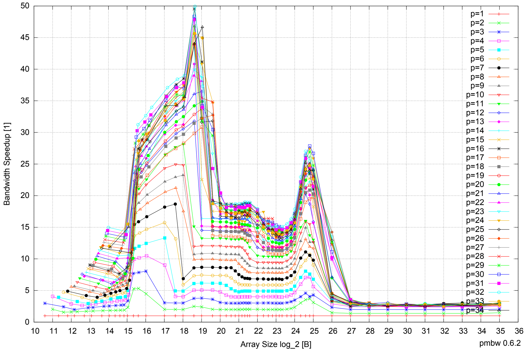
Intel Xeon E5-2670 64GB - Speedup of Parallel Memory Bandwidth - ScanRead256PtrSimpleLoop
