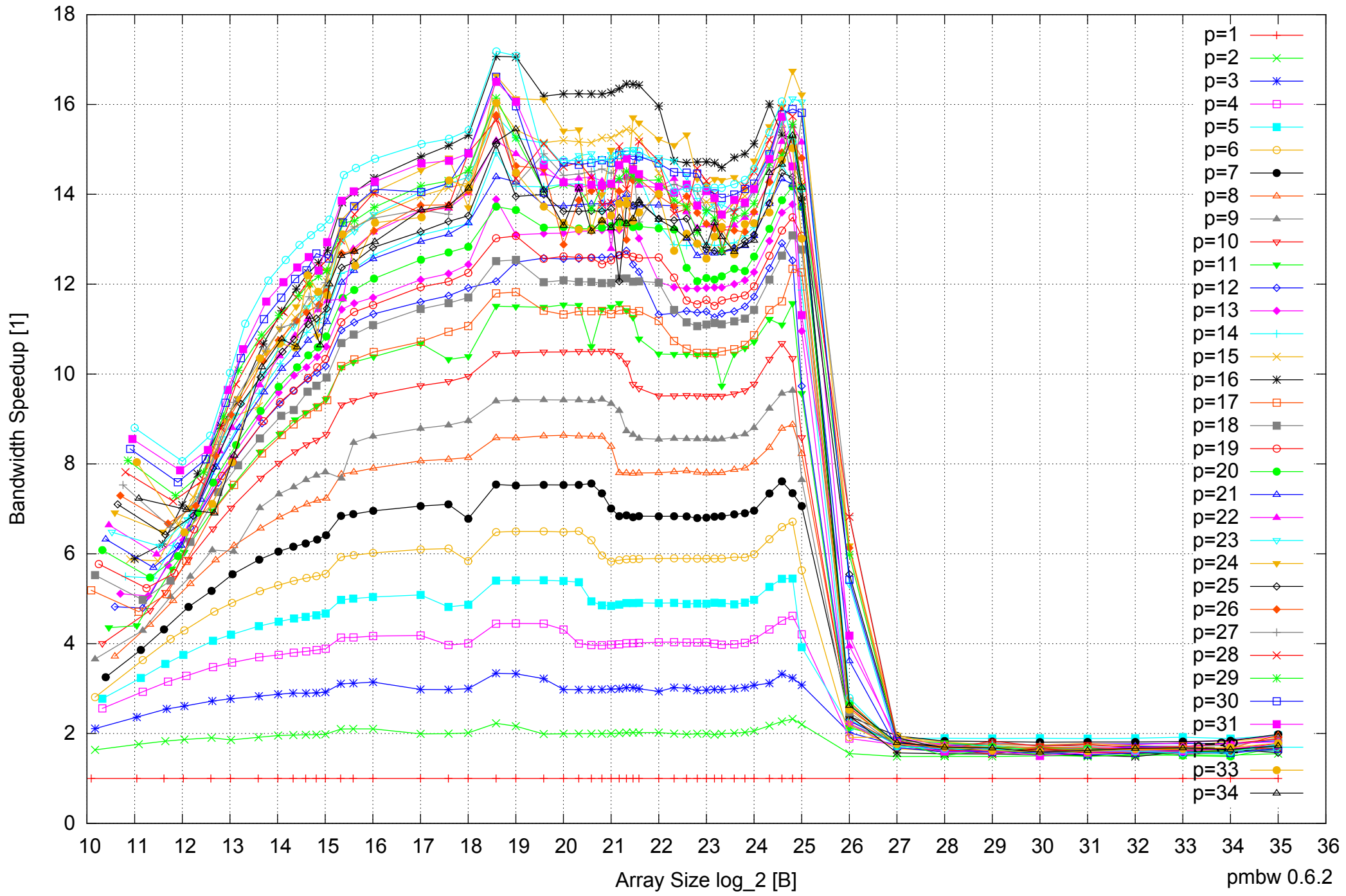
Intel Xeon E5-2670 64GB - Speedup of Parallel Memory Bandwidth - ScanWrite32PtrSimpleLoop
