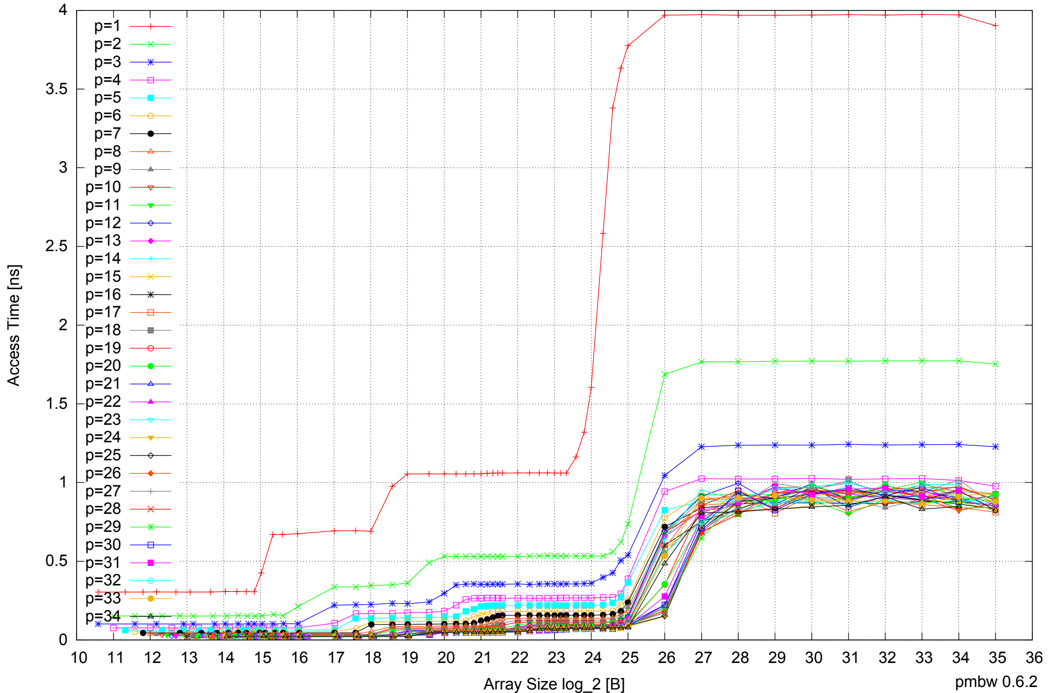
Intel Xeon E5-2670 64GB - Parallel Memory Access Time - ScanRead256PtrUnrollLoop
