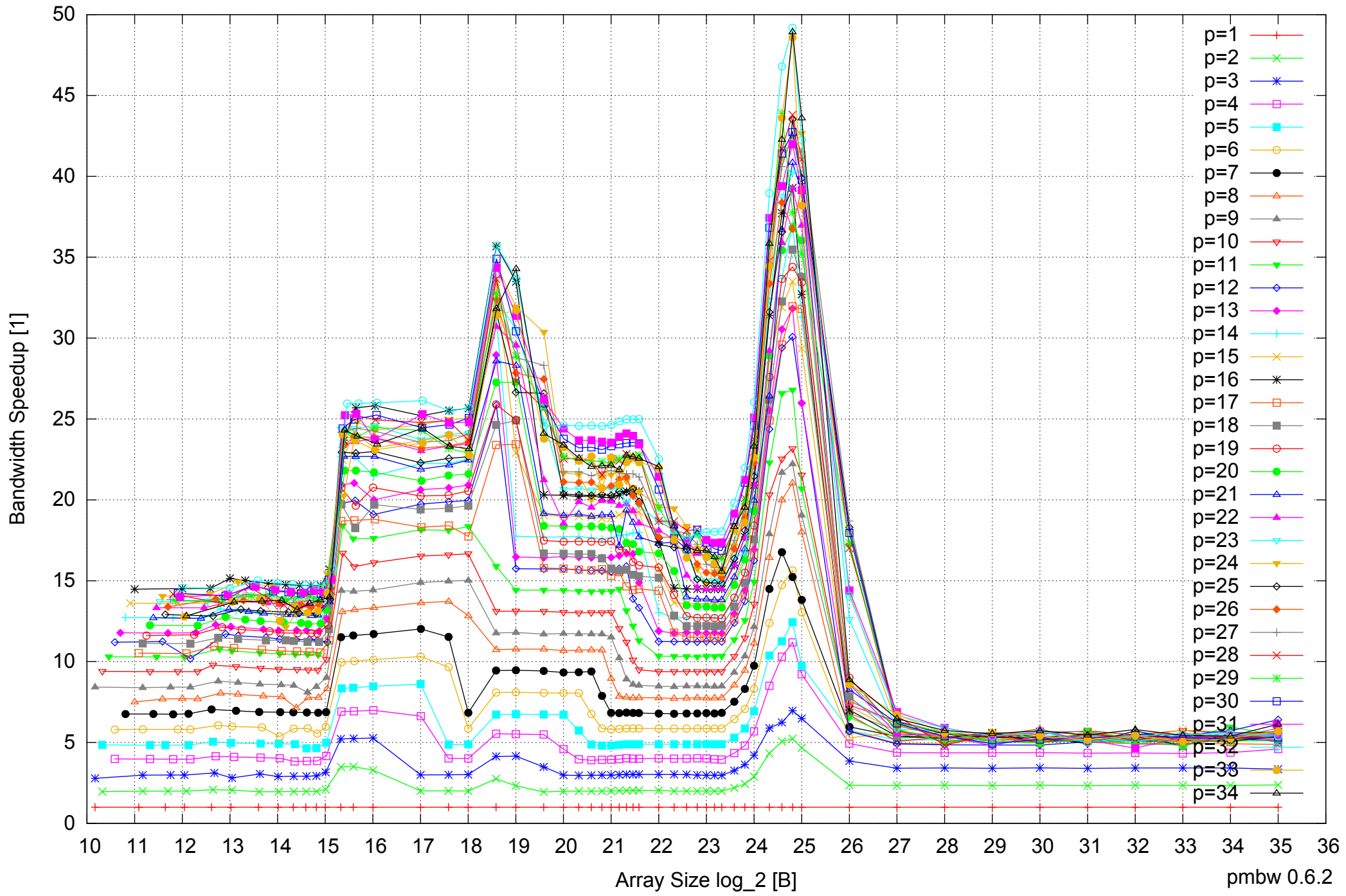
Intel Xeon E5-2670 64GB - Speedup of Parallel Memory Bandwidth - ScanRead64IndexUnrollLoop
