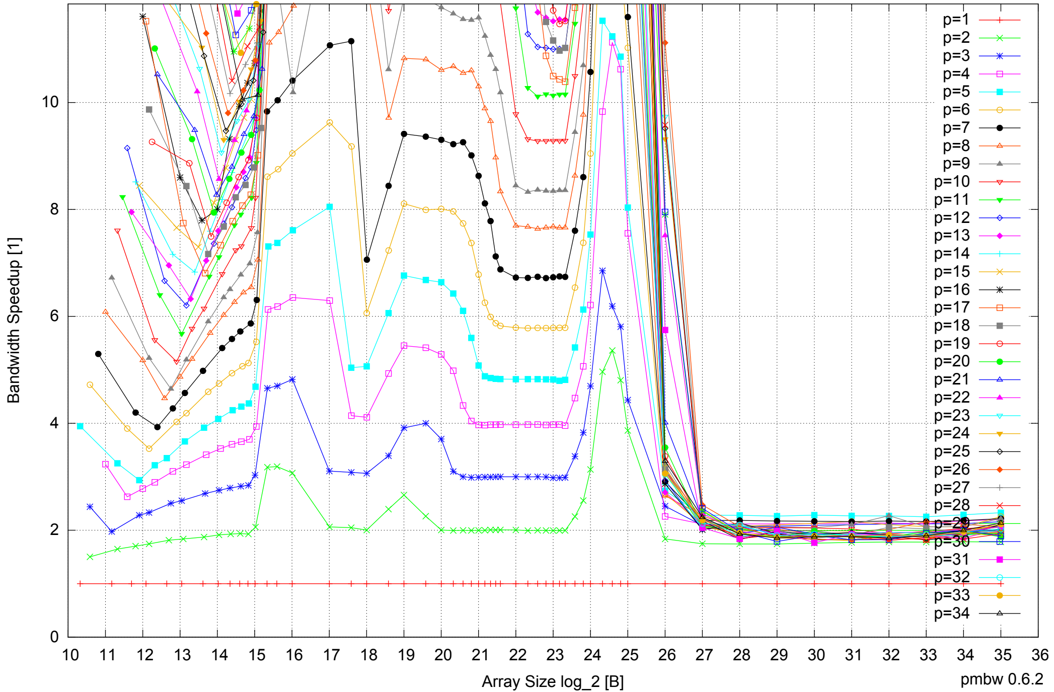
Intel Xeon E5-2670 64GB - Speedup of Parallel Memory Bandwidth (enlarged) - ScanWrite128PtrSimpleLoop
