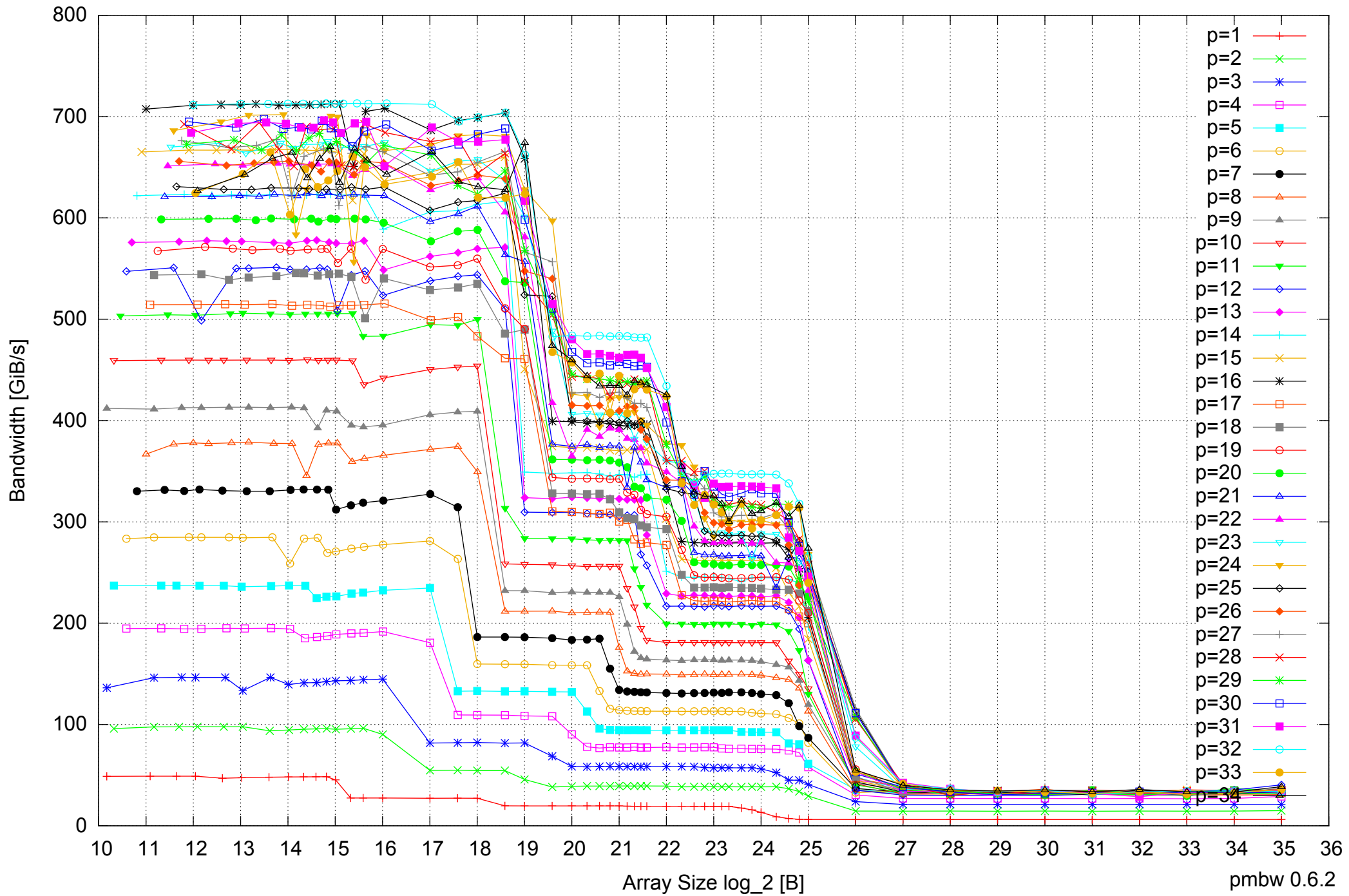
Intel Xeon E5-2670 64GB - Parallel Memory Bandwidth - ScanRead64IndexUnrollLoop
