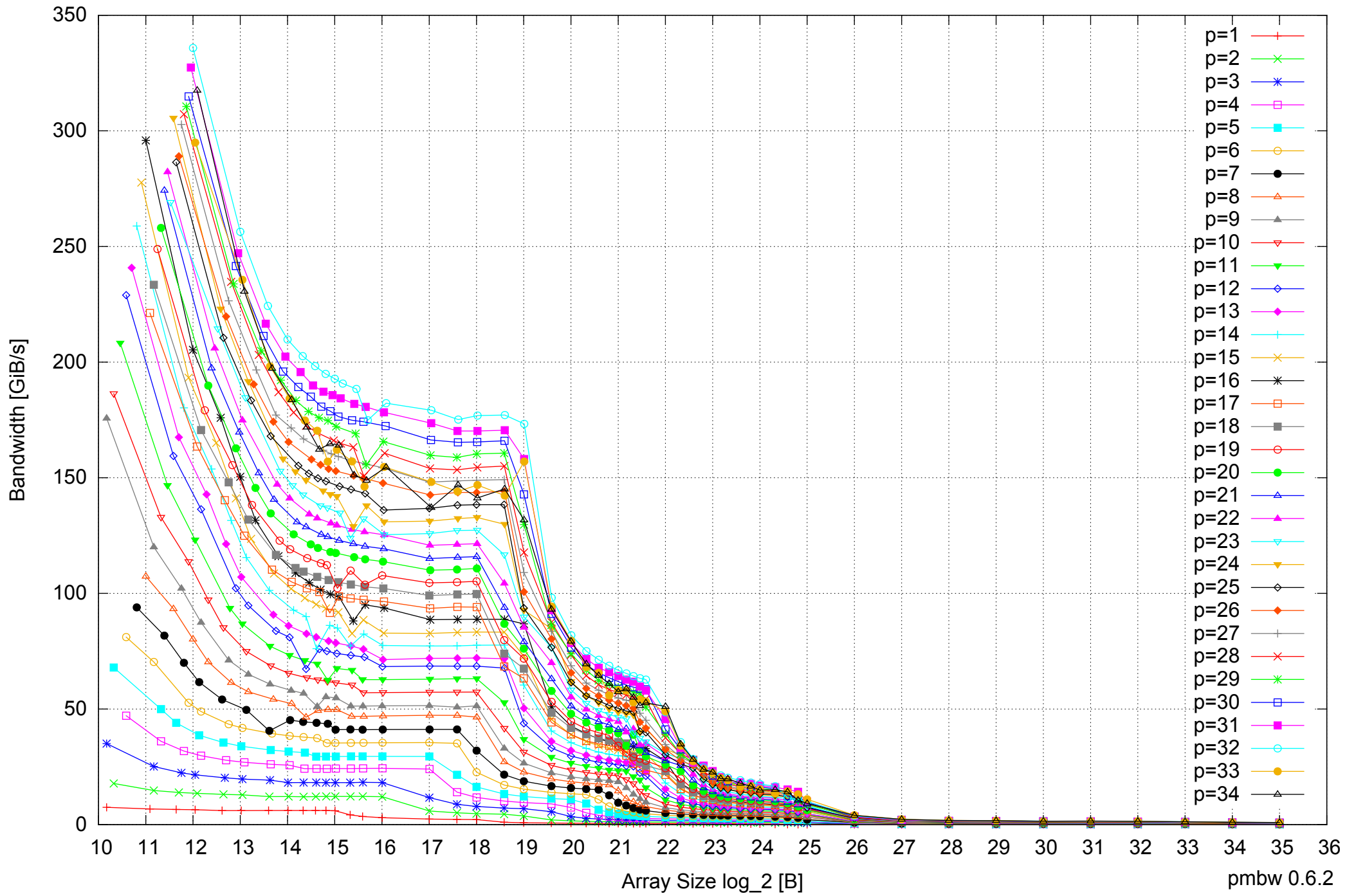
Intel Xeon E5-2670 64GB - Parallel Memory Bandwidth - PermRead64UnrollLoop
