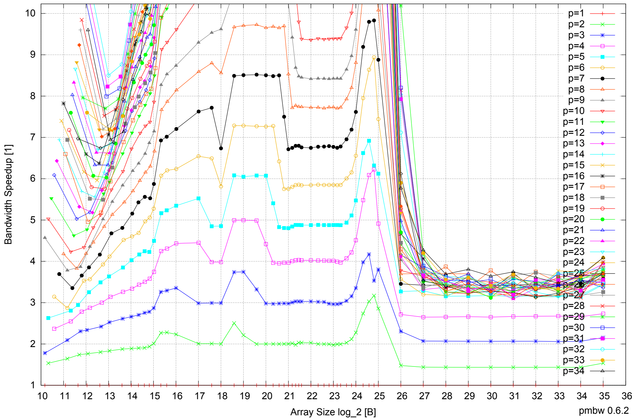
Intel Xeon E5-2670 64GB - Speedup of Parallel Memory Bandwidth (enlarged) - ScanRead64PtrSimpleLoop
