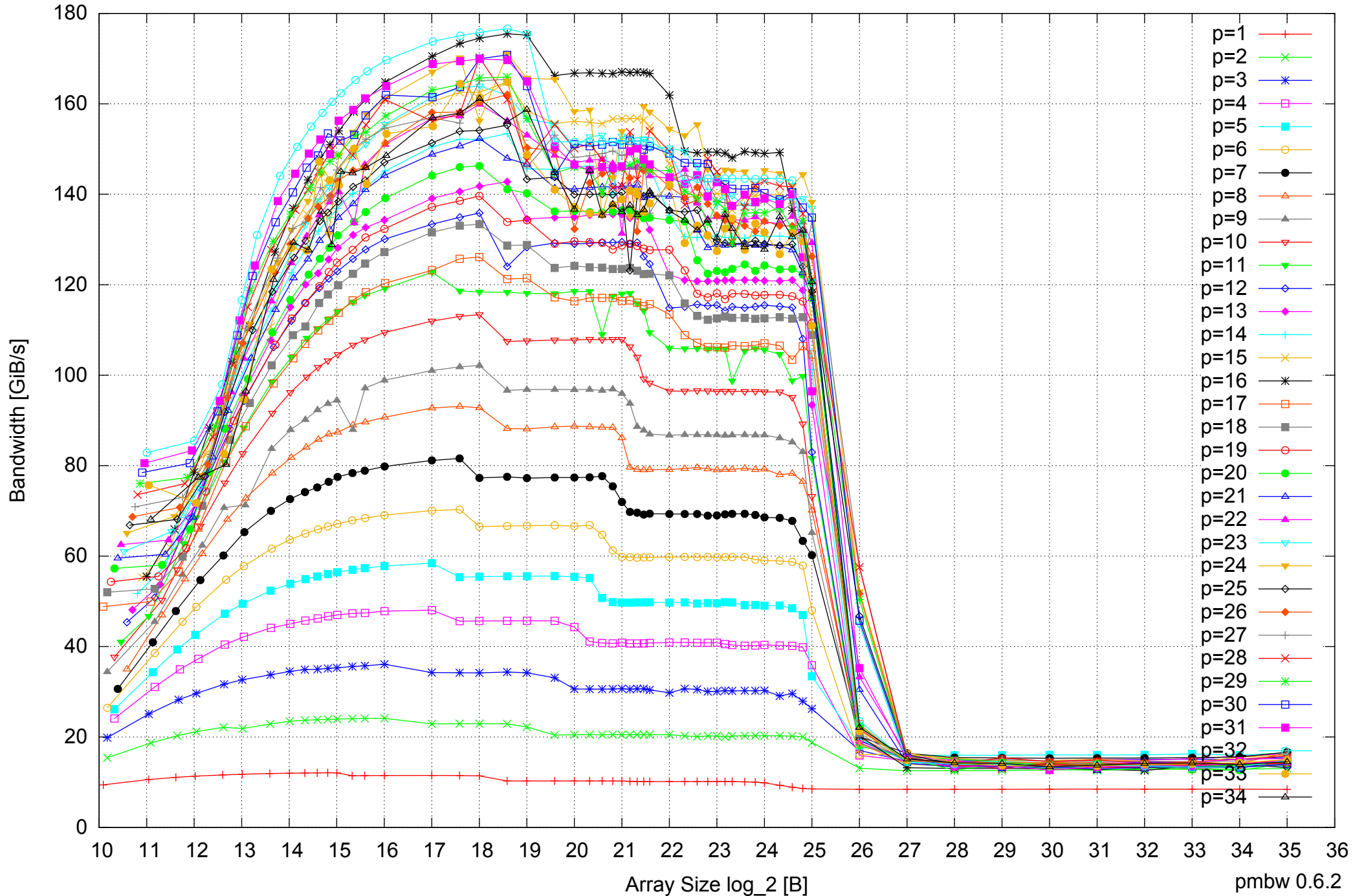
Intel Xeon E5-2670 64GB - Parallel Memory Bandwidth - ScanWrite32PtrSimpleLoop
