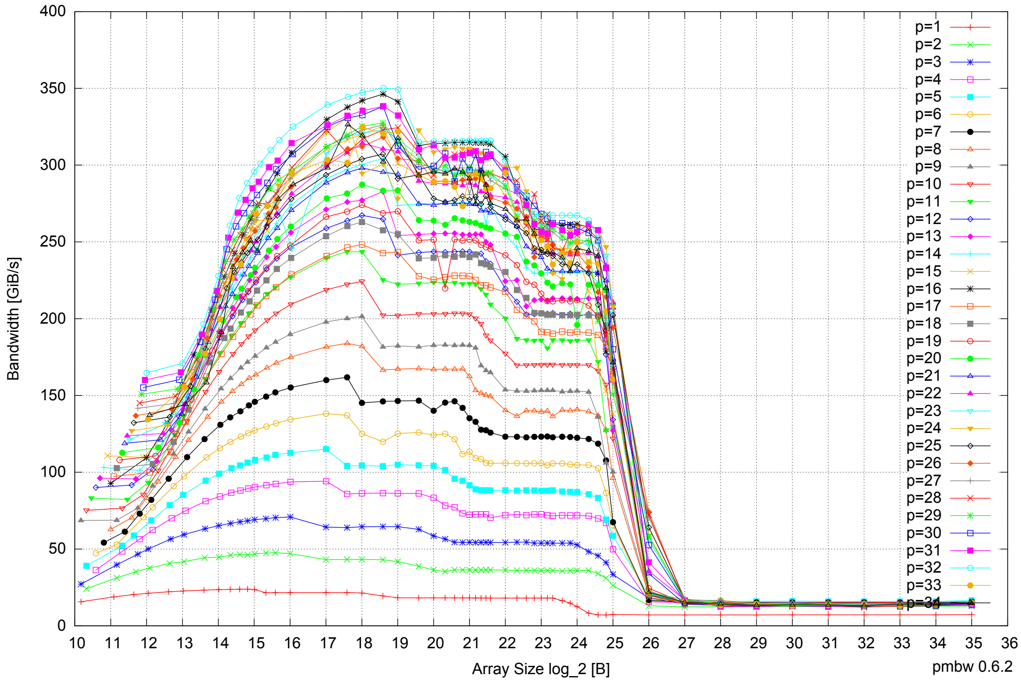
Intel Xeon E5-2670 64GB - Parallel Memory Bandwidth - ScanWrite64IndexSimpleLoop
