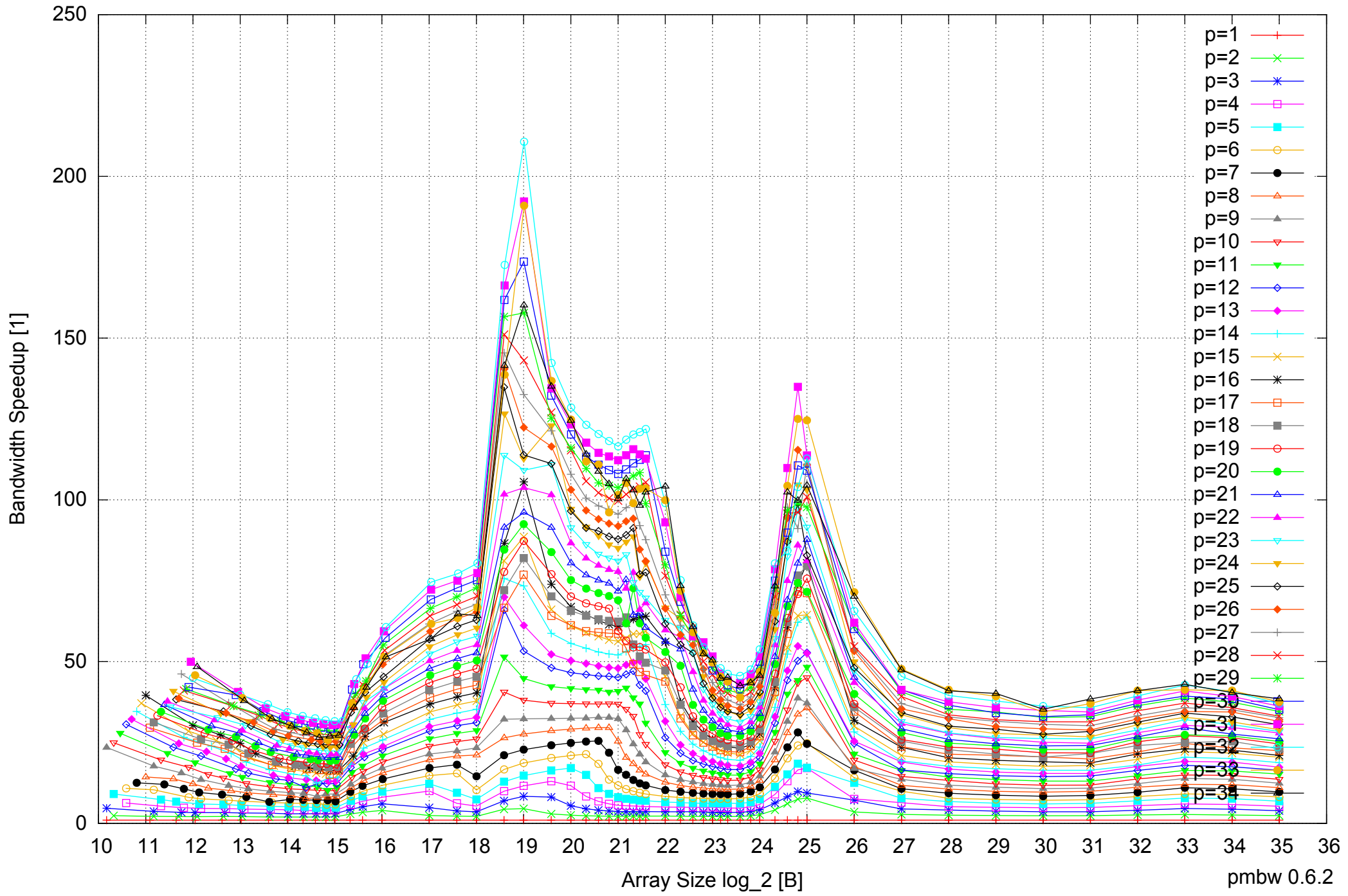
Intel Xeon E5-2670 64GB - Speedup of Parallel Memory Bandwidth - PermRead64UnrollLoop
