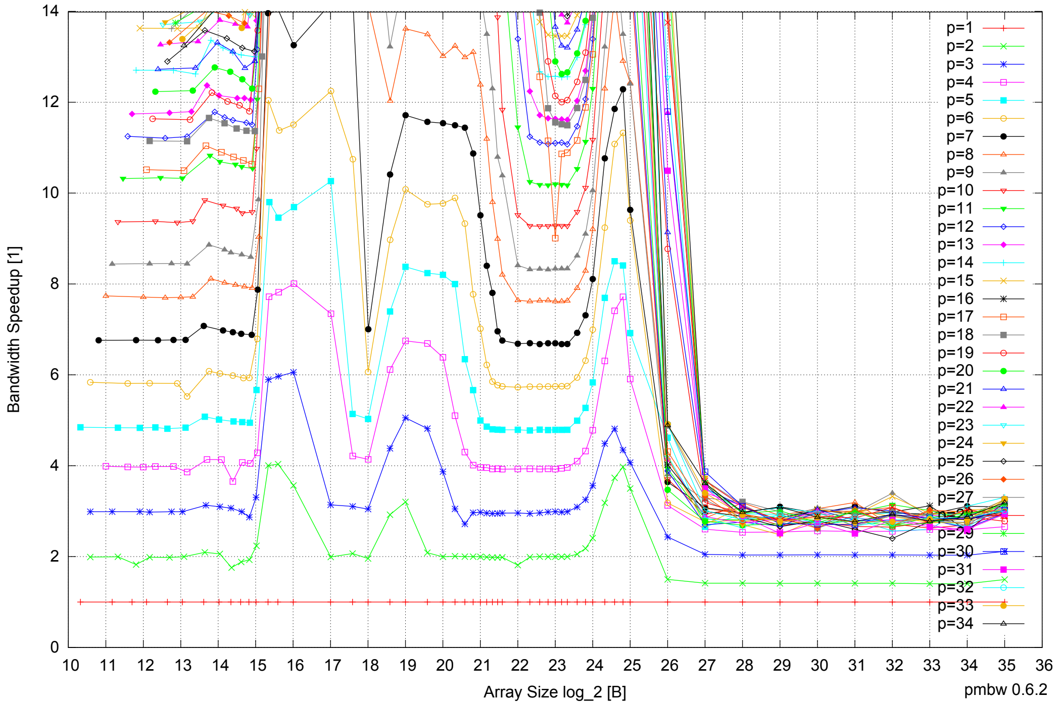
Intel Xeon E5-2670 64GB - Speedup of Parallel Memory Bandwidth (enlarged) - ScanRead128PtrUnrollLoop
