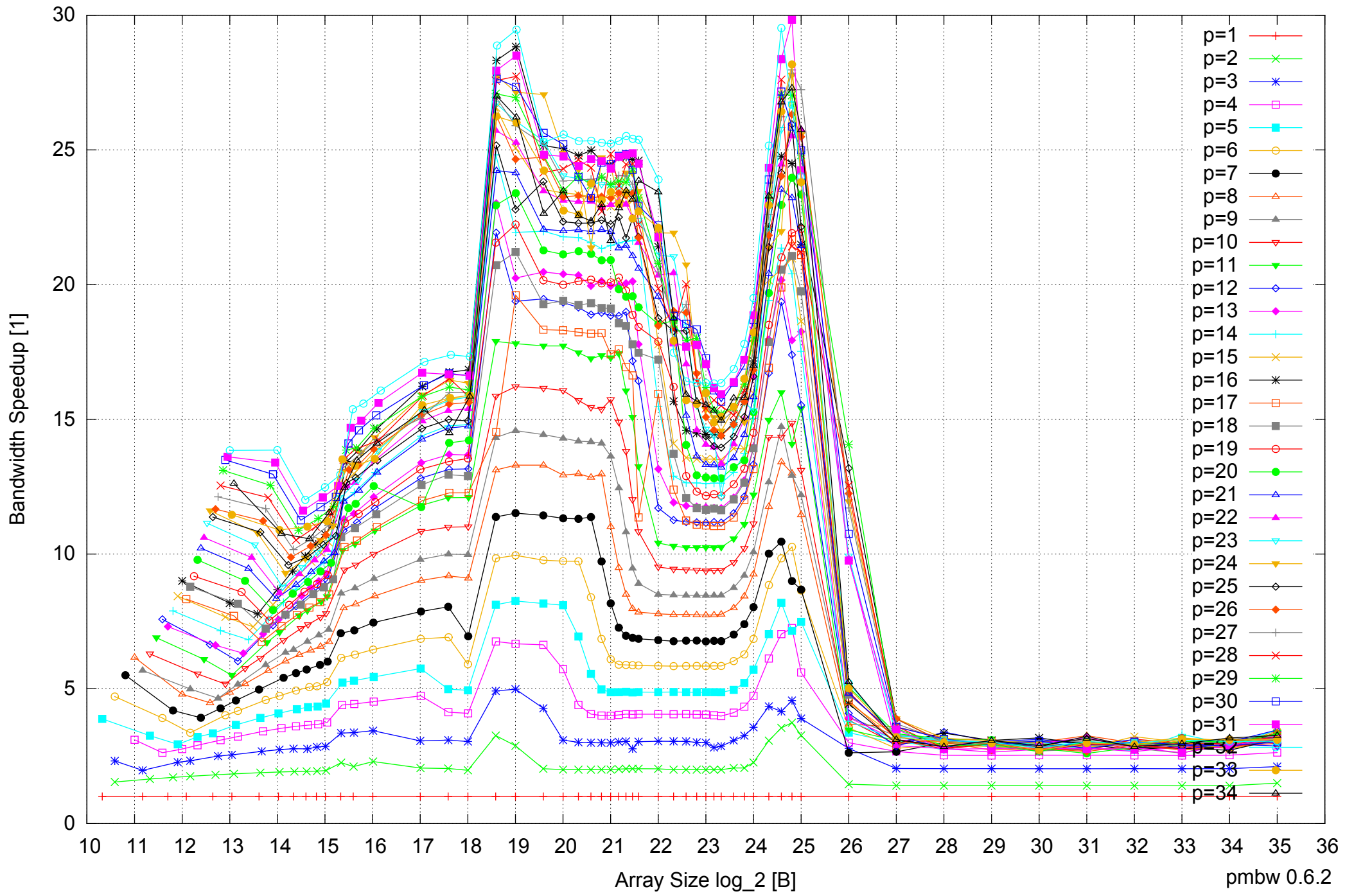
Intel Xeon E5-2670 64GB - Speedup of Parallel Memory Bandwidth - ScanRead128PtrSimpleLoop
