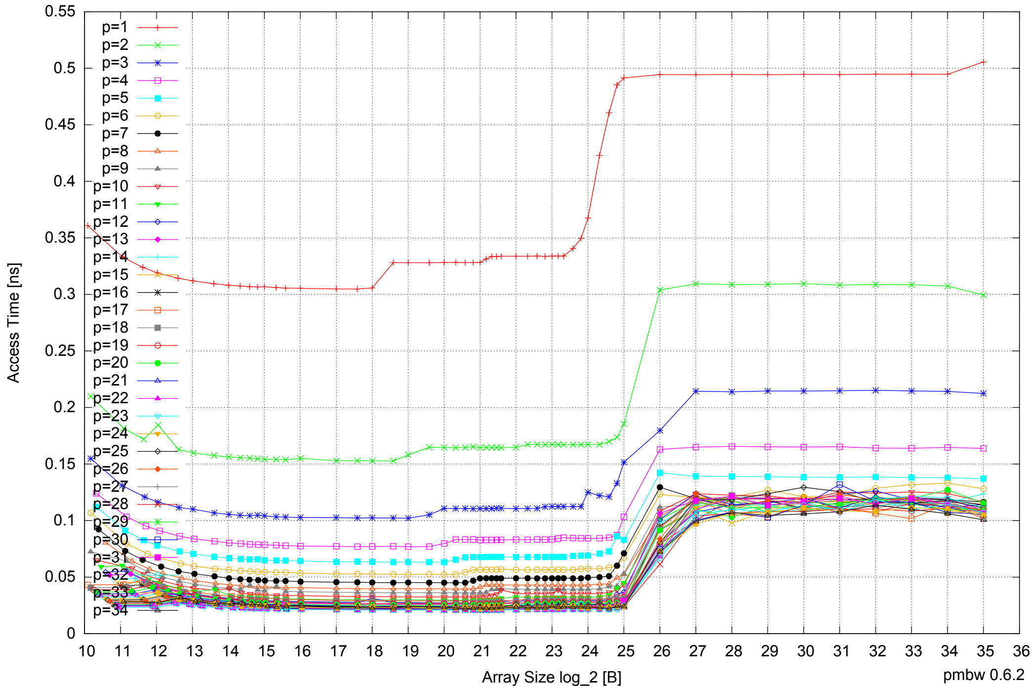
Intel Xeon E5-2670 64GB - Parallel Memory Access Time - ScanRead32PtrSimpleLoop
