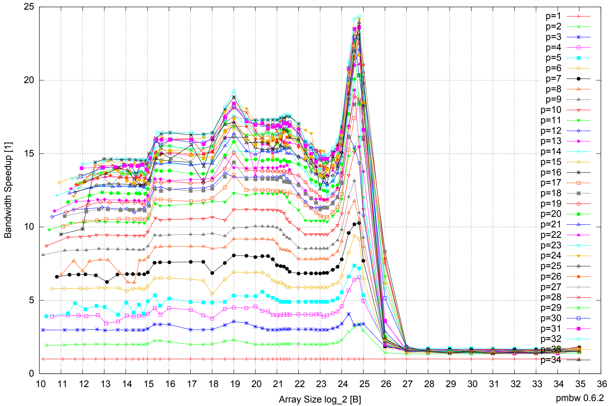
Intel Xeon E5-2670 64GB - Speedup of Parallel Memory Bandwidth - ScanWrite64PtrUnrollLoop
