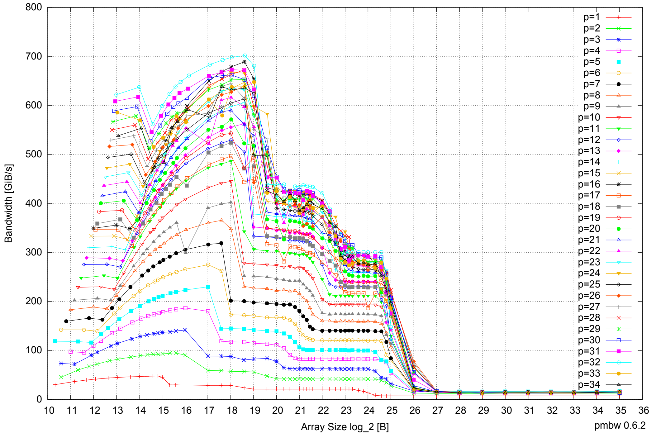
Intel Xeon E5-2670 64GB - Parallel Memory Bandwidth - ScanWrite128PtrSimpleLoop
