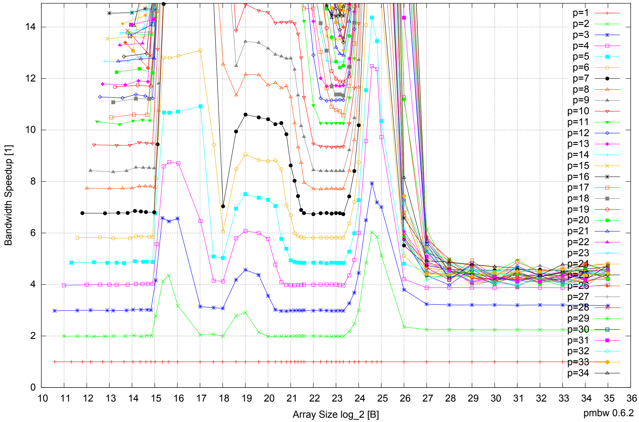
Intel Xeon E5-2670 64GB - Speedup of Parallel Memory Bandwidth (enlarged) - ScanRead256PtrUnrollLoop
