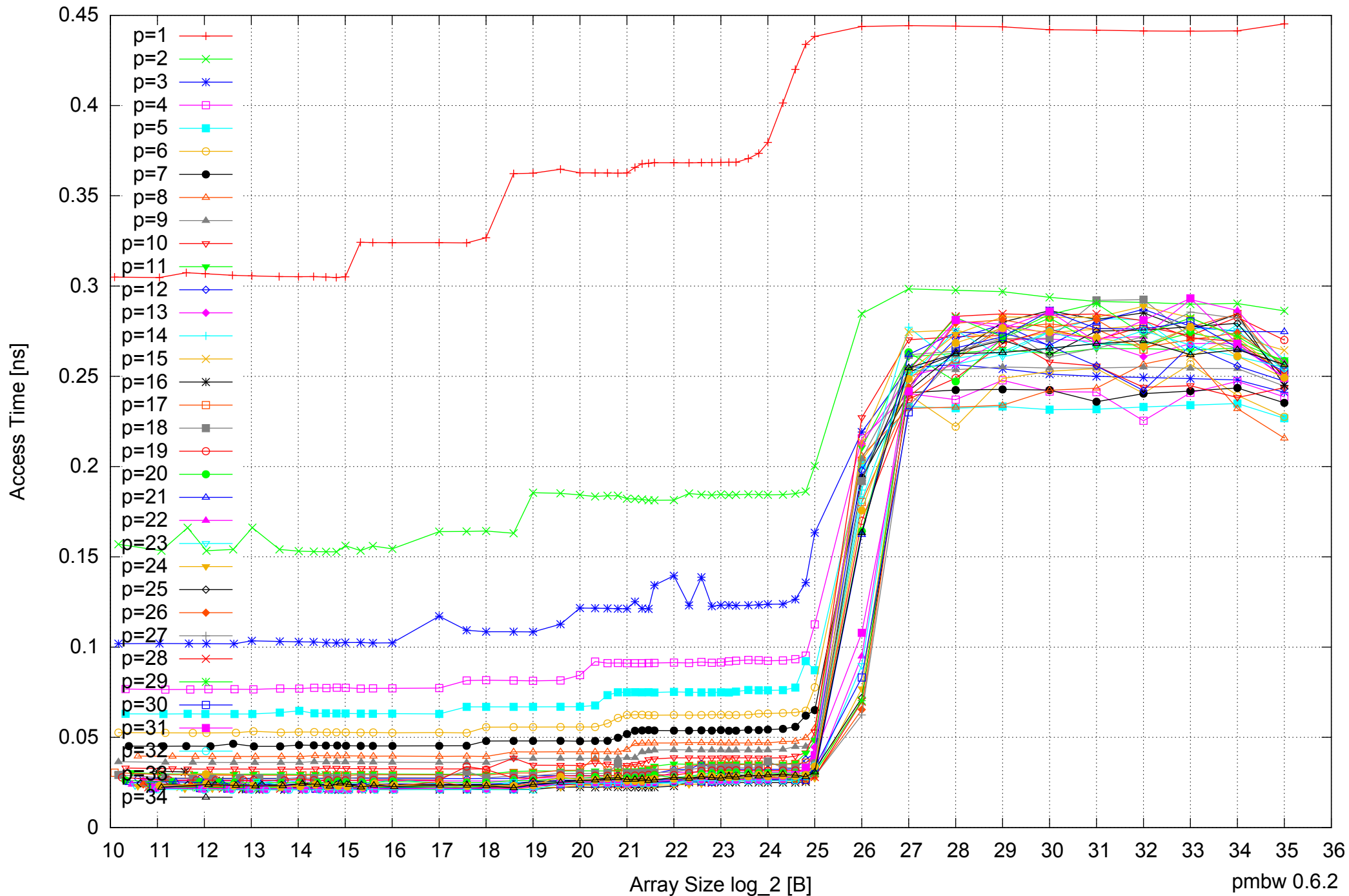
Intel Xeon E5-2670 64GB - Parallel Memory Access Time - ScanWrite32PtrUnrollLoop
