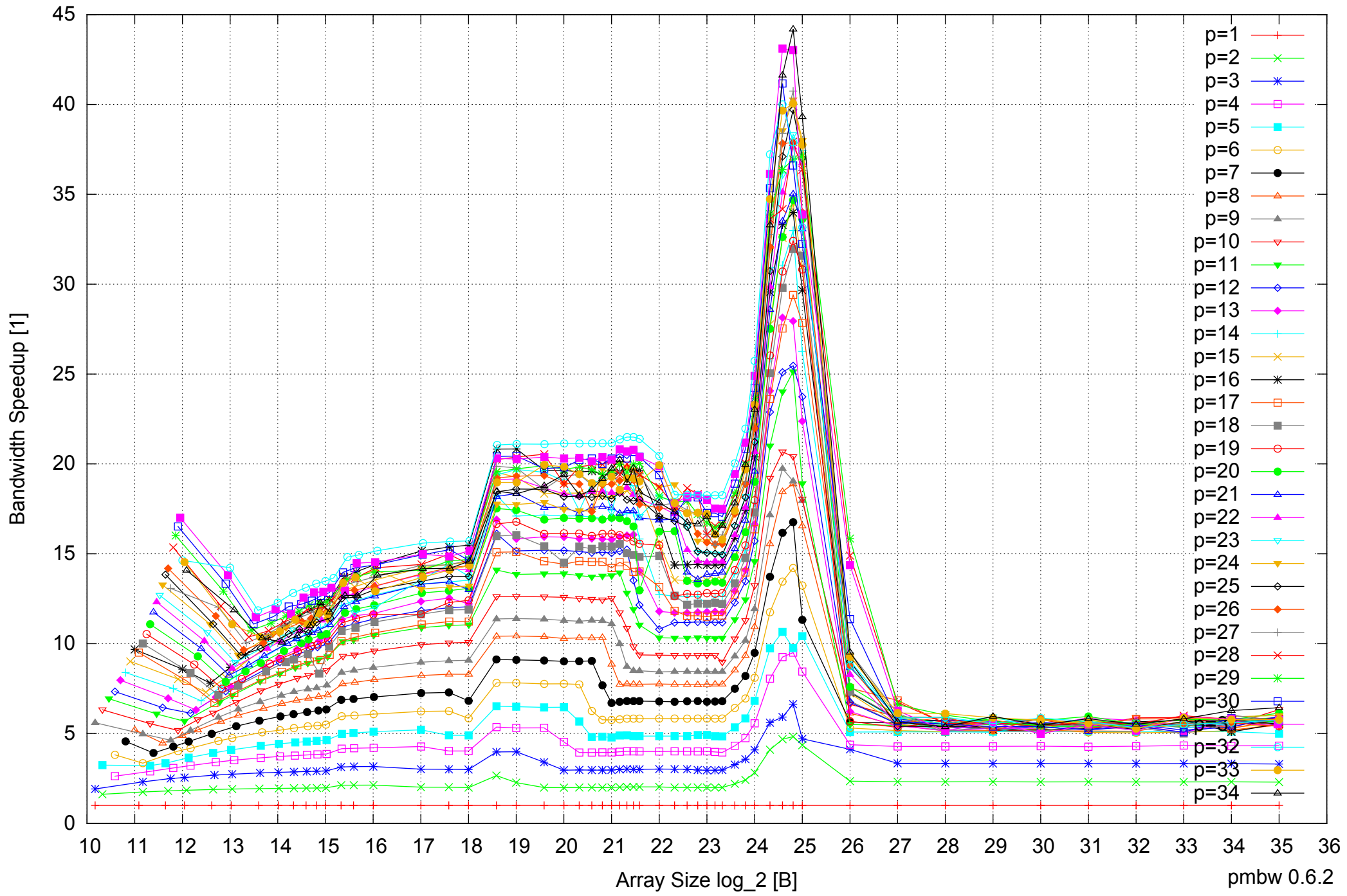
Intel Xeon E5-2670 64GB - Speedup of Parallel Memory Bandwidth - ScanRead64IndexSimpleLoop
