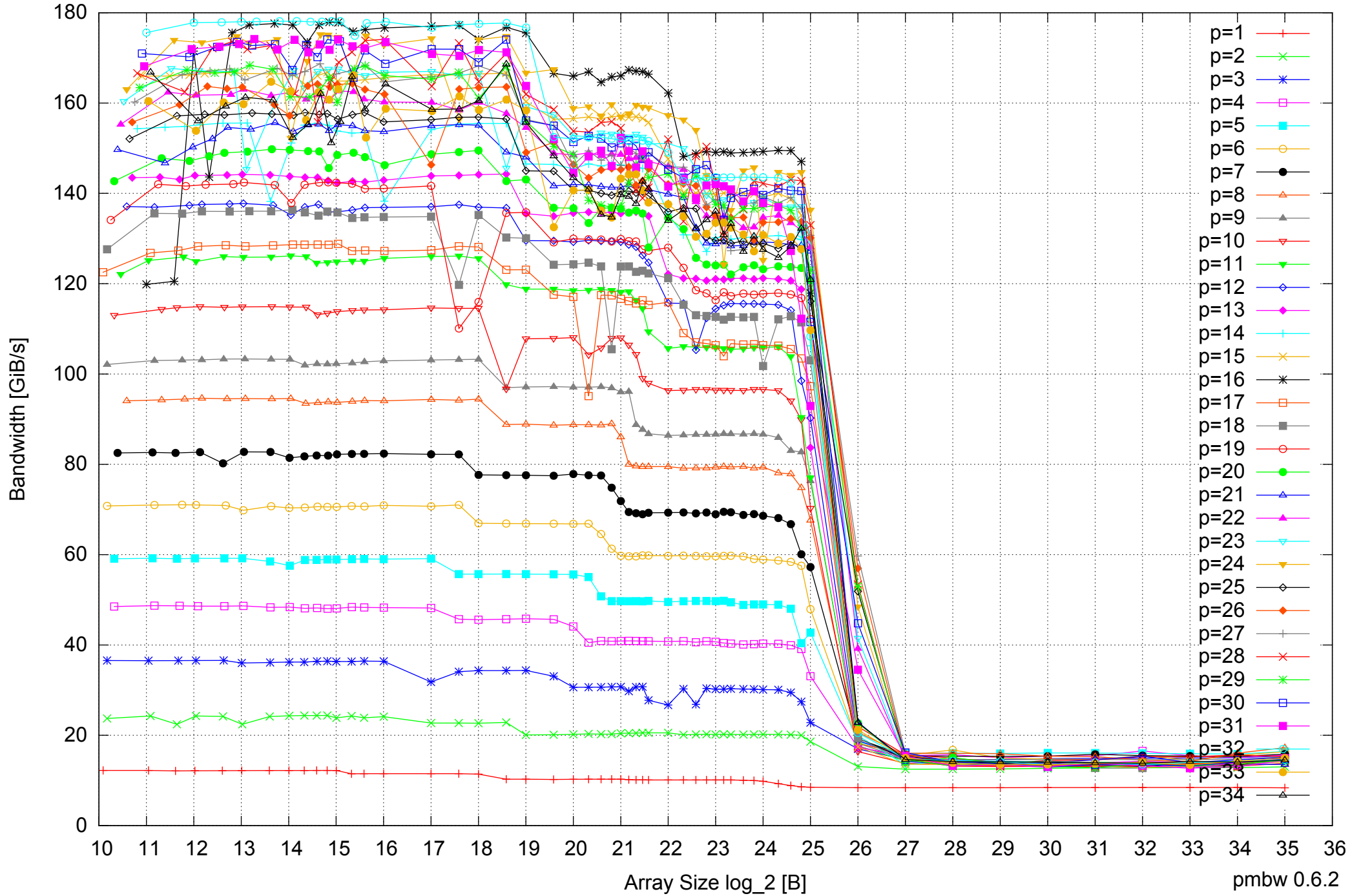
Intel Xeon E5-2670 64GB - Parallel Memory Bandwidth - ScanWrite32PtrUnrollLoop
