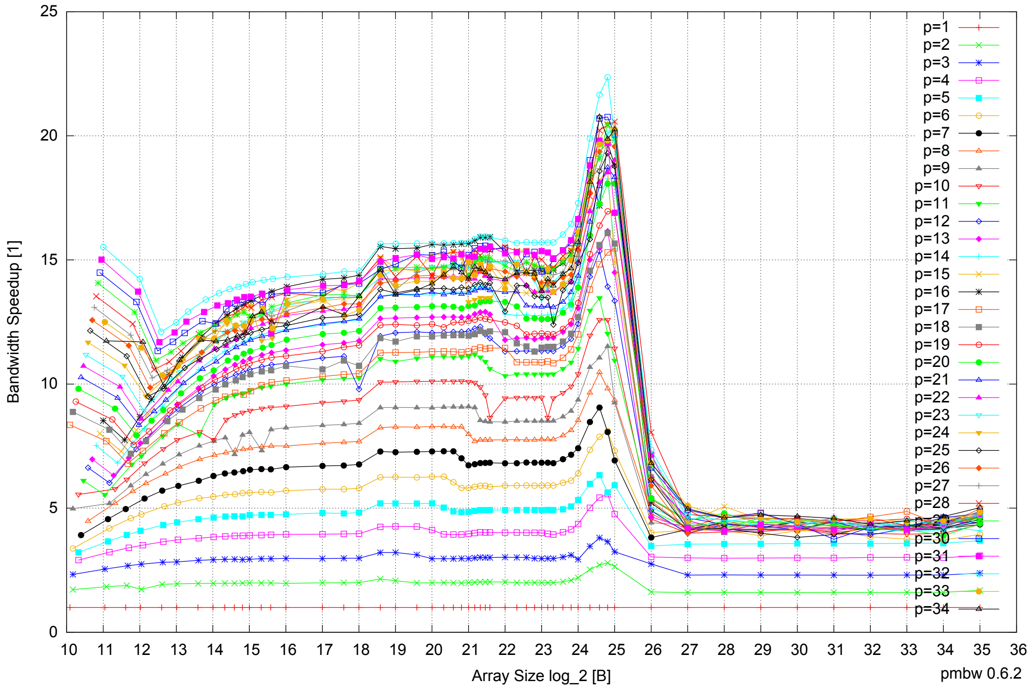
Intel Xeon E5-2670 64GB - Speedup of Parallel Memory Bandwidth - ScanRead32PtrSimpleLoop
