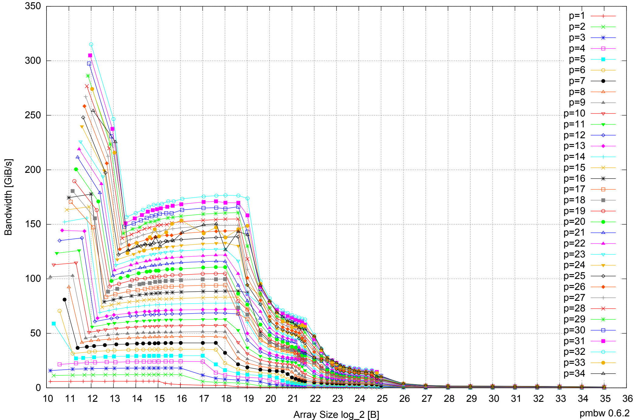
Intel Xeon E5-2670 64GB - Parallel Memory Bandwidth - PermRead64SimpleLoop
