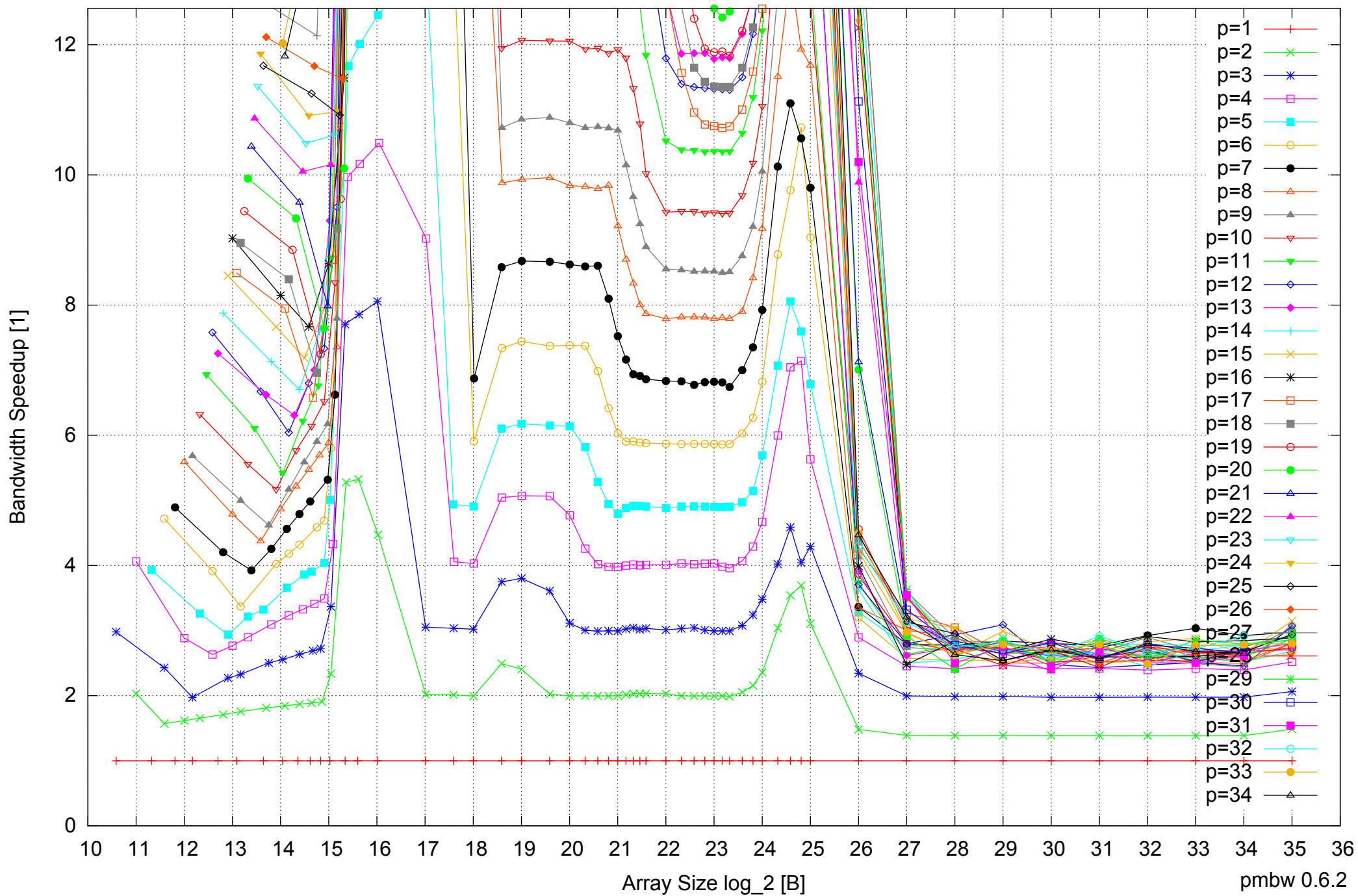
Intel Xeon E5-2670 64GB - Speedup of Parallel Memory Bandwidth (enlarged) - ScanRead256PtrSimpleLoop
