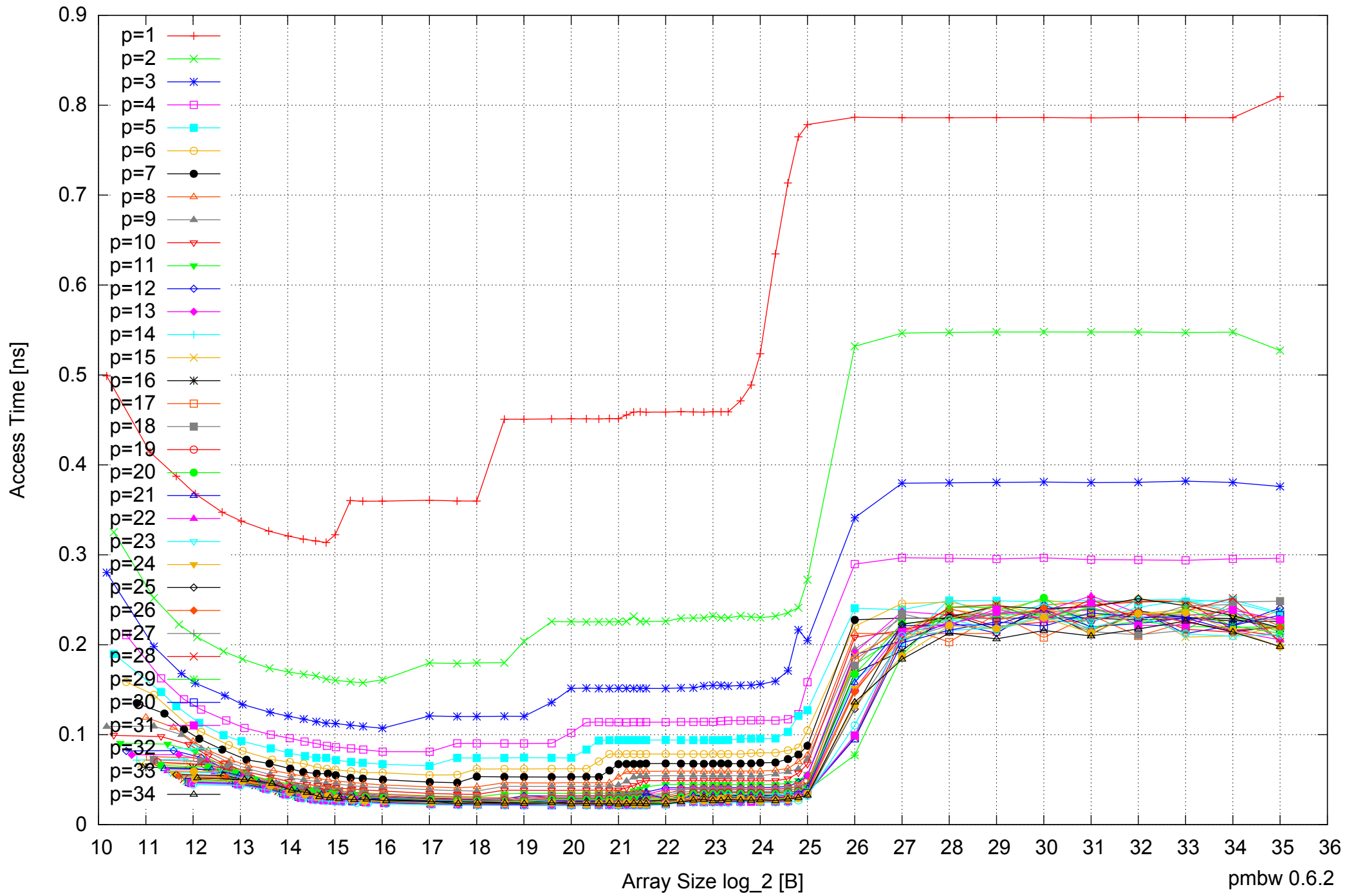
Intel Xeon E5-2670 64GB - Parallel Memory Access Time - ScanRead64PtrSimpleLoop
