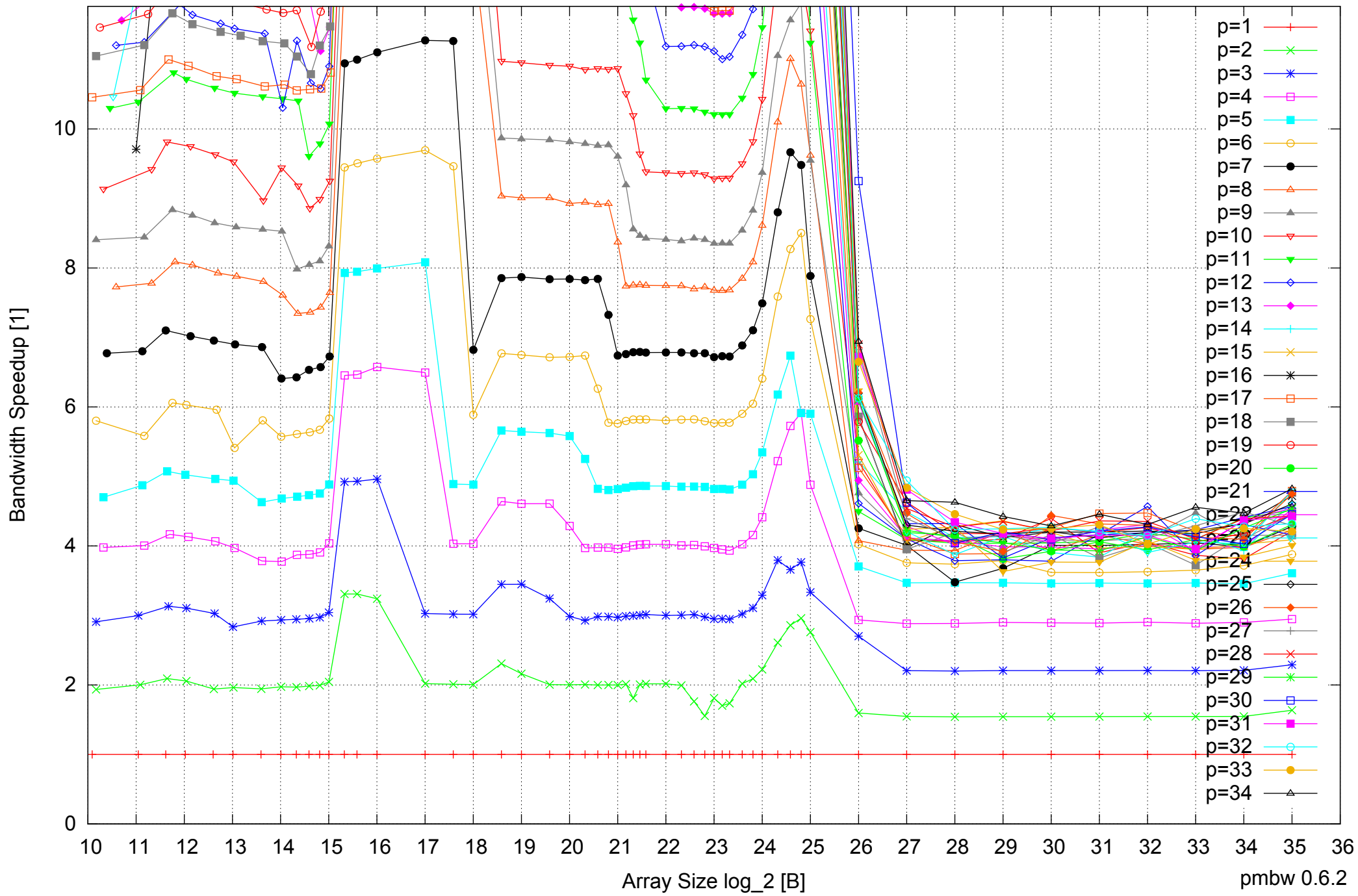
Intel Xeon E5-2670 64GB - Speedup of Parallel Memory Bandwidth (enlarged) - ScanRead32PtrUnrollLoop
