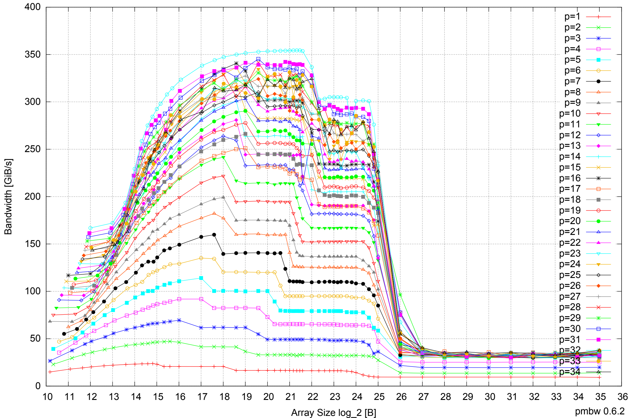
Intel Xeon E5-2670 64GB - Parallel Memory Bandwidth - ScanRead64PtrSimpleLoop
