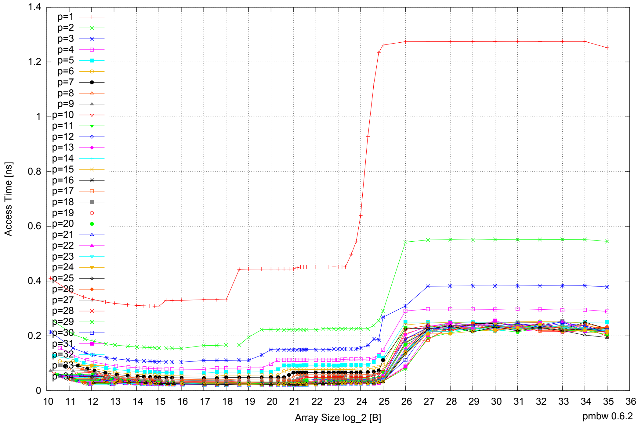
Intel Xeon E5-2670 64GB - Parallel Memory Access Time - ScanRead64IndexSimpleLoop
