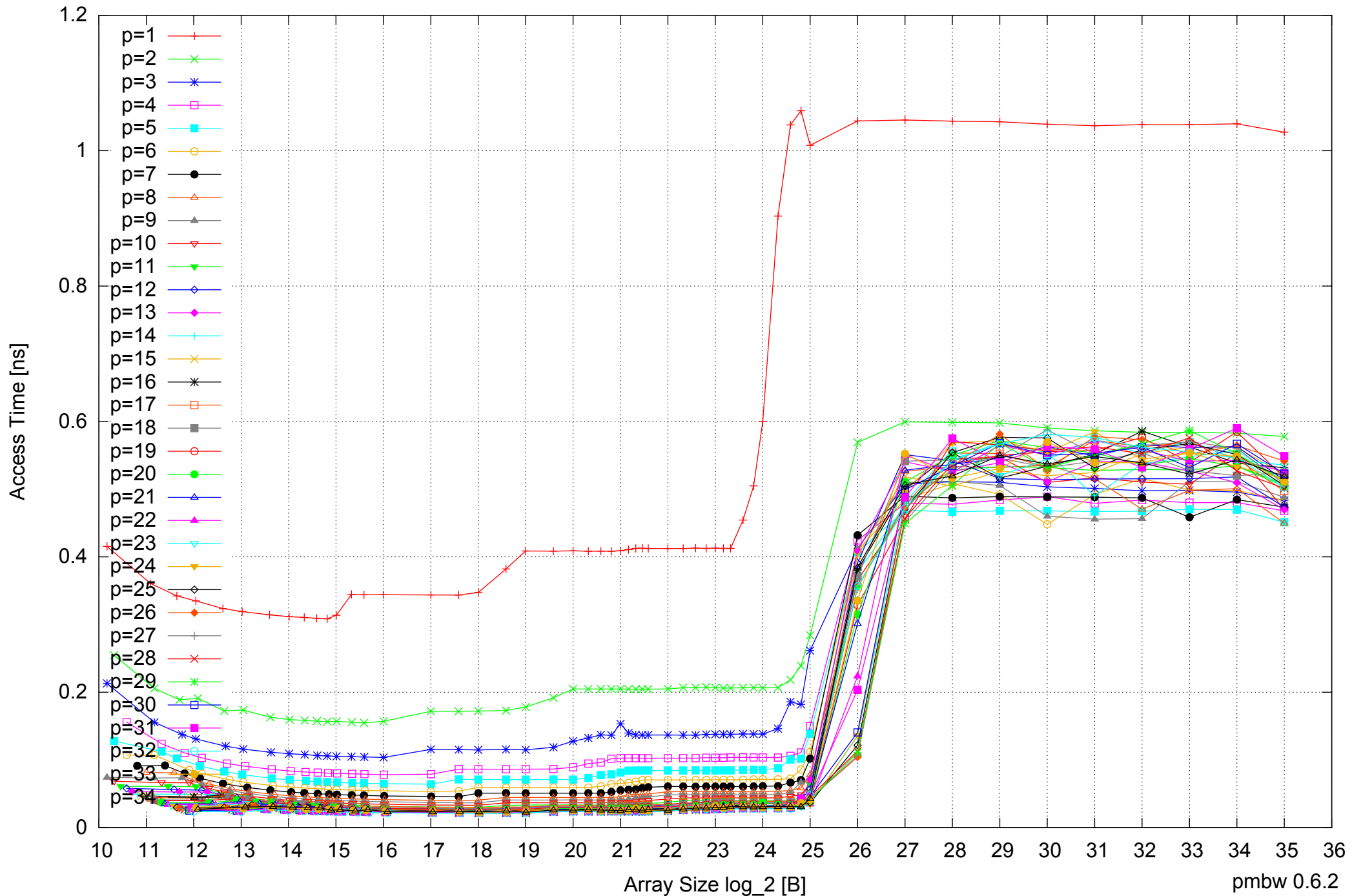
Intel Xeon E5-2670 64GB - Parallel Memory Access Time - ScanWrite64PtrSimpleLoop
