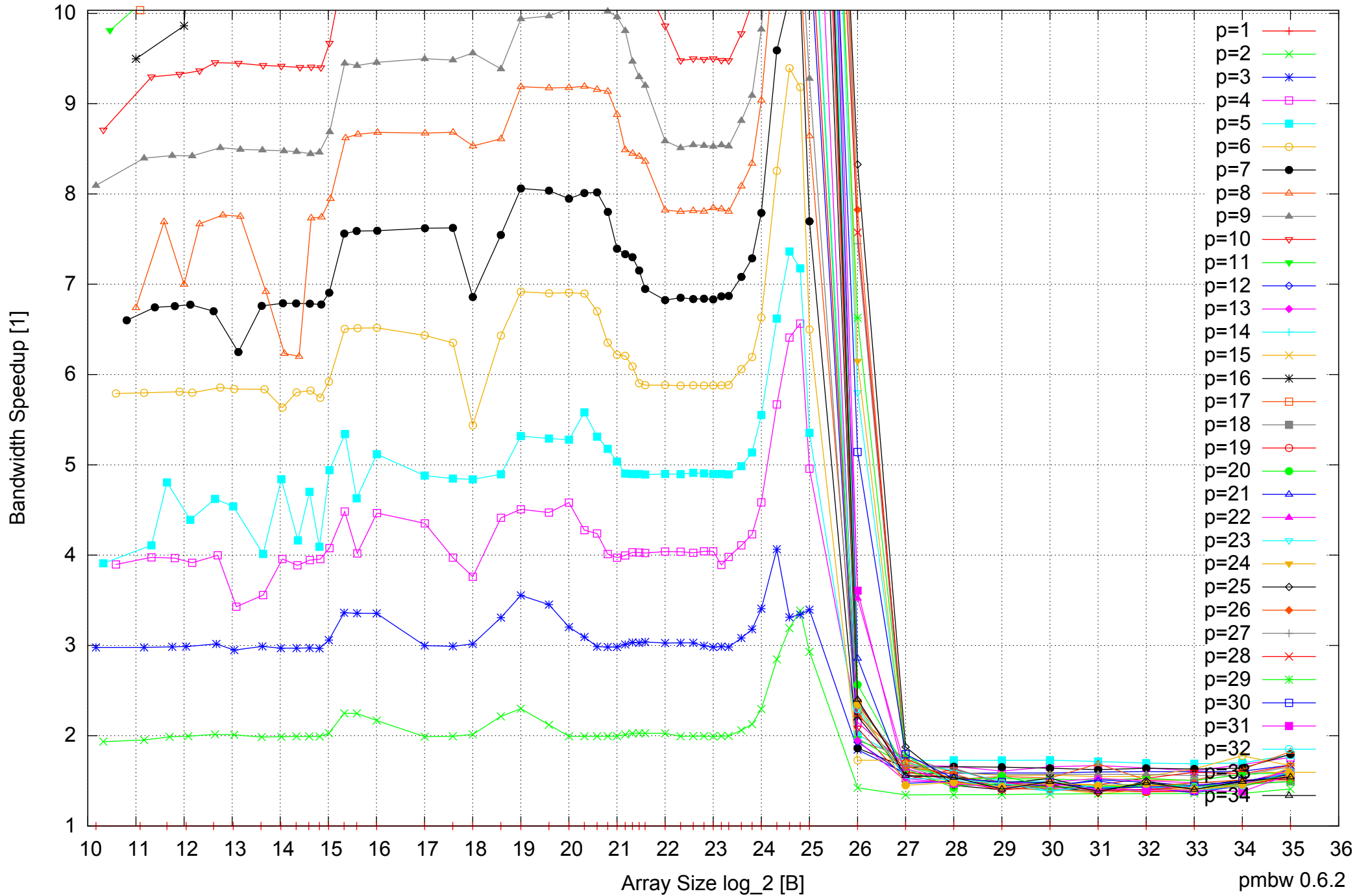
Intel Xeon E5-2670 64GB - Speedup of Parallel Memory Bandwidth (enlarged) - ScanWrite64PtrUnrollLoop
