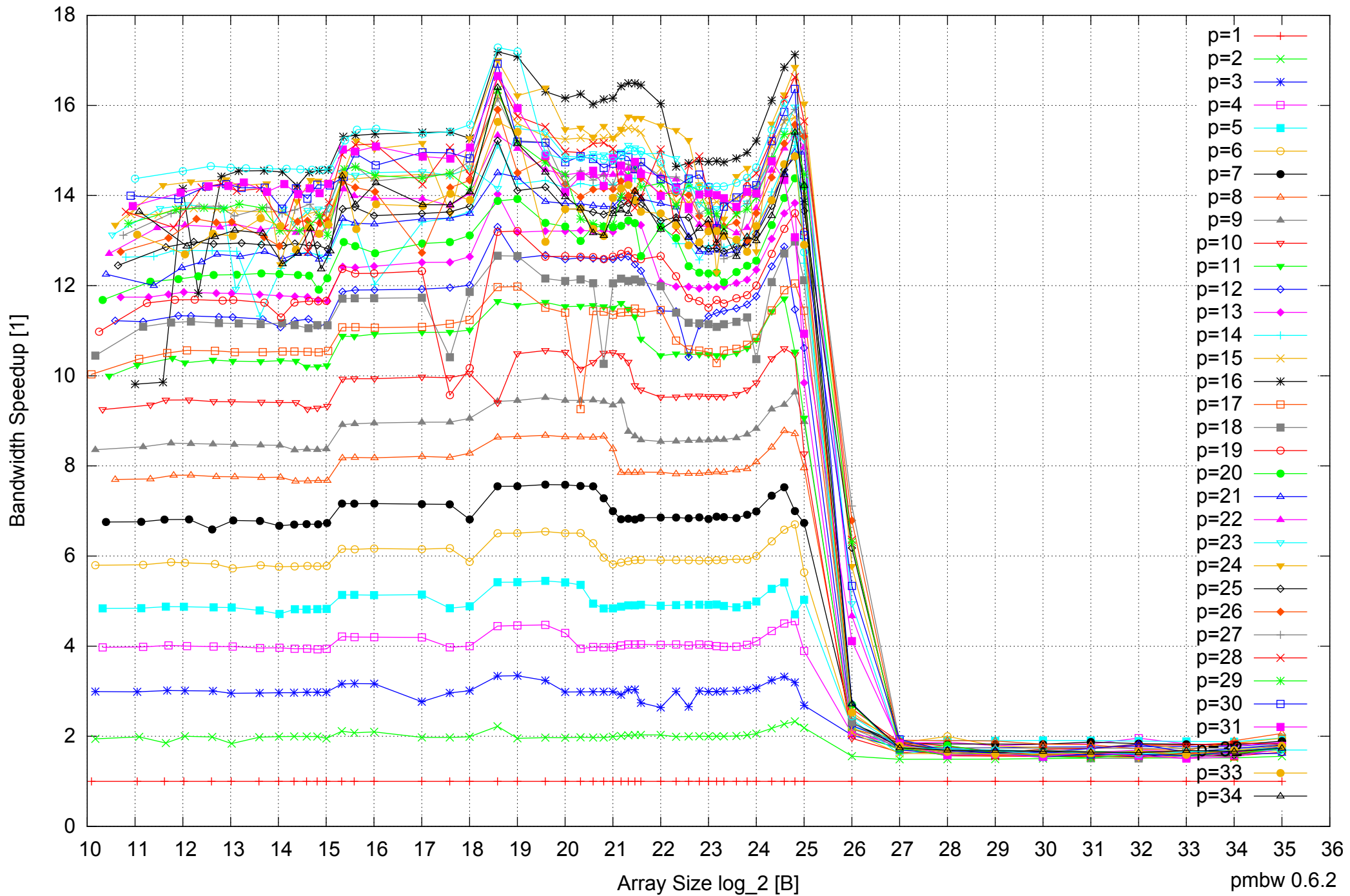
Intel Xeon E5-2670 64GB - Speedup of Parallel Memory Bandwidth - ScanWrite32PtrUnrollLoop
