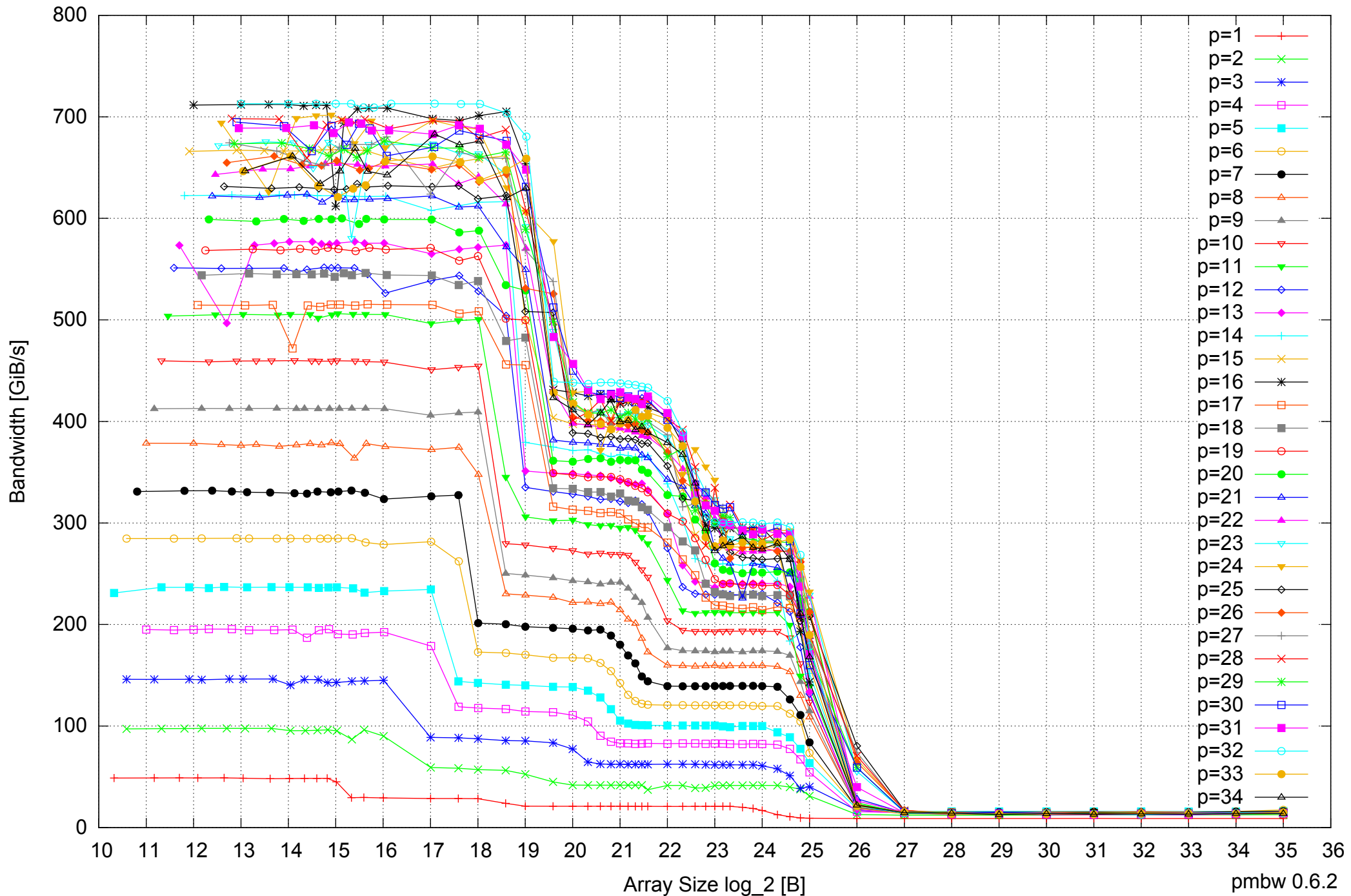
Intel Xeon E5-2670 64GB - Parallel Memory Bandwidth - ScanWrite128PtrUnrollLoop
