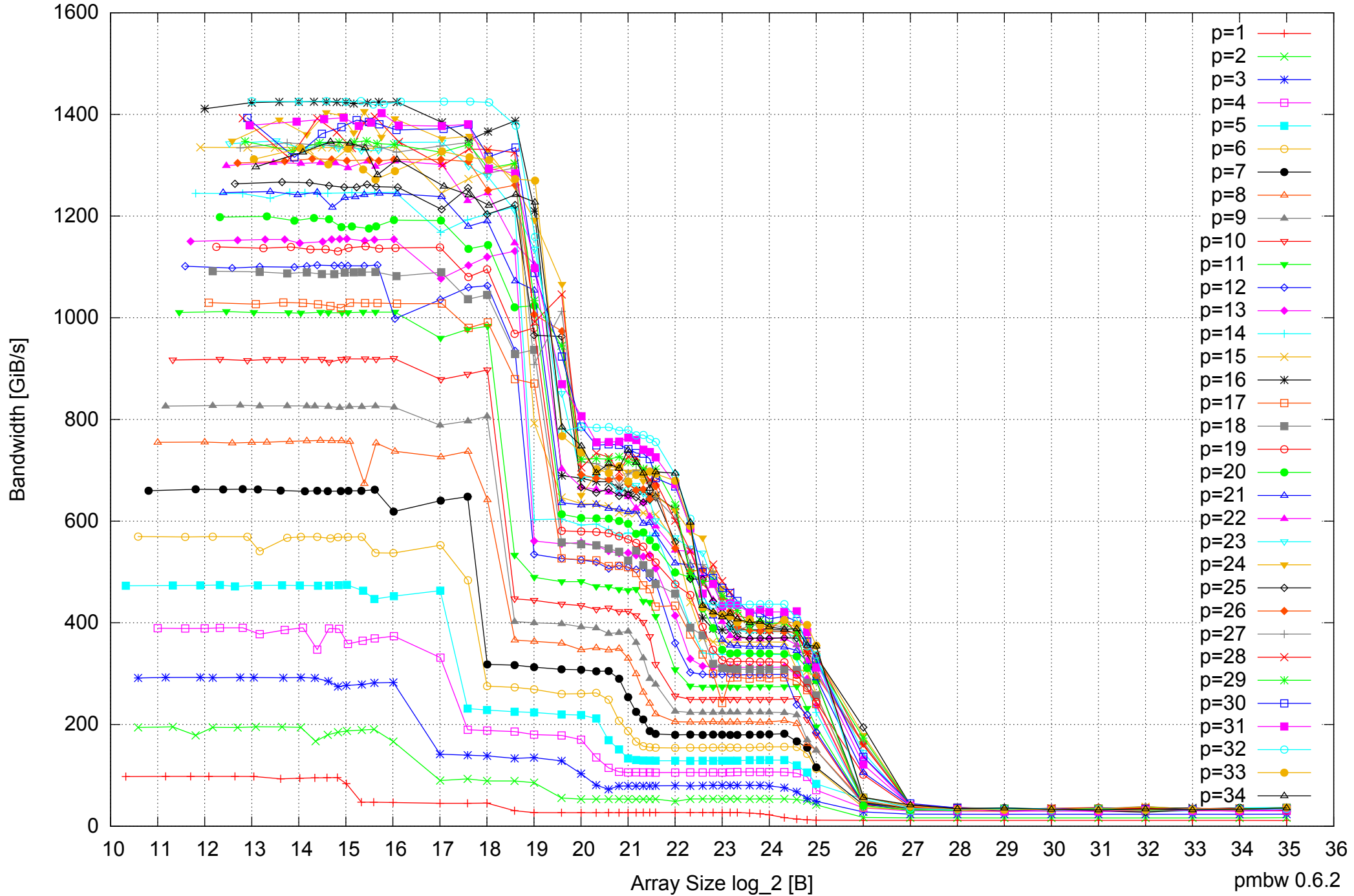
Intel Xeon E5-2670 64GB - Parallel Memory Bandwidth - ScanRead128PtrUnrollLoop
