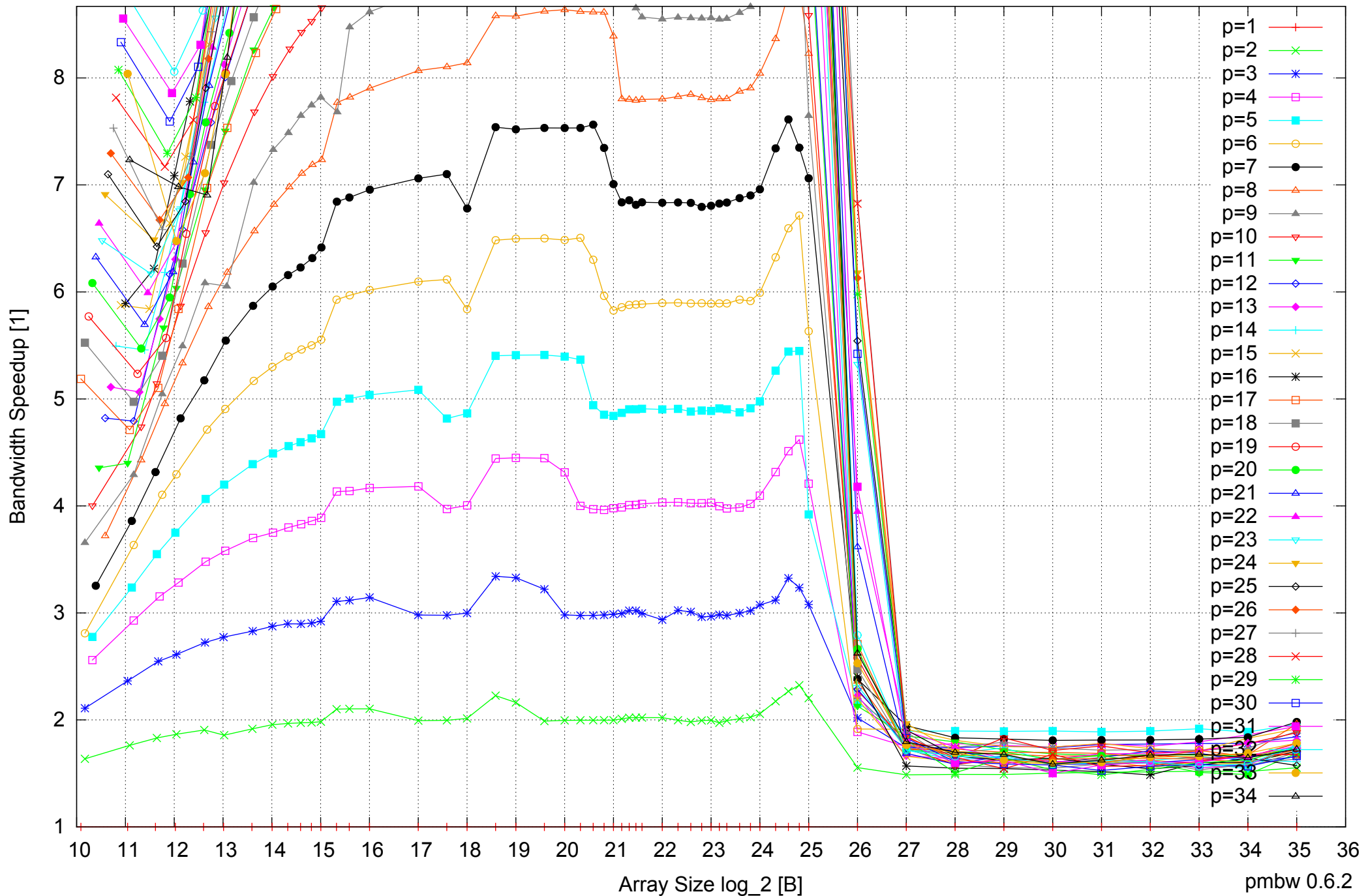
Intel Xeon E5-2670 64GB - Speedup of Parallel Memory Bandwidth (enlarged) - ScanWrite32PtrSimpleLoop
