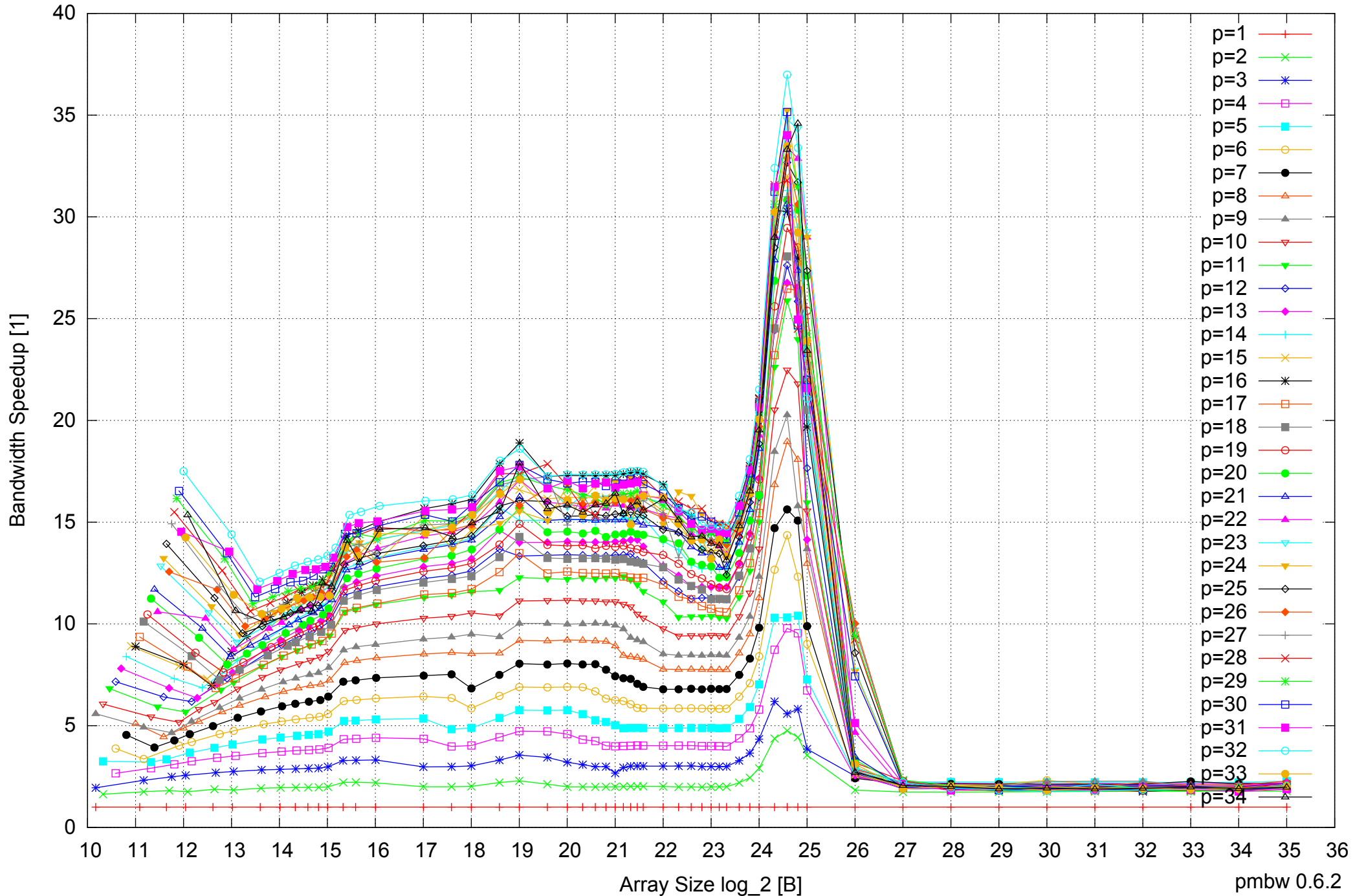
Intel Xeon E5-2670 64GB - Speedup of Parallel Memory Bandwidth - ScanWrite64PtrSimpleLoop
