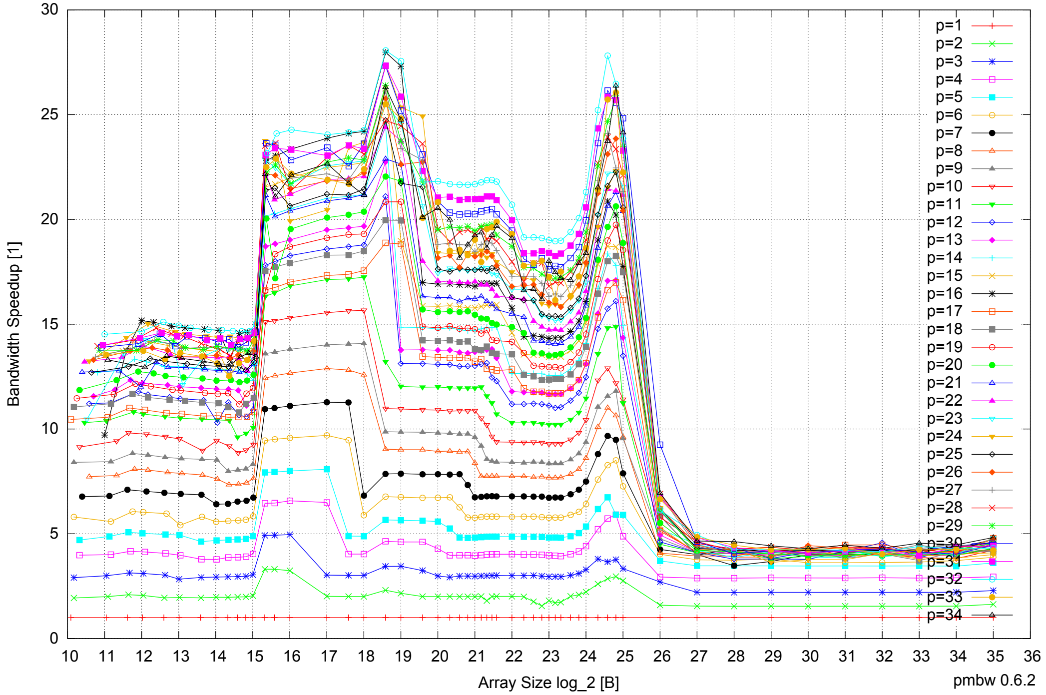
Intel Xeon E5-2670 64GB - Speedup of Parallel Memory Bandwidth - ScanRead32PtrUnrollLoop
