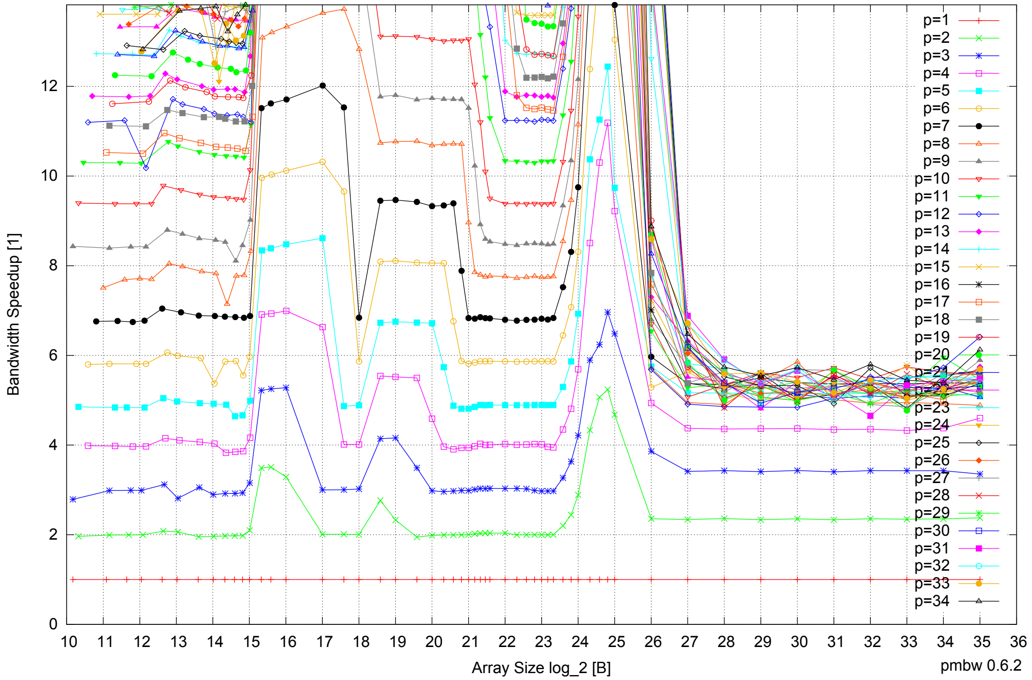
Intel Xeon E5-2670 64GB - Speedup of Parallel Memory Bandwidth (enlarged) - ScanRead64IndexUnrollLoop
