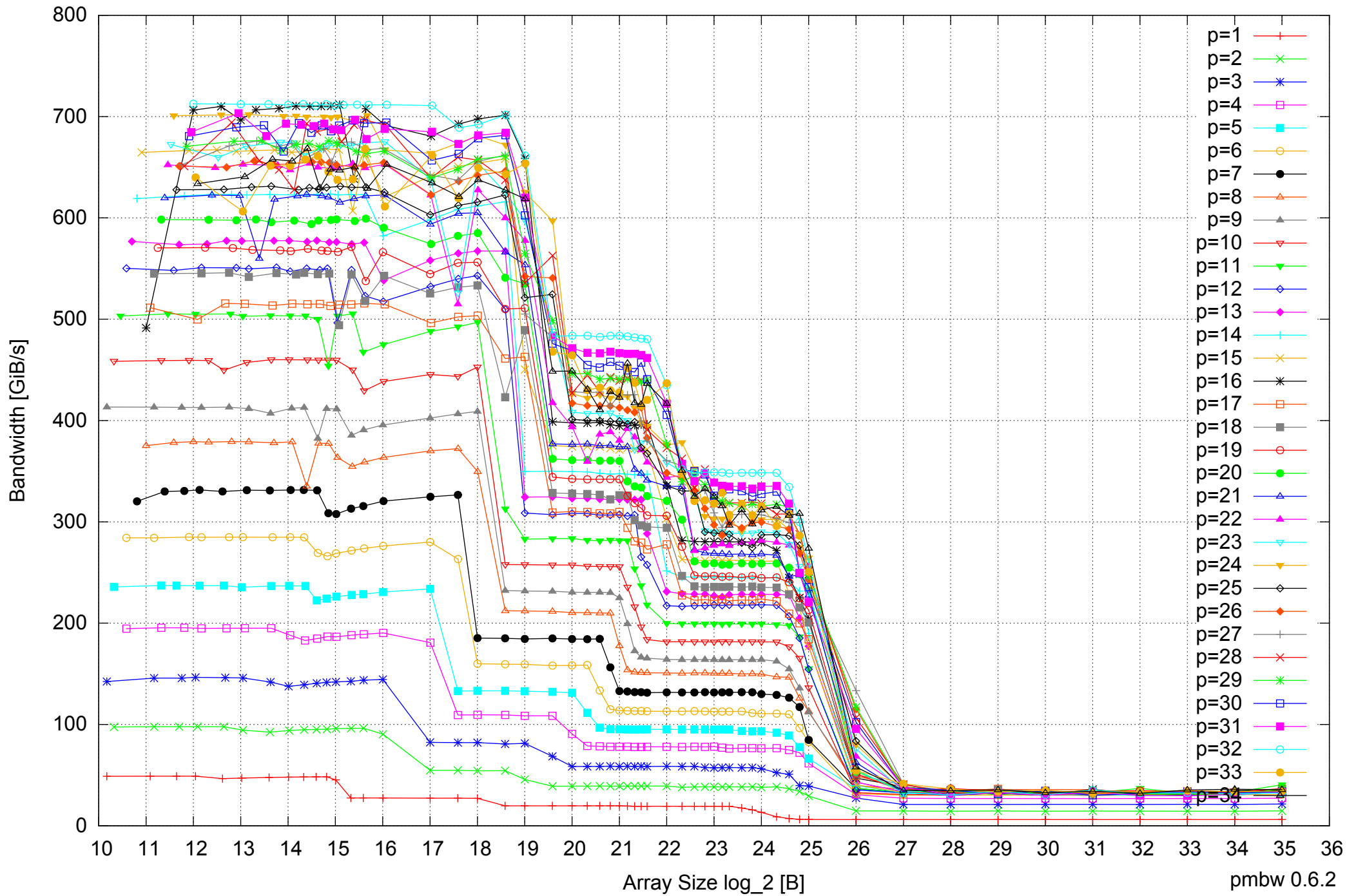
Intel Xeon E5-2670 64GB - Parallel Memory Bandwidth - ScanRead64PtrUnrollLoop
