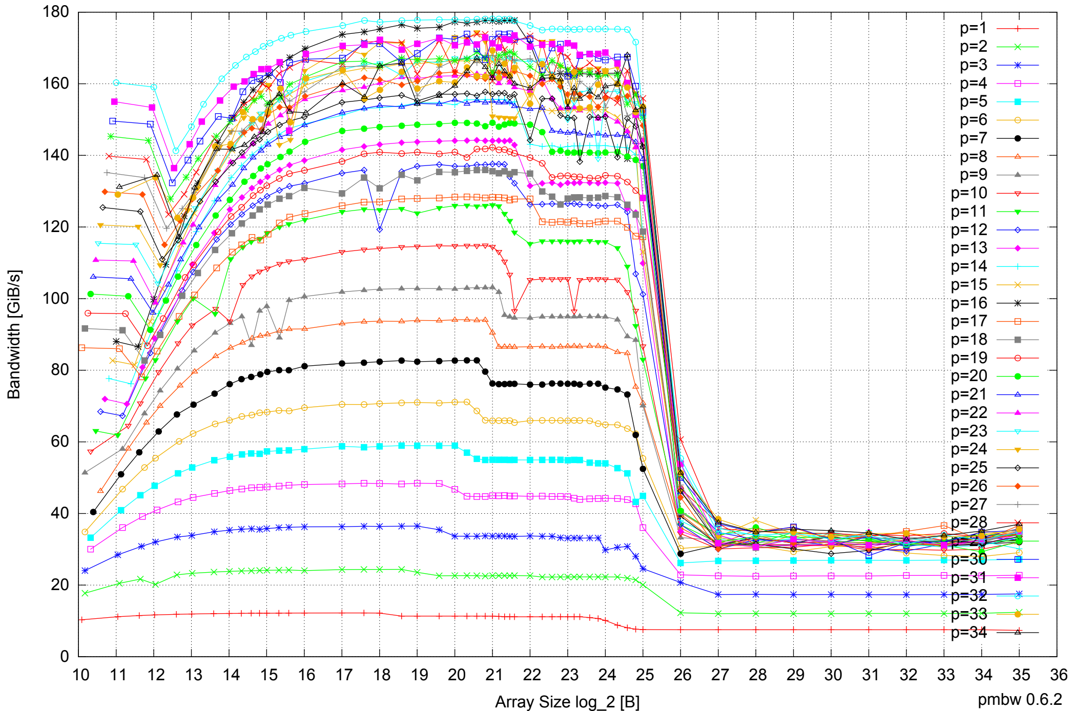
Intel Xeon E5-2670 64GB - Parallel Memory Bandwidth - ScanRead32PtrSimpleLoop
