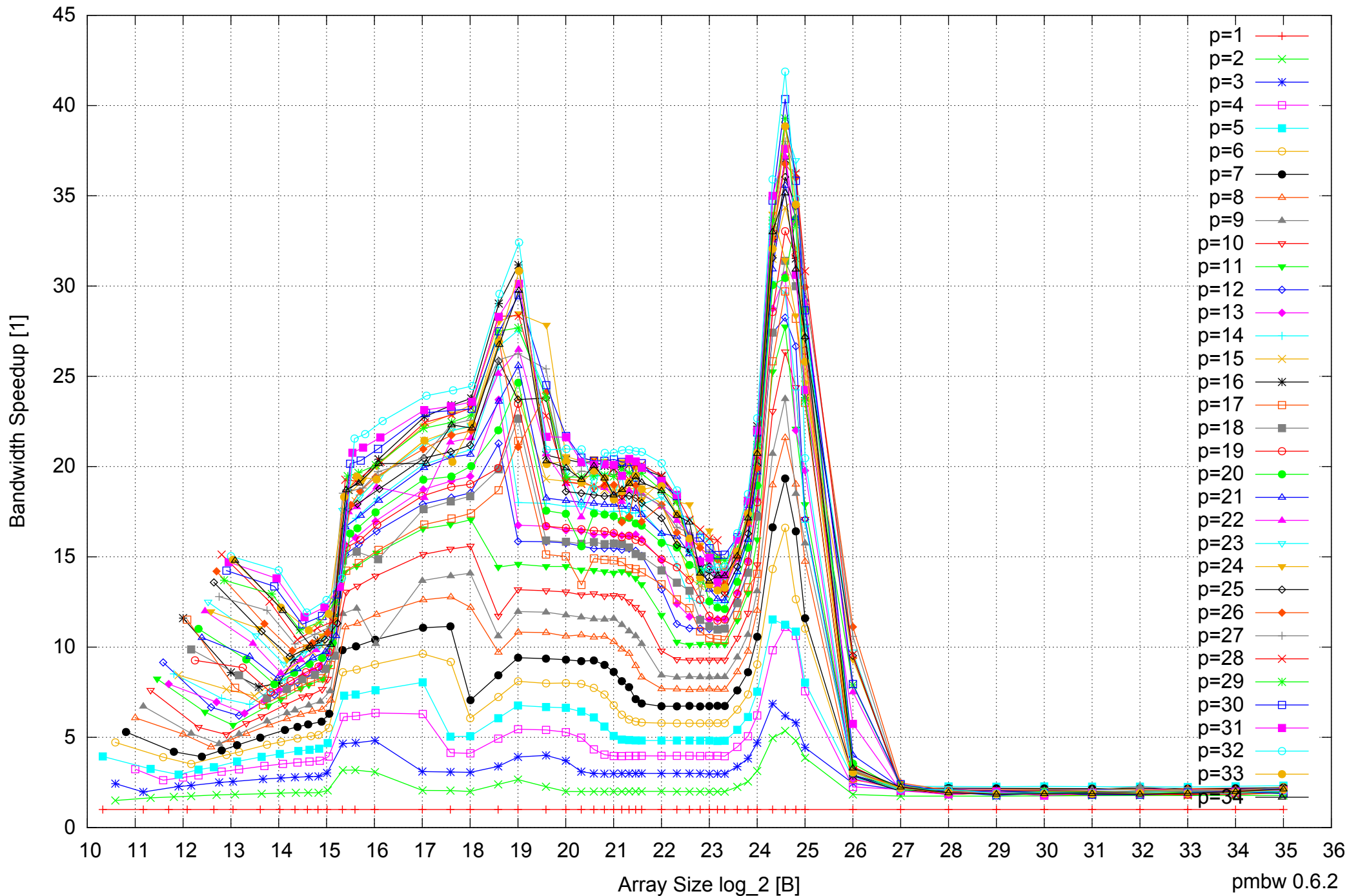
Intel Xeon E5-2670 64GB - Speedup of Parallel Memory Bandwidth - ScanWrite128PtrSimpleLoop
