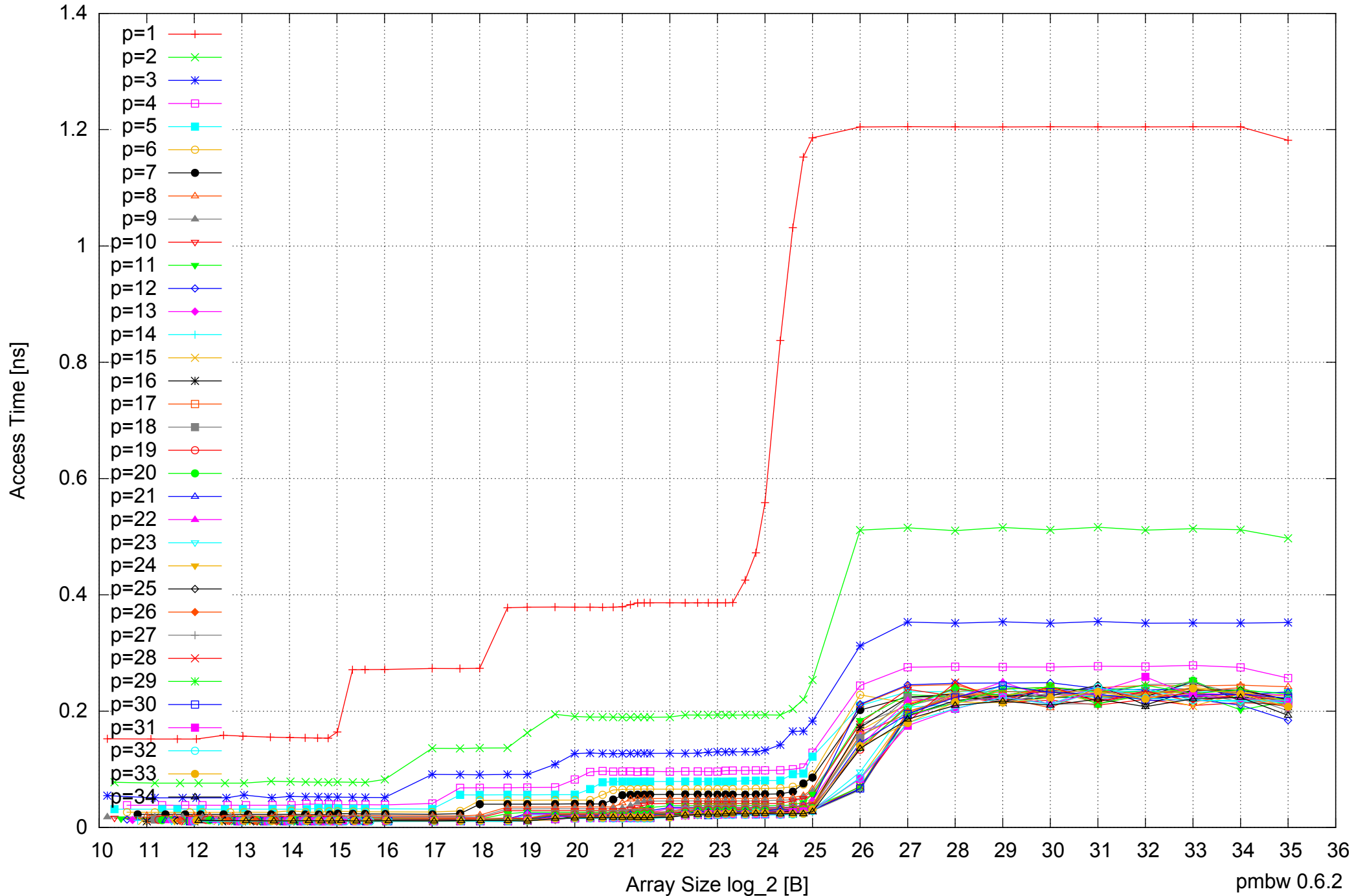
Intel Xeon E5-2670 64GB - Parallel Memory Access Time - ScanRead64IndexUnrollLoop
