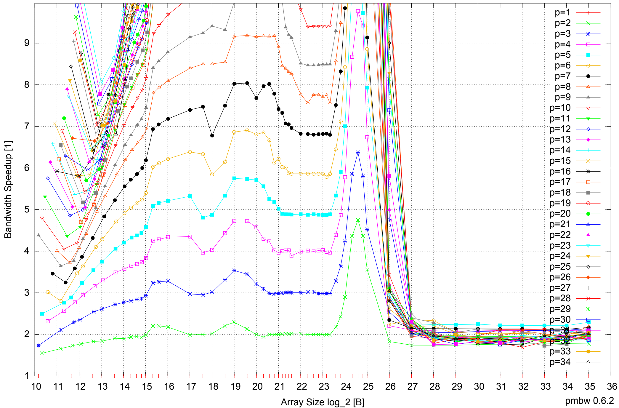
Intel Xeon E5-2670 64GB - Speedup of Parallel Memory Bandwidth (enlarged) - ScanWrite64IndexSimpleLoop
