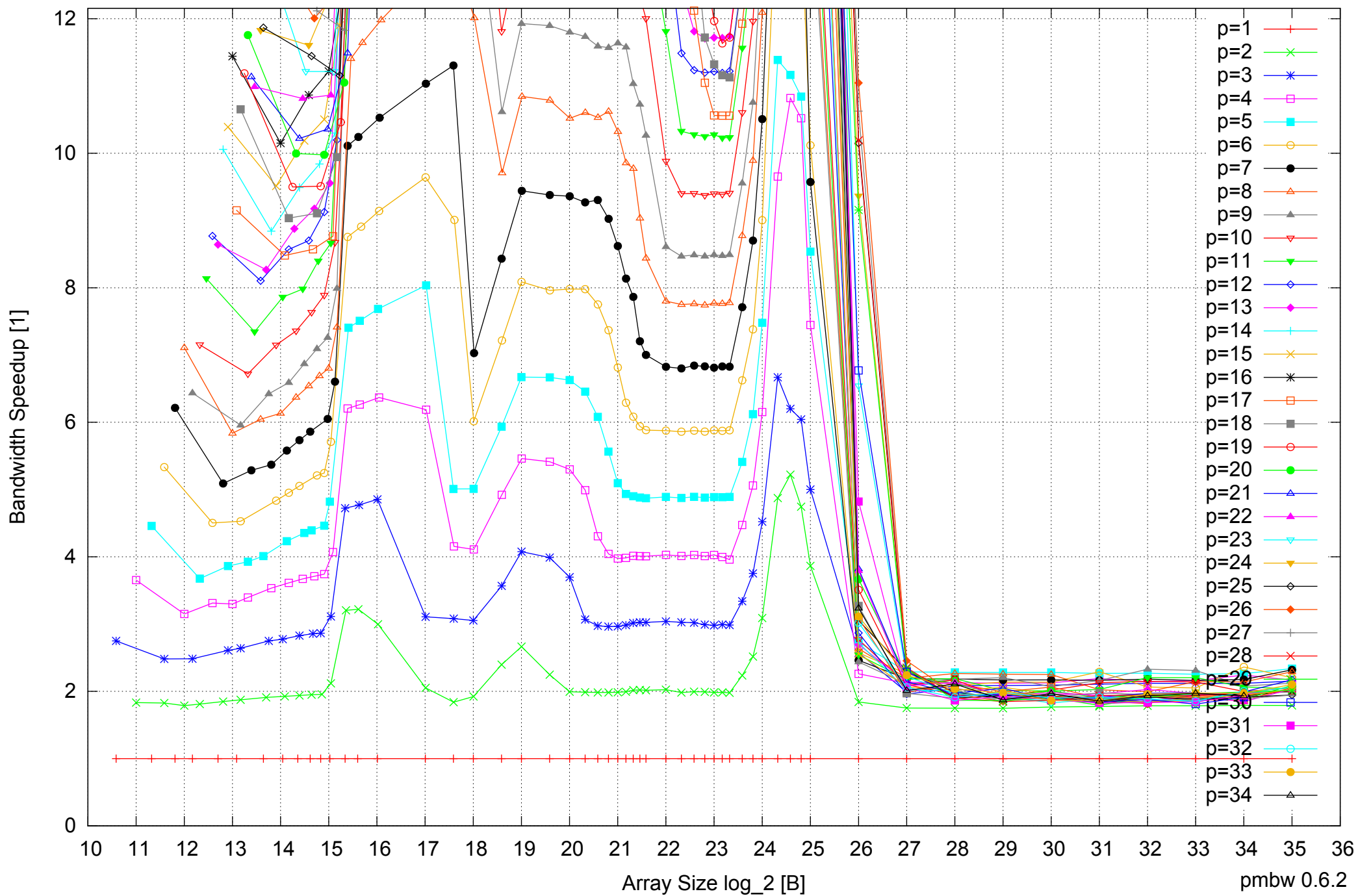
Intel Xeon E5-2670 64GB - Speedup of Parallel Memory Bandwidth (enlarged) - ScanWrite256PtrSimpleLoop
