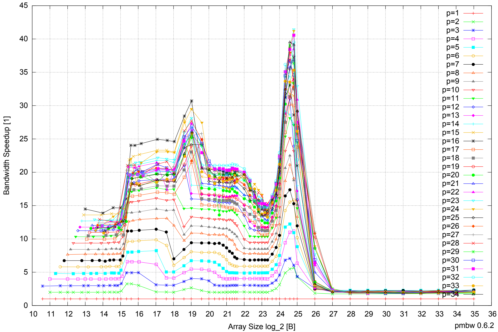
Intel Xeon E5-2670 64GB - Speedup of Parallel Memory Bandwidth - ScanWrite256PtrUnrollLoop
