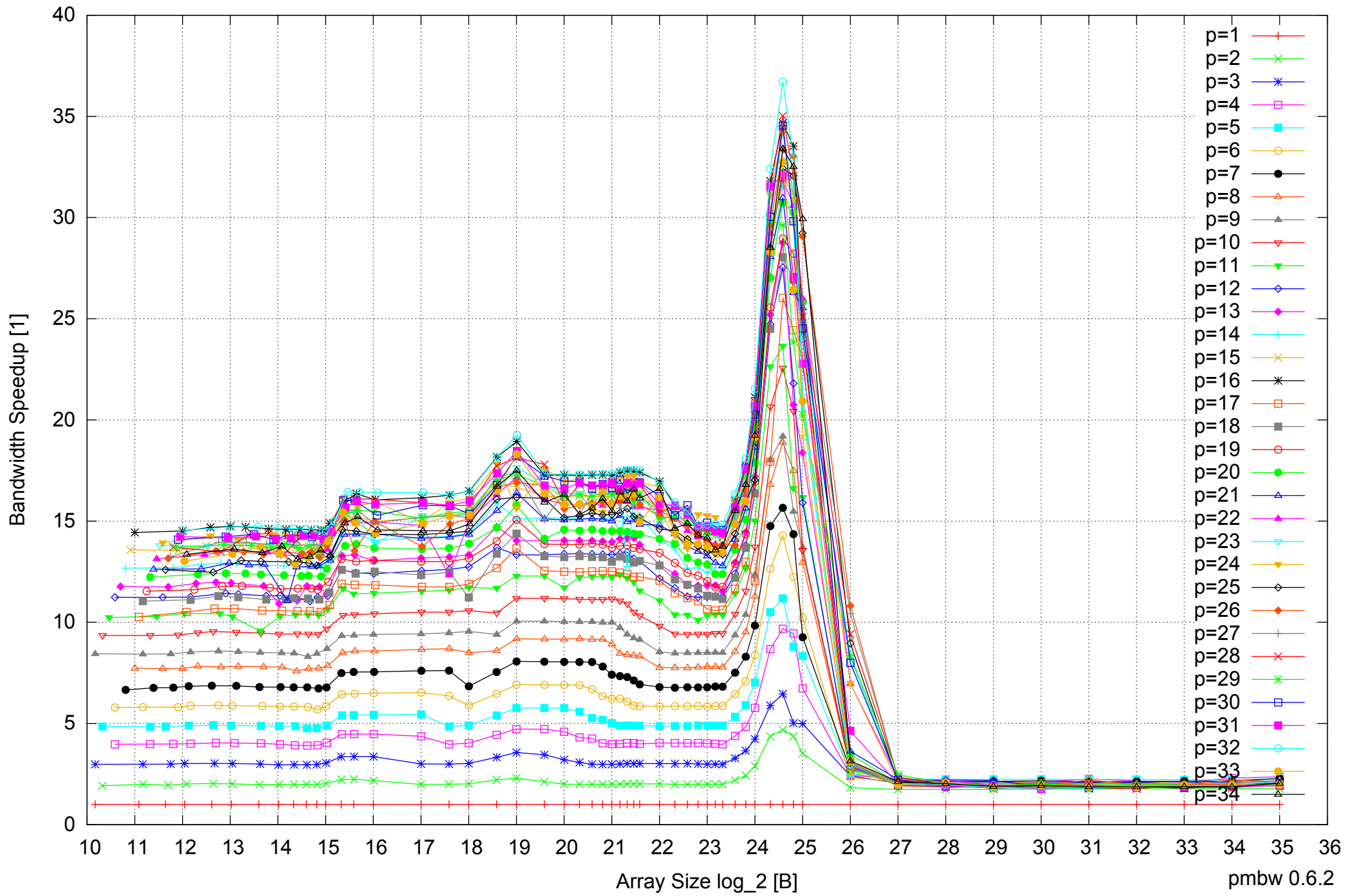
Intel Xeon E5-2670 64GB - Speedup of Parallel Memory Bandwidth - ScanWrite64IndexUnrollLoop
