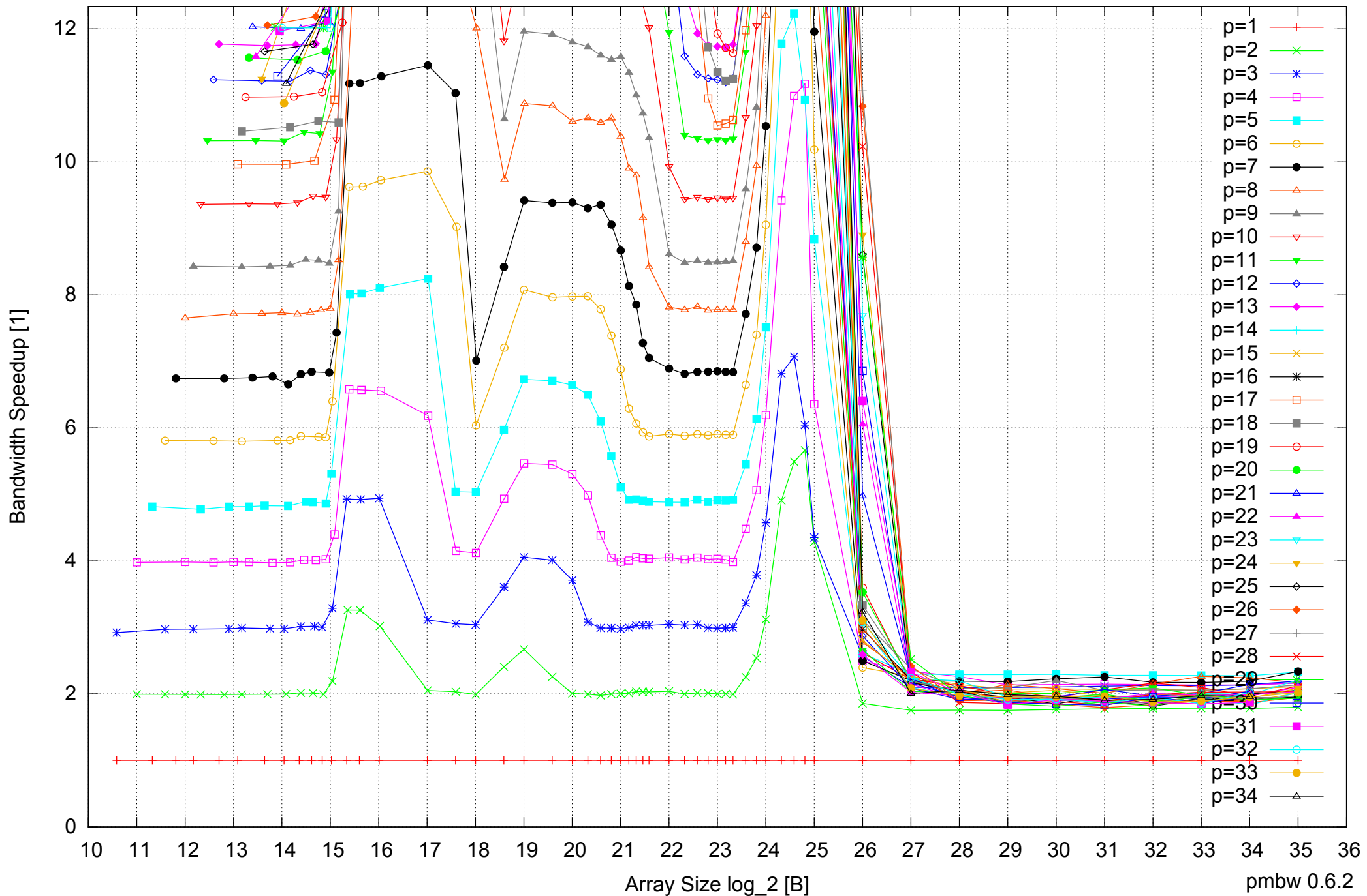
Intel Xeon E5-2670 64GB - Speedup of Parallel Memory Bandwidth (enlarged) - ScanWrite256PtrUnrollLoop
