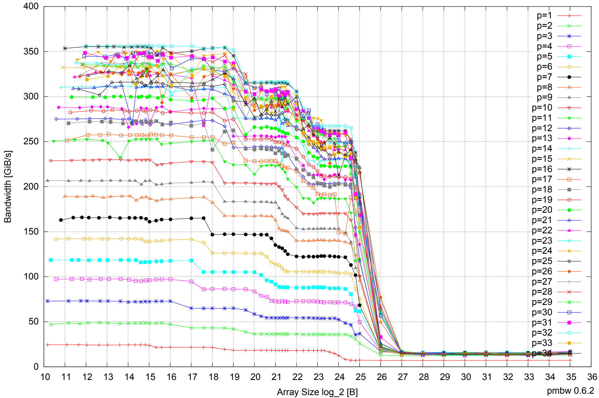
Intel Xeon E5-2670 64GB - Parallel Memory Bandwidth - ScanWrite64IndexUnrollLoop
