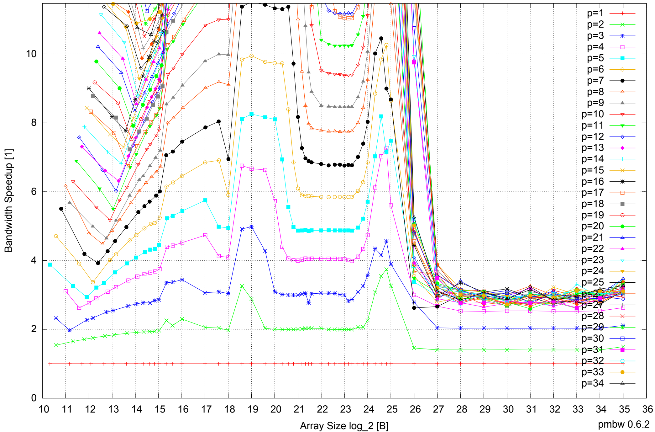
Intel Xeon E5-2670 64GB - Speedup of Parallel Memory Bandwidth (enlarged) - ScanRead128PtrSimpleLoop
