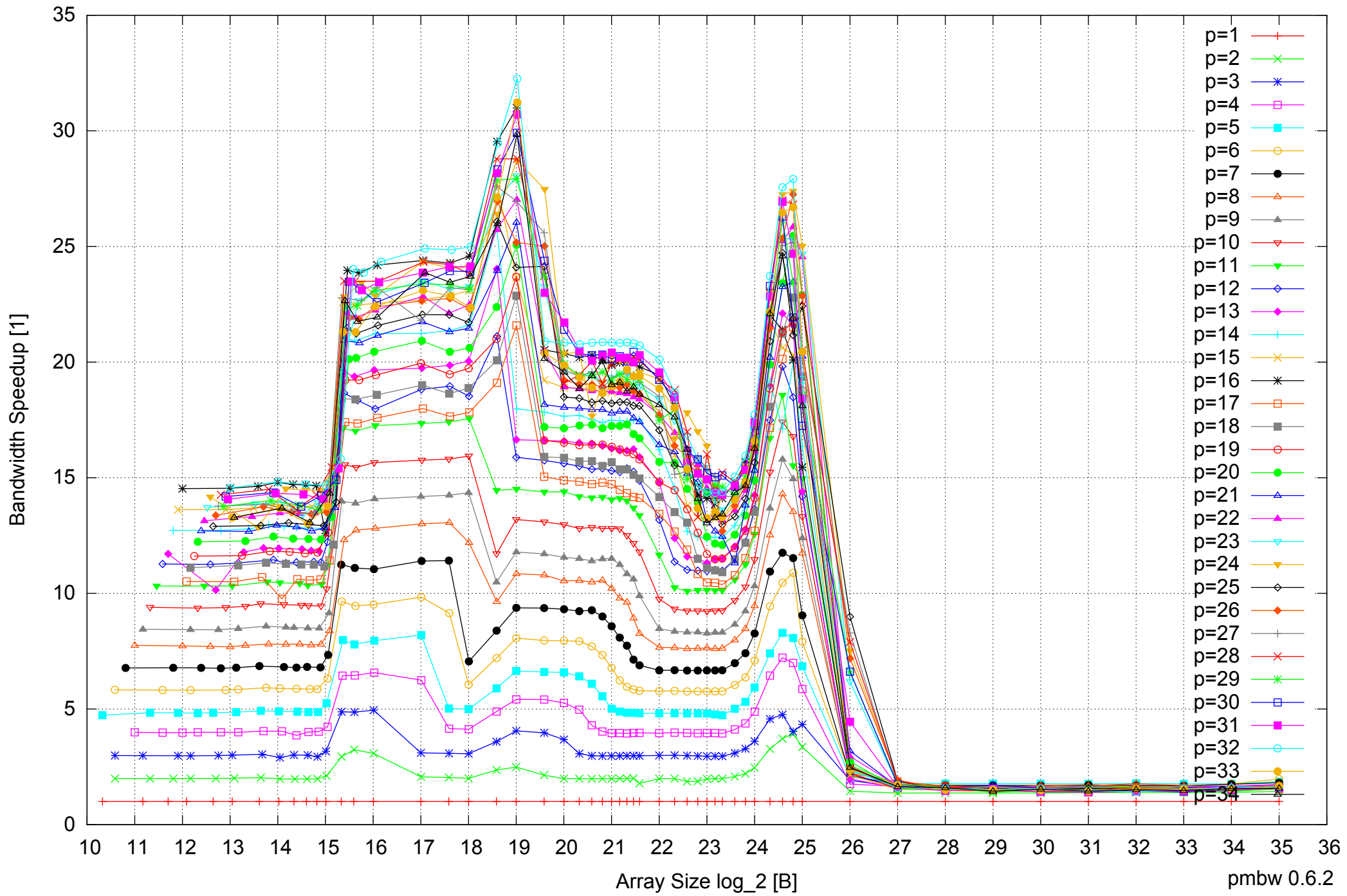
Intel Xeon E5-2670 64GB - Speedup of Parallel Memory Bandwidth - ScanWrite128PtrUnrollLoop
