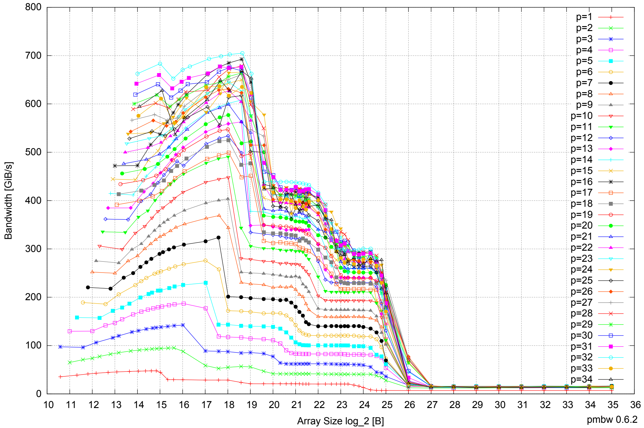
Intel Xeon E5-2670 64GB - Parallel Memory Bandwidth - ScanWrite256PtrSimpleLoop
