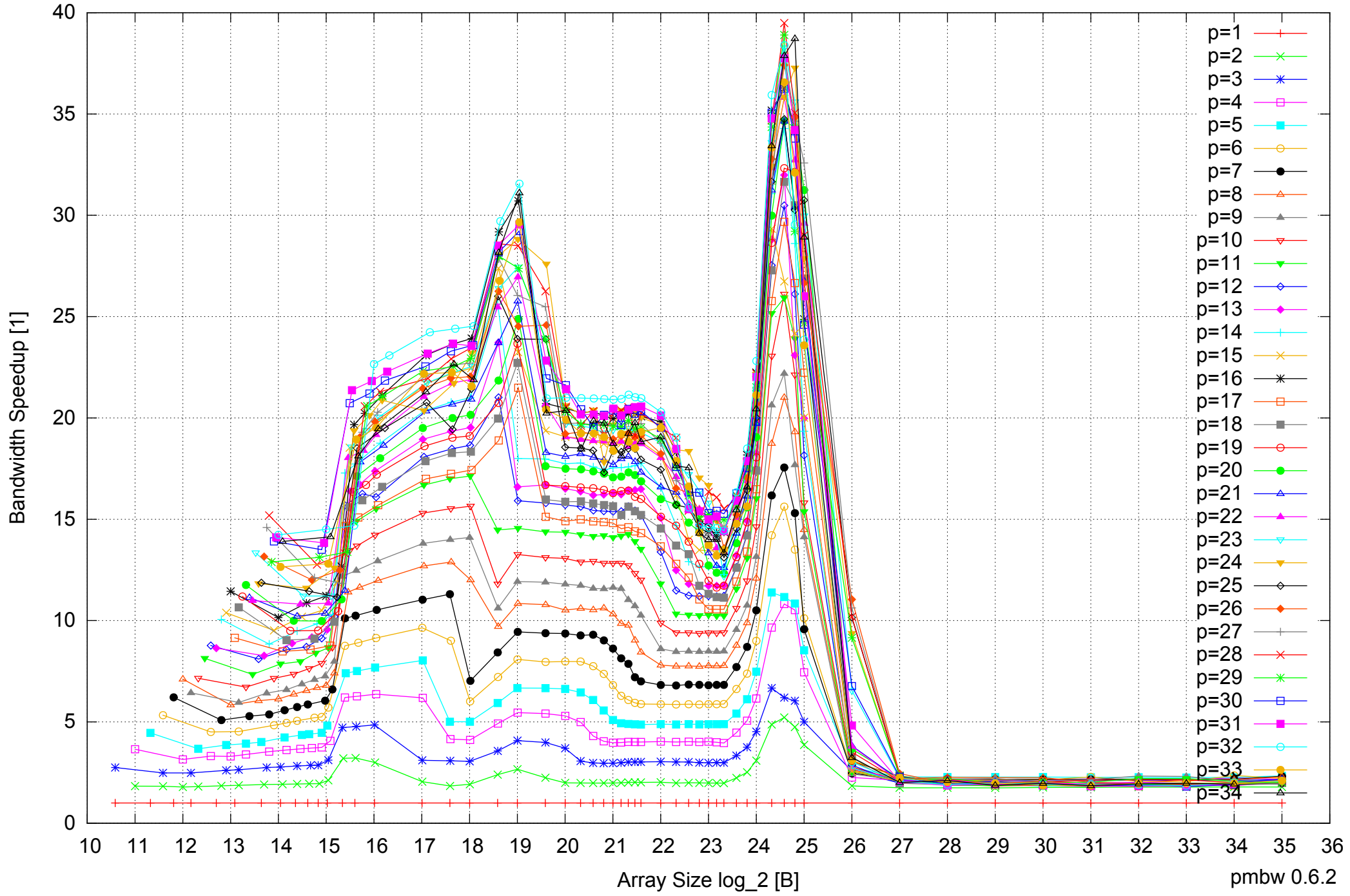
Intel Xeon E5-2670 64GB - Speedup of Parallel Memory Bandwidth - ScanWrite256PtrSimpleLoop
