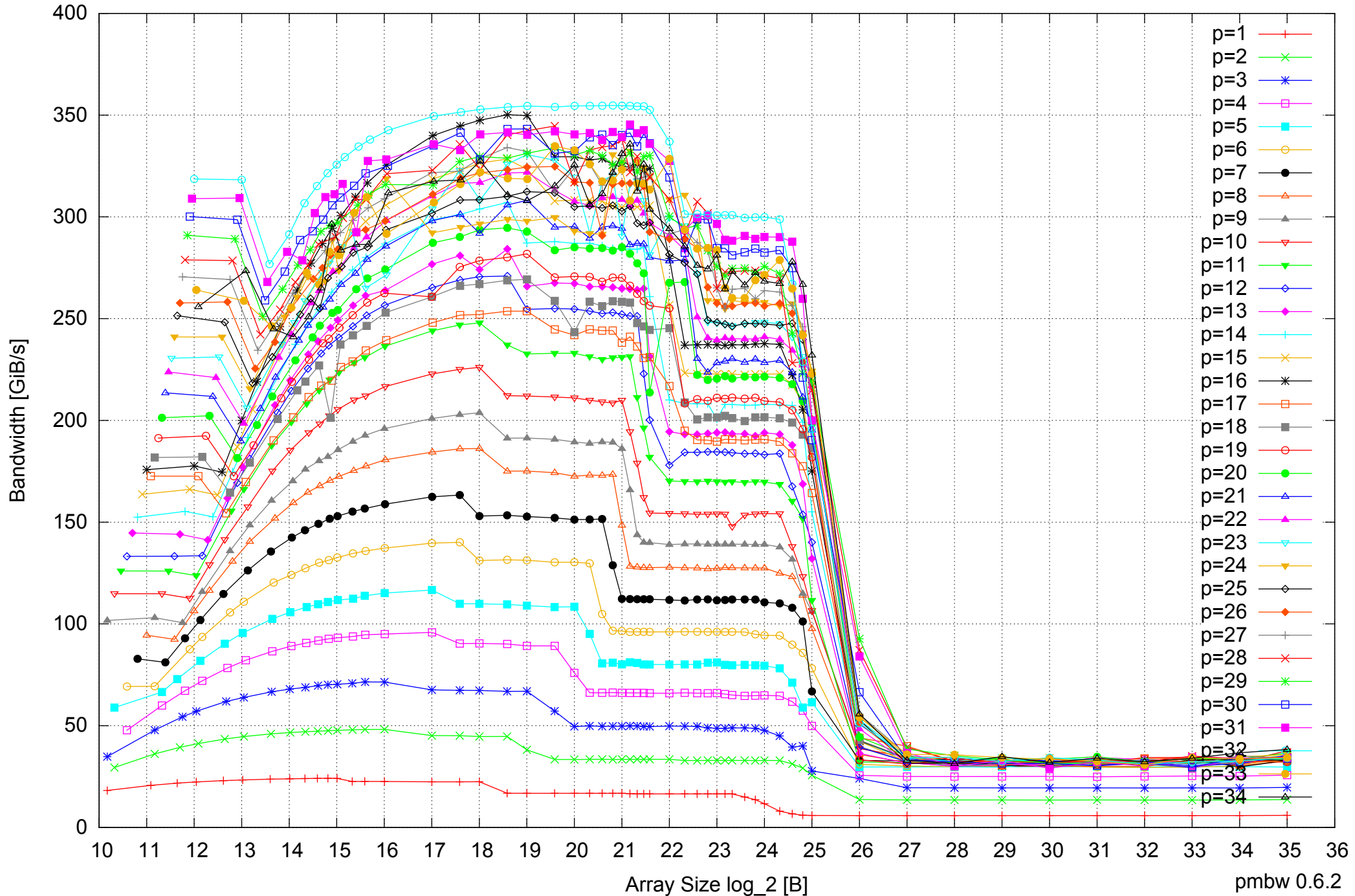
Intel Xeon E5-2670 64GB - Parallel Memory Bandwidth - ScanRead64IndexSimpleLoop
