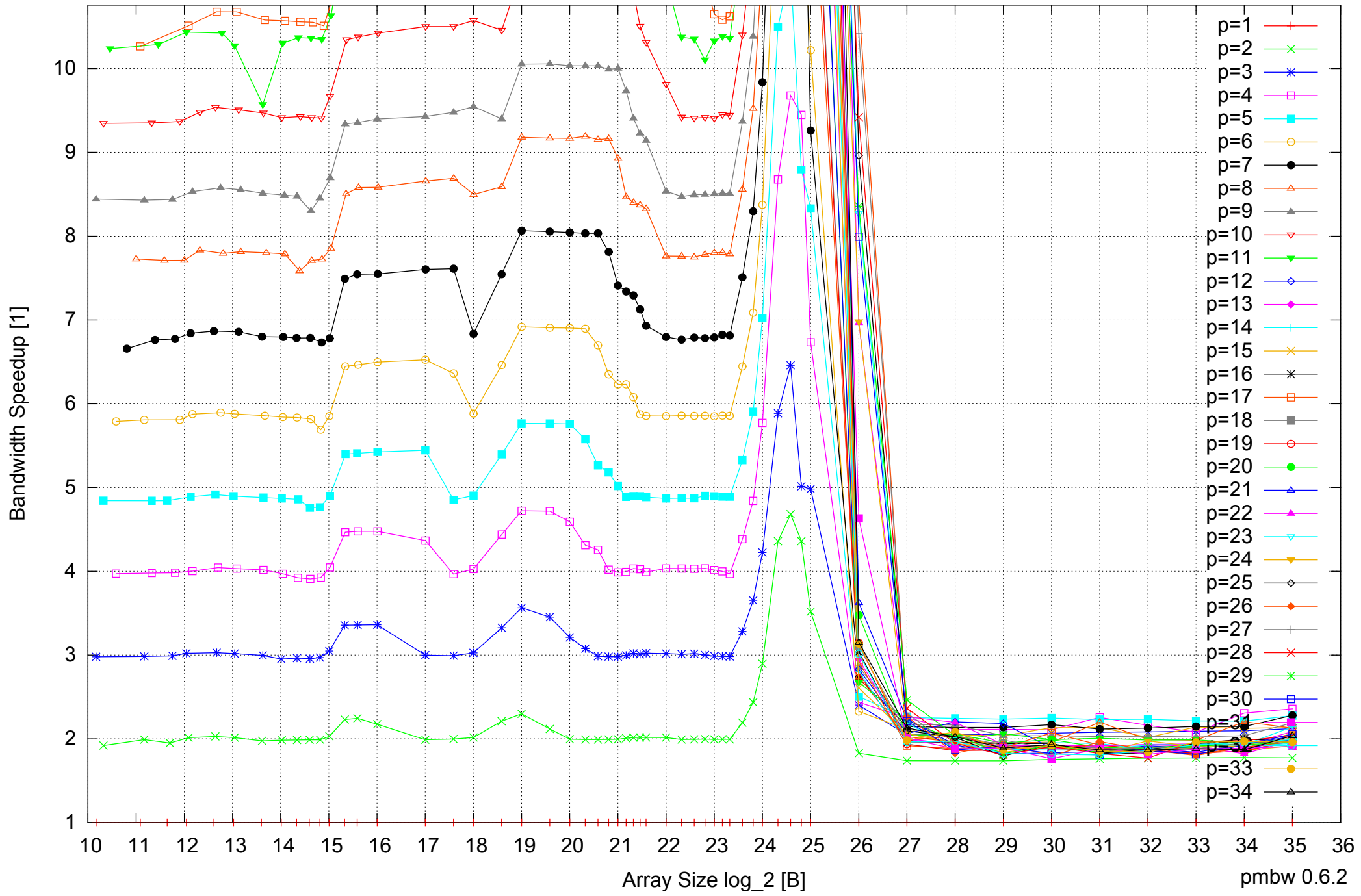
Intel Xeon E5-2670 64GB - Speedup of Parallel Memory Bandwidth (enlarged) - ScanWrite64IndexUnrollLoop
