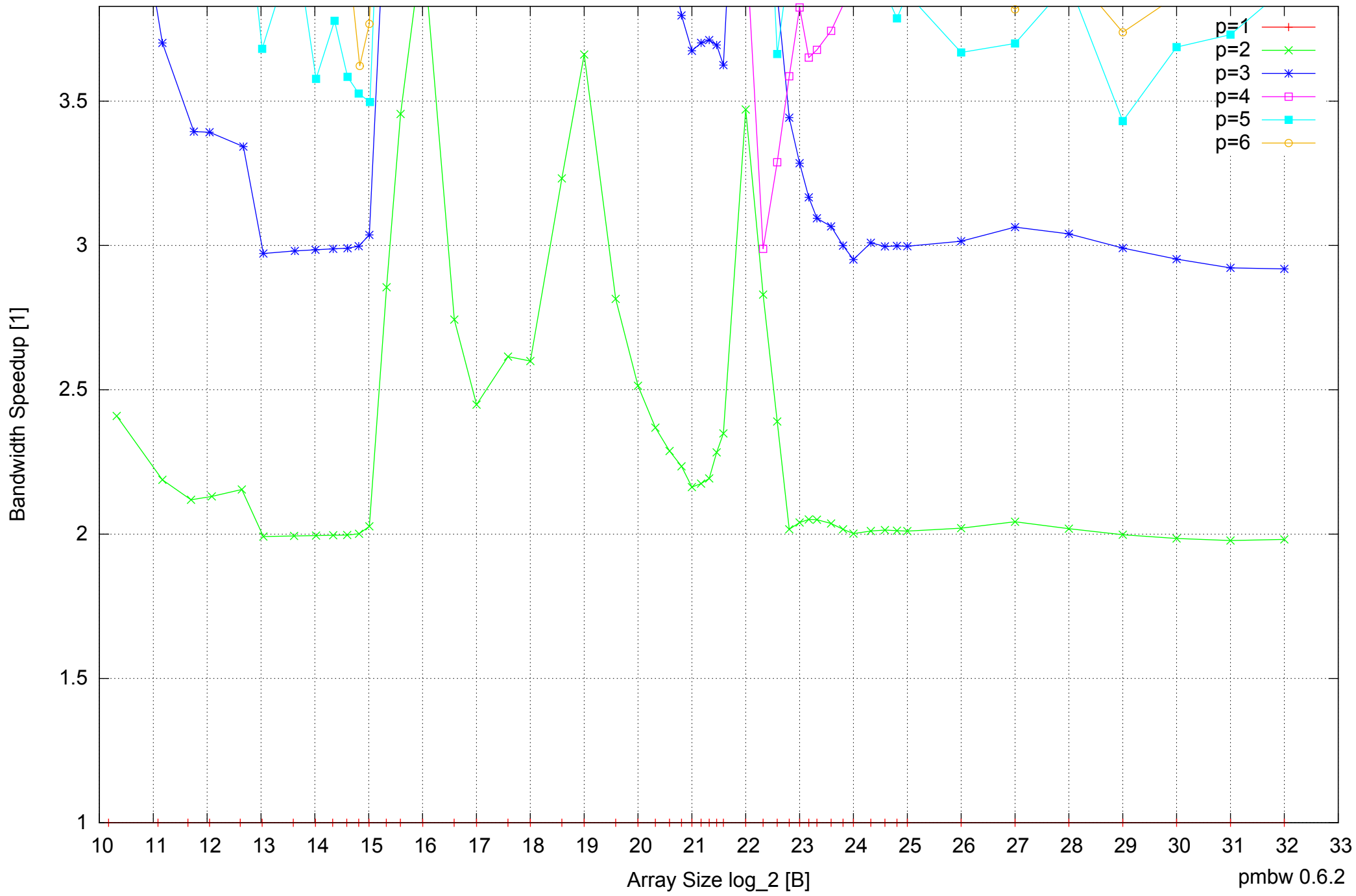
Intel Core i5-2500 8GB - Speedup of Parallel Memory Bandwidth (enlarged) - PermRead64UnrollLoop
