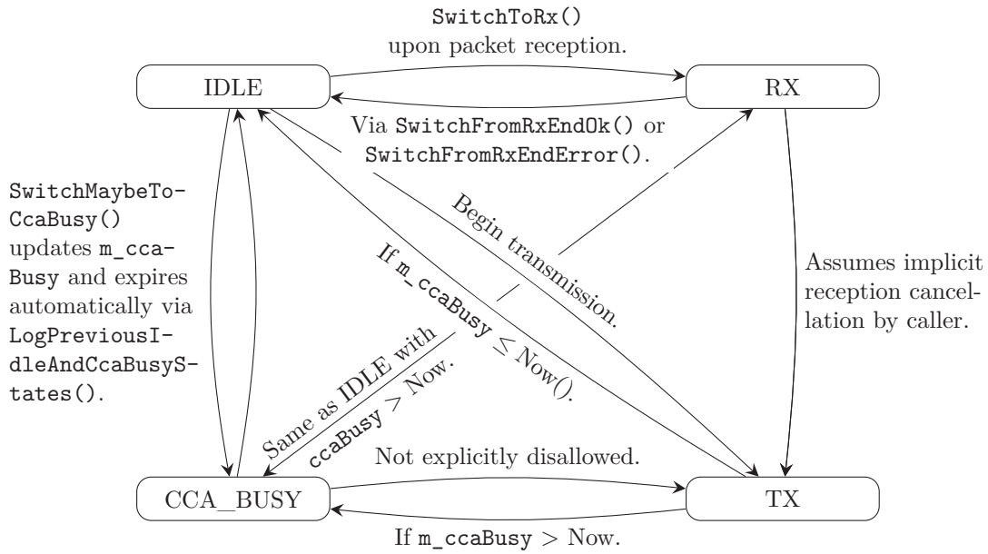
Figure 6.6: State transitions of WifiStateHelper
