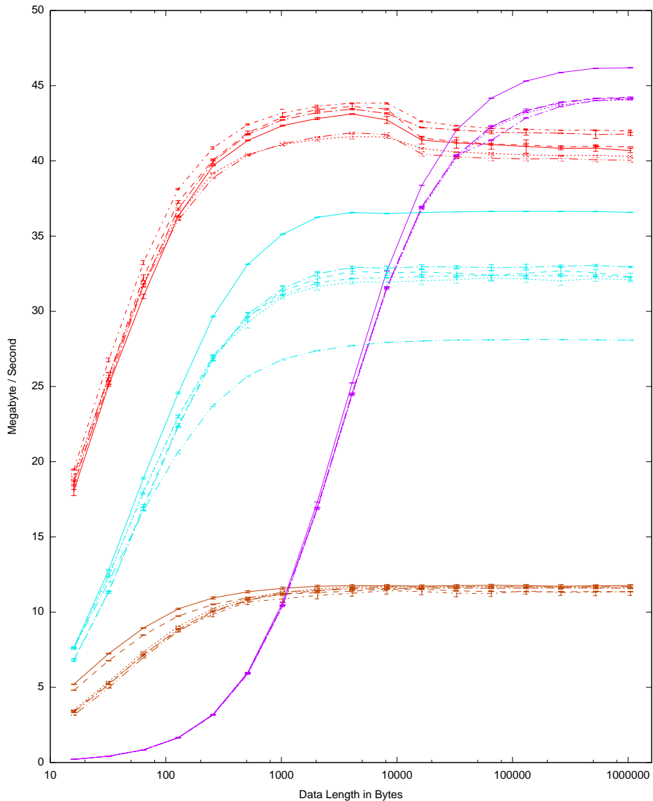
OpenSSL Ciphers: Speed by Data Length
