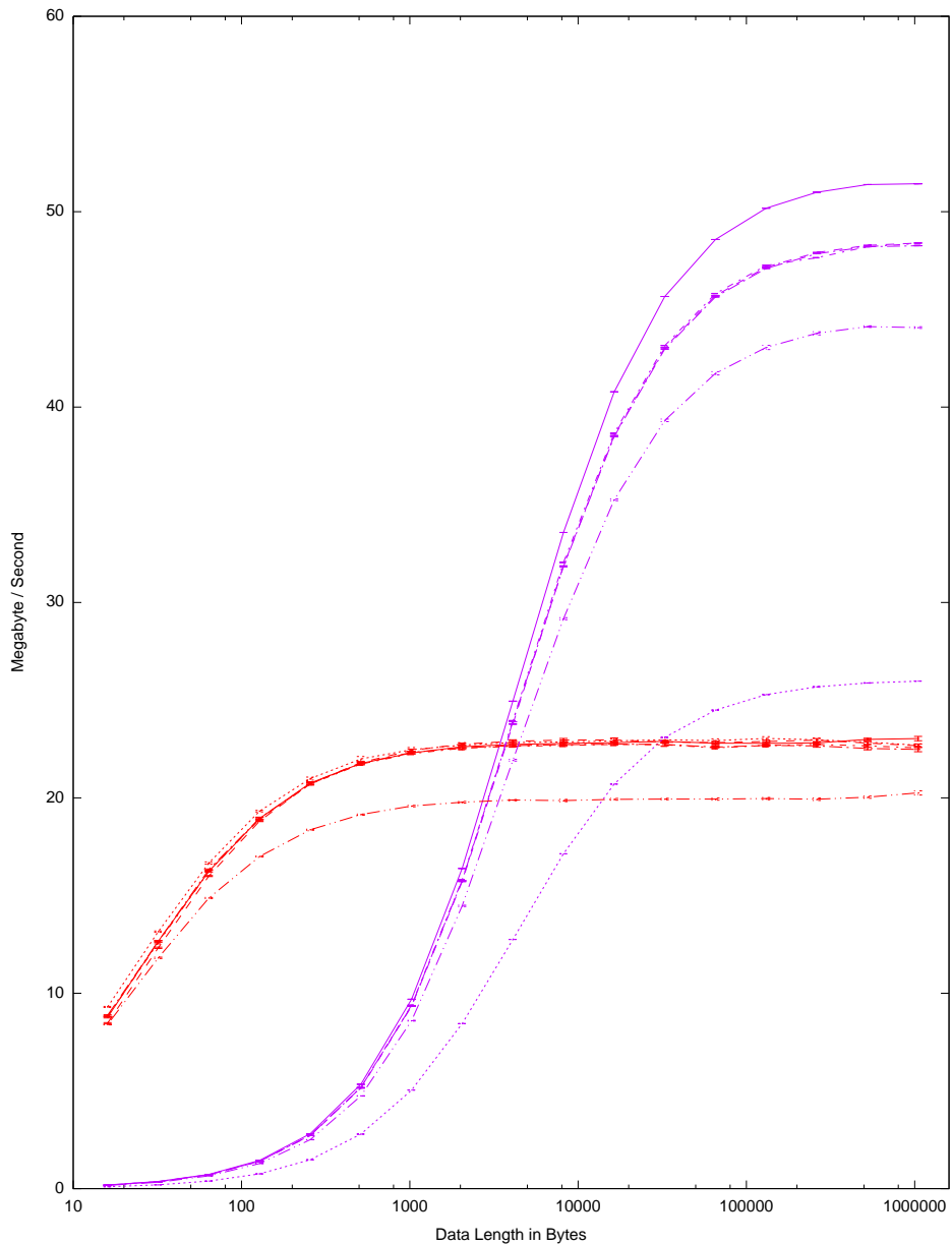
Beecrypt Ciphers: Speed by Data Length
