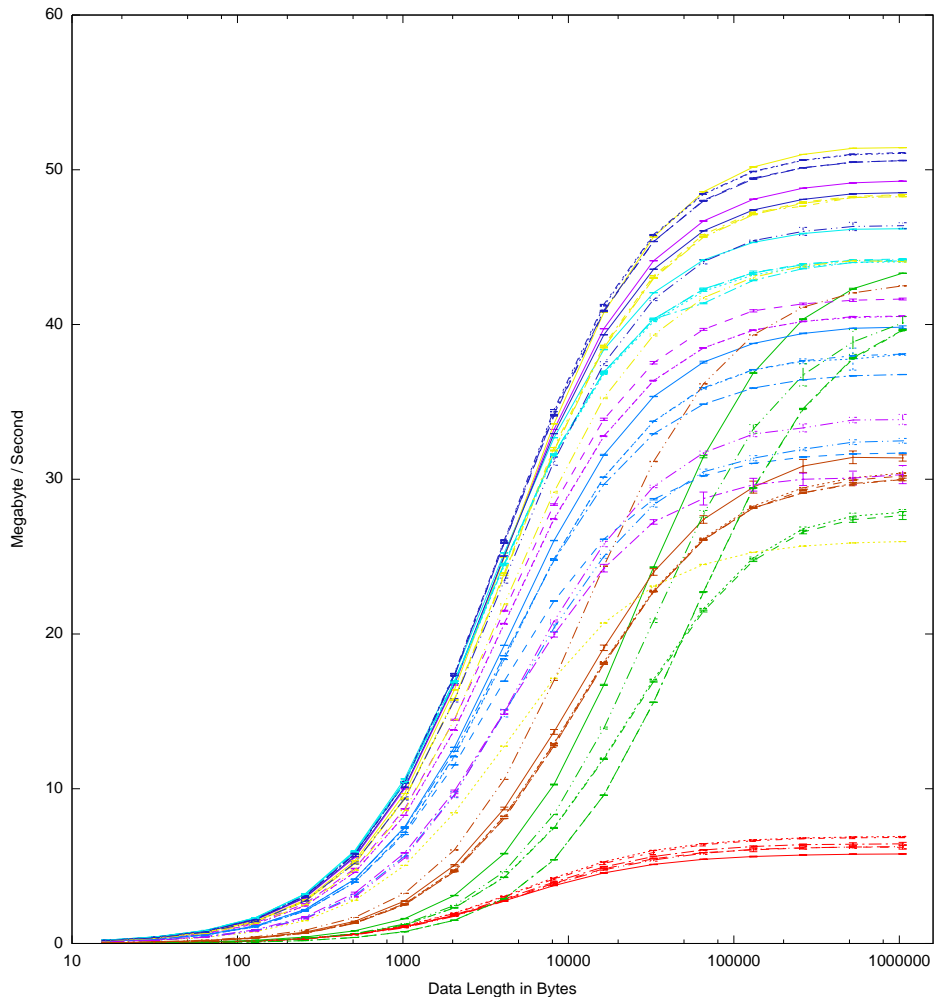
Blowfish: Speed by Data Length
