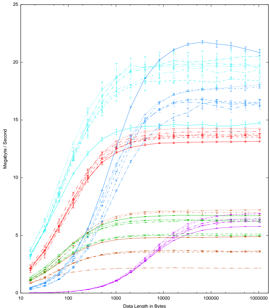
libcrypt Ciphers: Speed by Data Length
