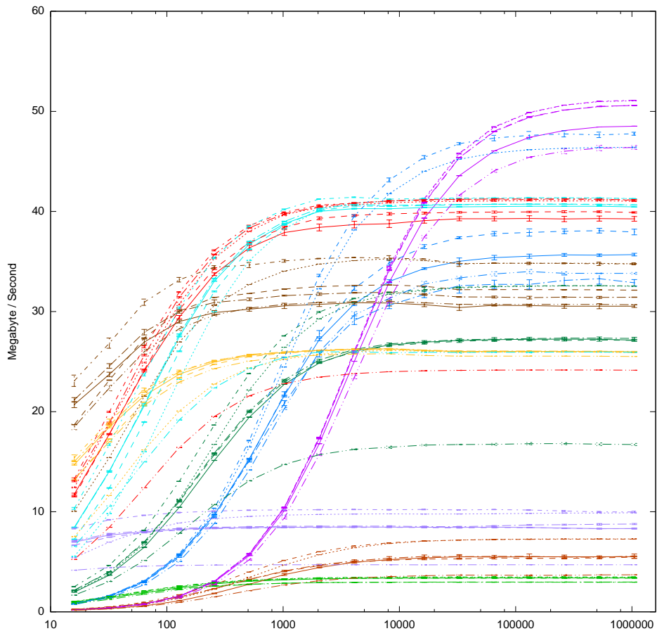
Tomcrypt Ciphers: Speed by Data Length
