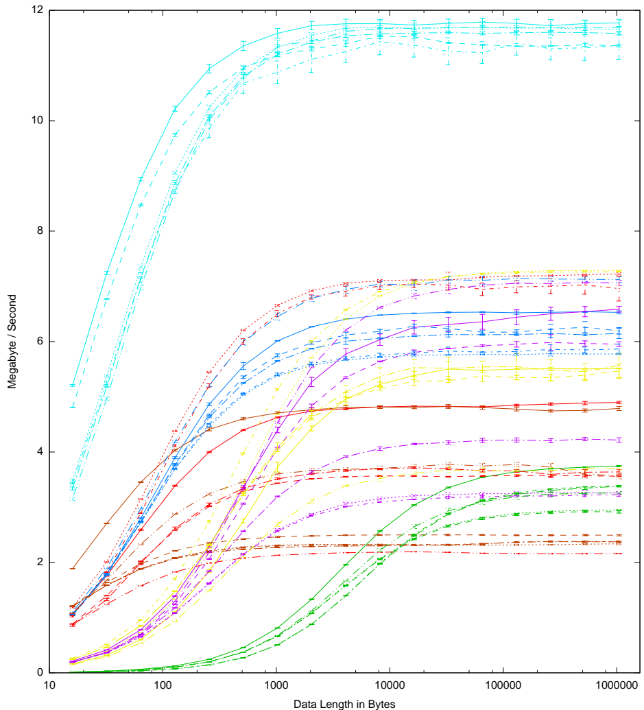
Triple DES: Speed by Data Length
