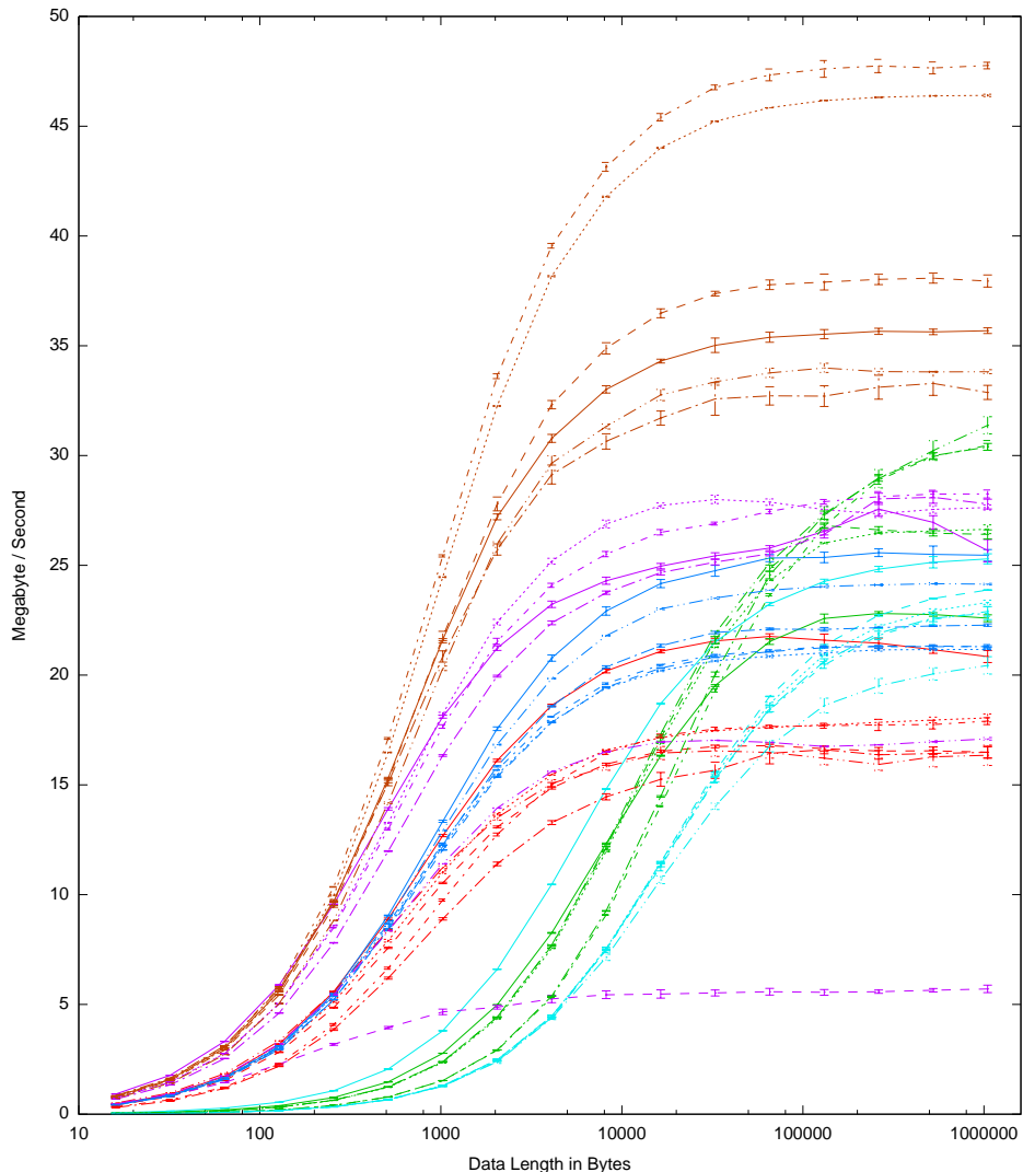
Twofish: Speed by Data Length
