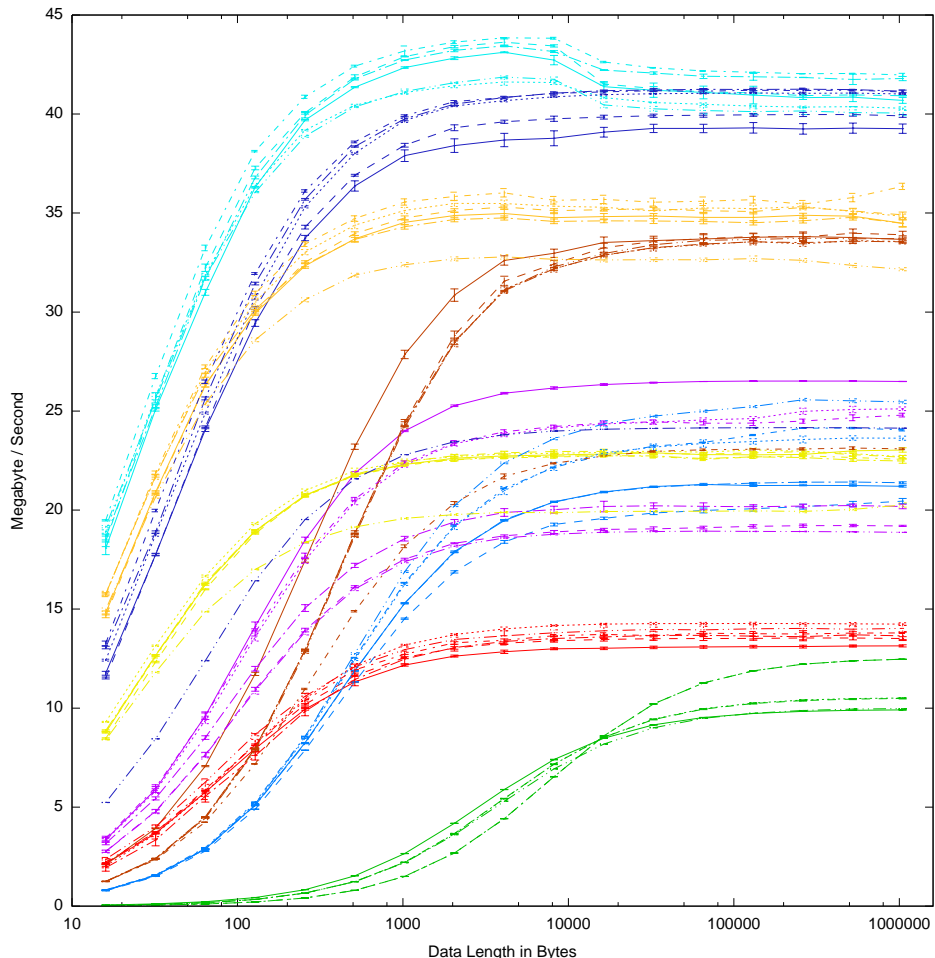
Rijndael AES: Speed by Data Length
