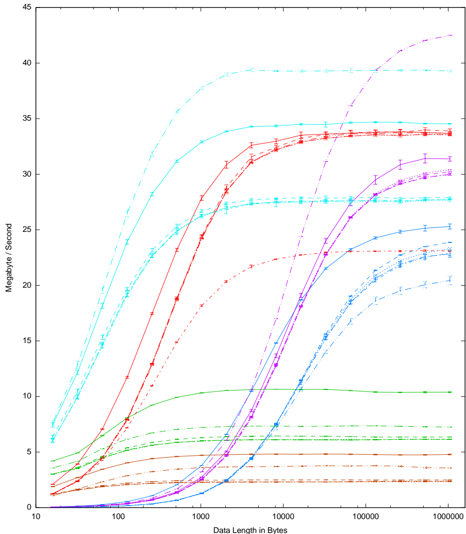
Nettle Ciphers: Speed by Data Length
