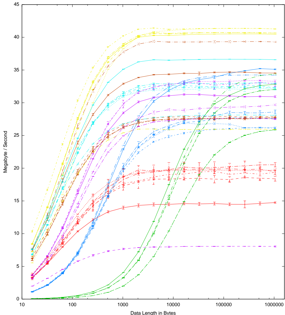
CAST5: Speed by Data Length
