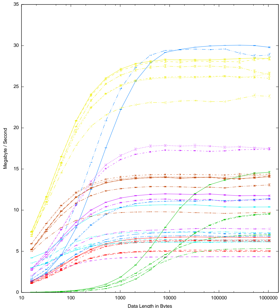
Serpent: Speed by Data Length
