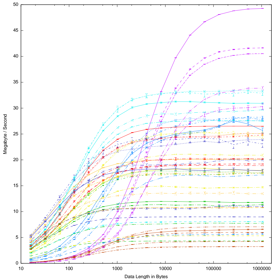
Crypto++ Ciphers: Speed by Data Length
